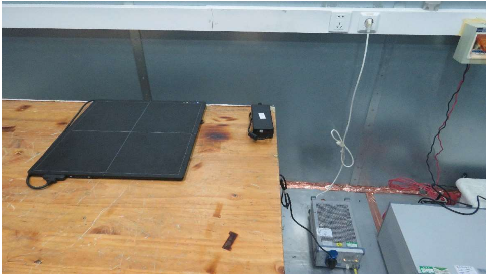
Picture 2 Conducted Emission Test Setup
