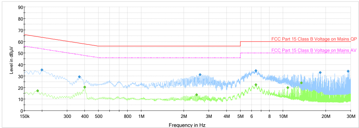
Plot 7-4. Line Conducted Plot (N)
