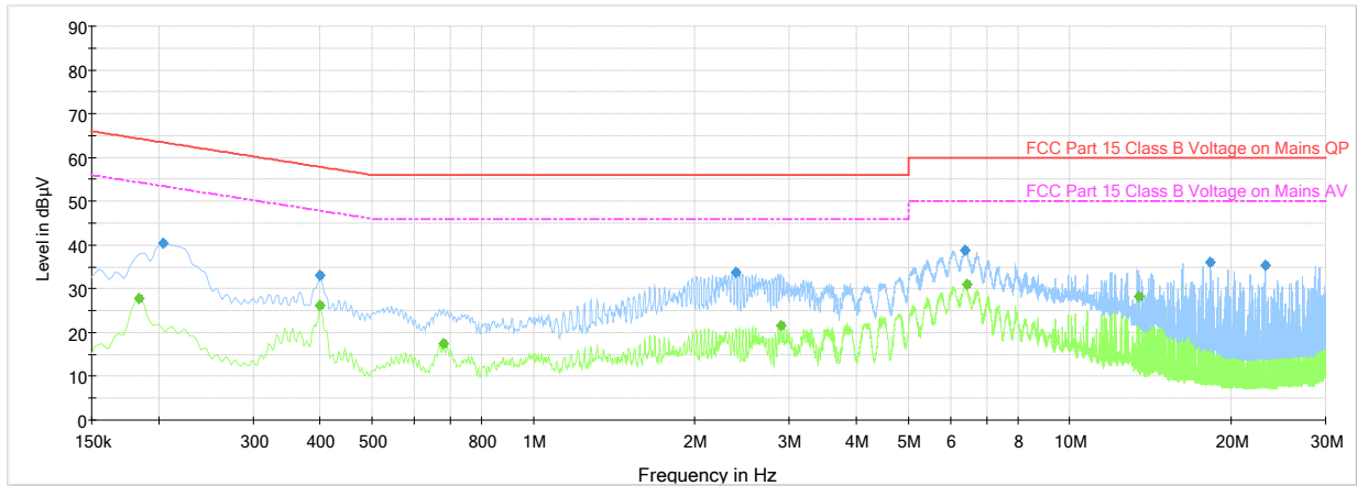
Plot 7-3. Line Conducted Plot (L1)
