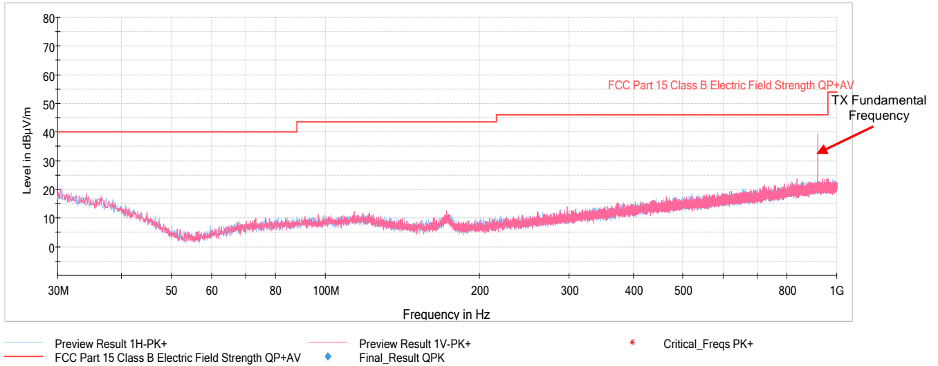
Plot 7-1. Radiated Spurious Plot Below 1GHz
