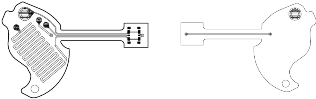
FPC Antenna
