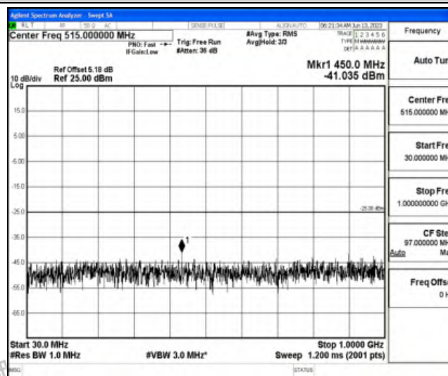
Band38-20MHz-16QAM-38000-1RB#0-Range3:30~1000MHz
