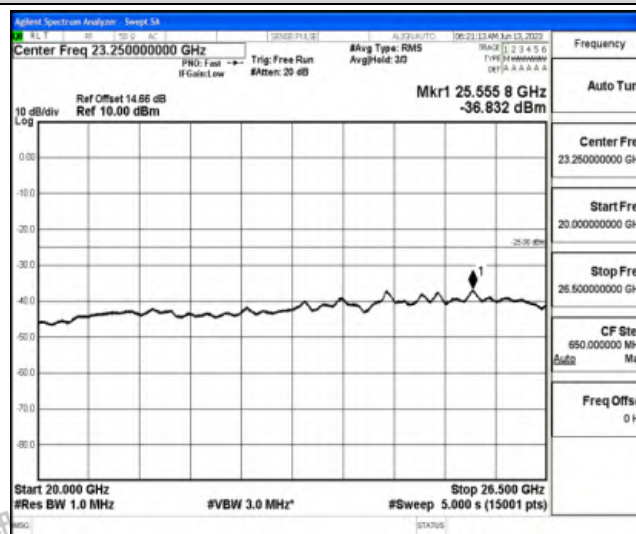
Band38-20MHz-QPSK-38000-1RB#0-Range6:20000~26500MHz
