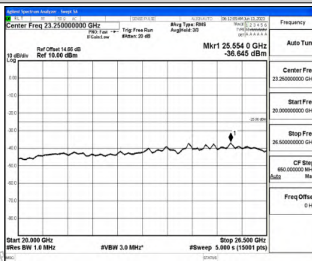
Band38-15MHz-QPSK-38175-1RB#0-Range6:20000~26500MHz
