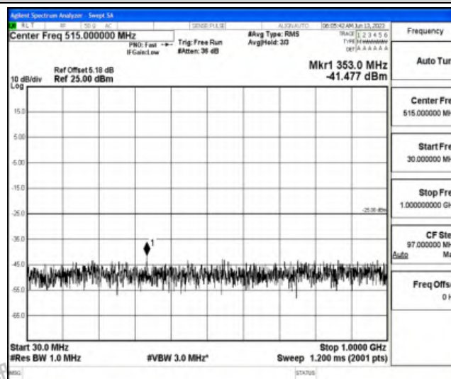
Band38-15MHz-QPSK-37825-1RB#0-Range3:30~1000MHz
