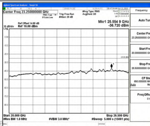
Band38-5MHz-16QAM-38000-1RB#0-Range6:20000~26500MHz
