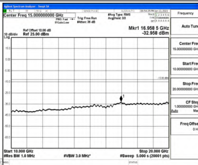
Band25-10MHz-QPSK-26640-1RB#0-Range5:10000~20000MHz
