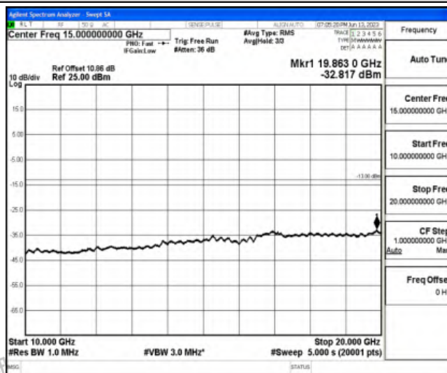
Band25-15MHz-16QAM-26615-1RB#0-Range5:10000~20000MHz
