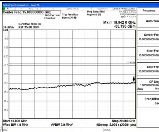
Band25-10MHz-16QAM-26640-1RB#0-Range5:10000~20000MHz
