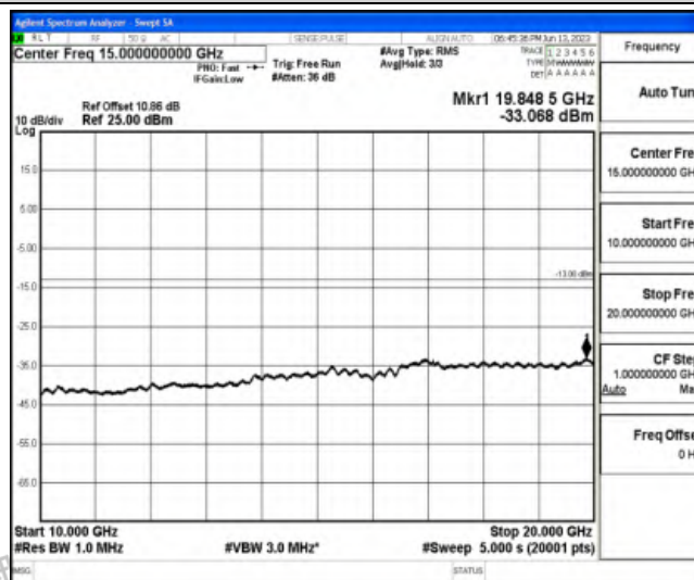
Band25-5MHz-16QAM-26665-1RB#0-Range5:10000~20000MHz
