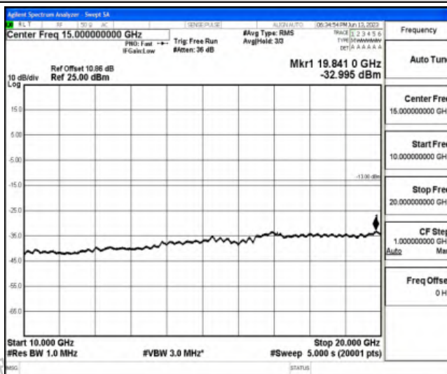
Band25-3MHz-16QAM-26675-1RB#0-Range5:10000~20000MHz
