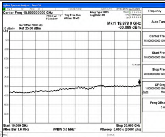
Band25-15MHz-QPSK-26615-1RB#0-Range5:10000~20000MHz
