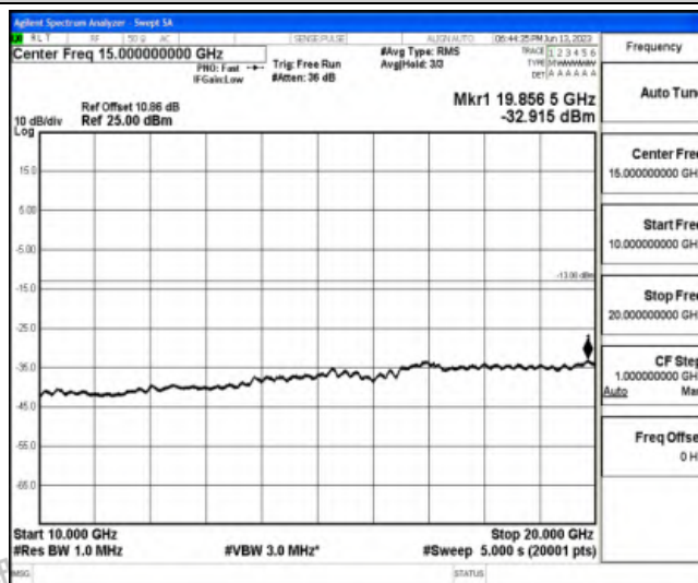
Band25-5MHz-QPSK-26665-1RB#0-Range5:10000~20000MHz
