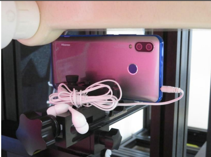
Photo 25: Bottom Side with Headset 5mm
