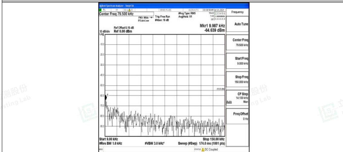
Band7_15MHz_16QAM_21100_1RB#0_0.009~0.15_0.009~0.15
