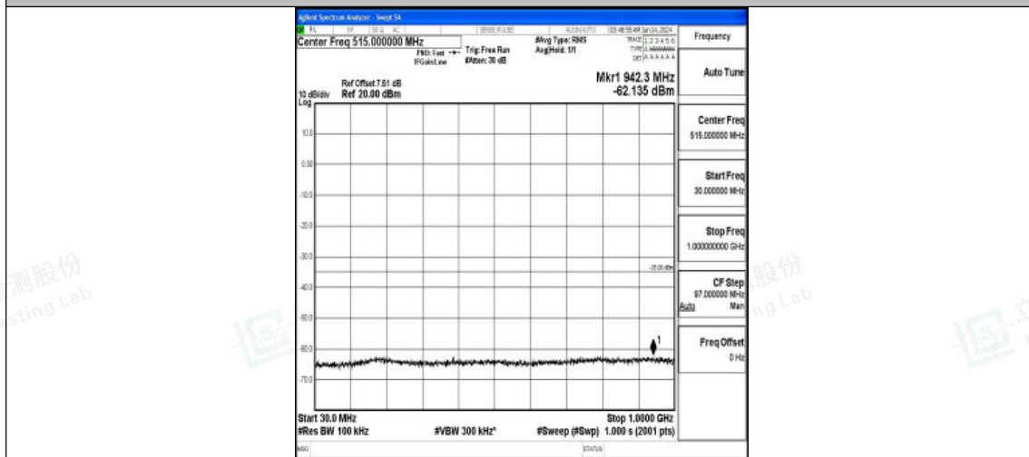
Band7_20MHz_QPSK_21100_1RB#0_30~1000_30~1000
