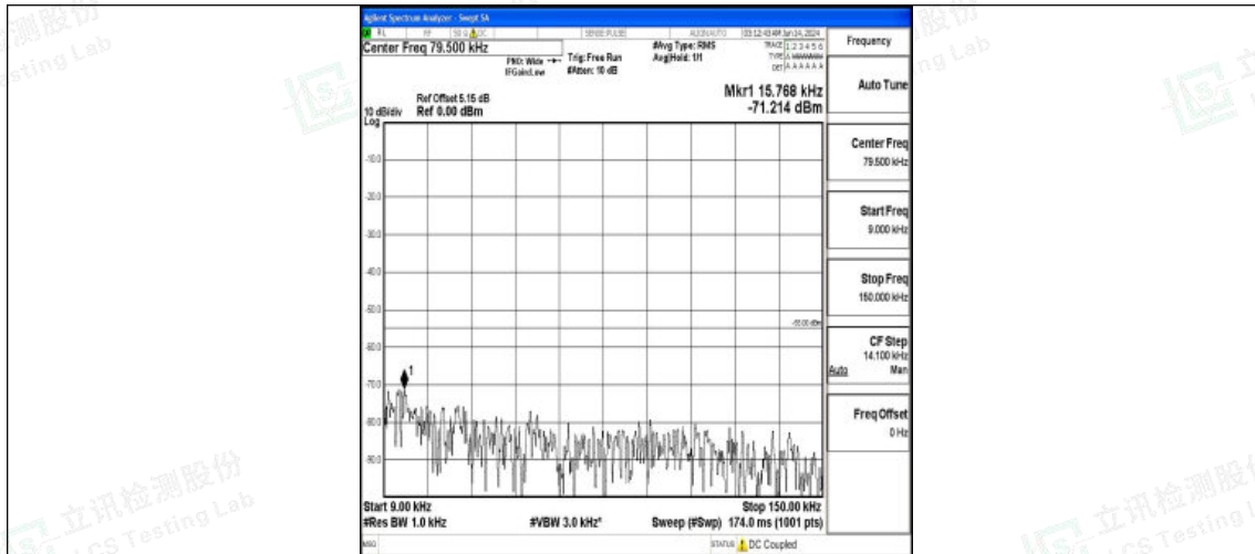
Band7_10MHz_QPSK_21400_1RB#0_0.009~0.15_0.009~0.15
