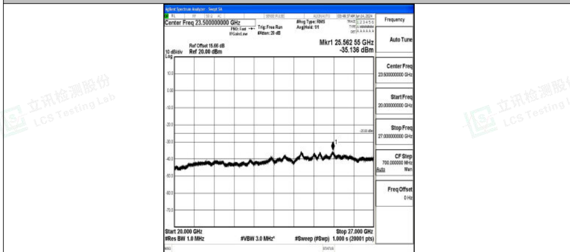
Band7_20MHz_16QAM_21100_1RB#0_20000~27000_20000~27000
