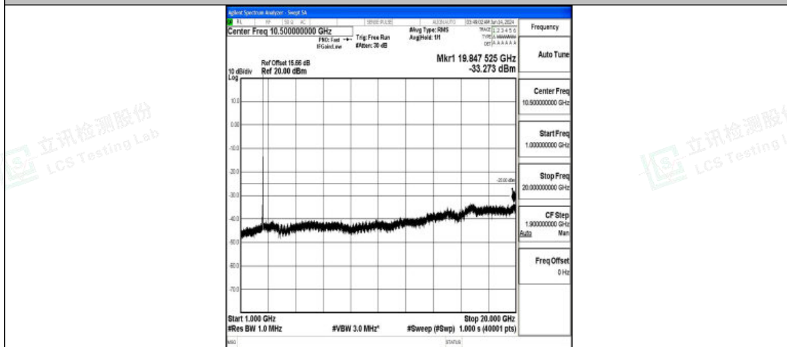
Band7_20MHz_QPSK_21100_1RB#0_1000~20000_1000~20000
