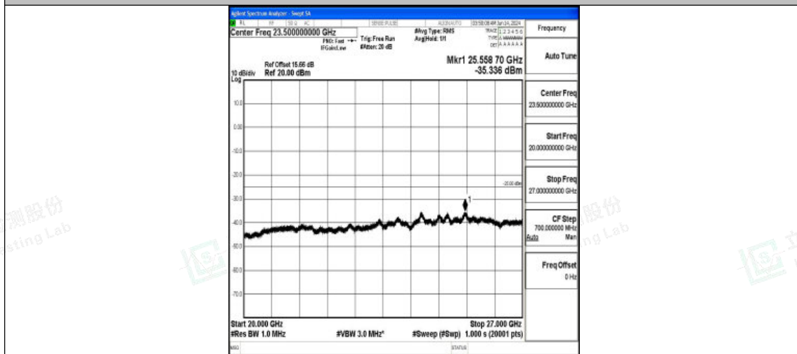
Band7_20MHz_QPSK_21350_1RB#0_20000~27000_20000~27000
