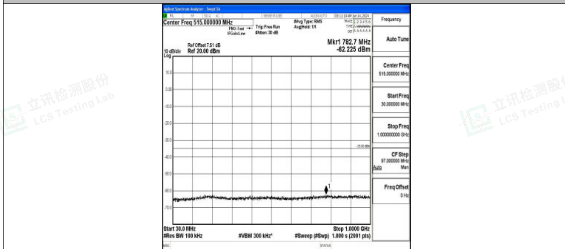
Band7_10MHz_16QAM_20800_1RB#0_30~1000_30~1000
