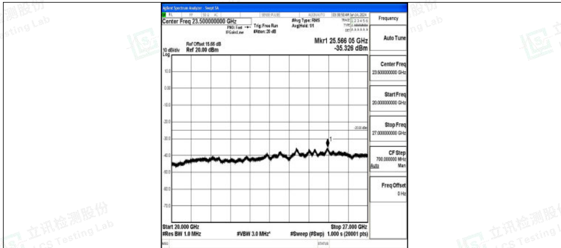
Band7_15MHz_QPSK_21100_1RB#0_20000~27000_20000~27000
