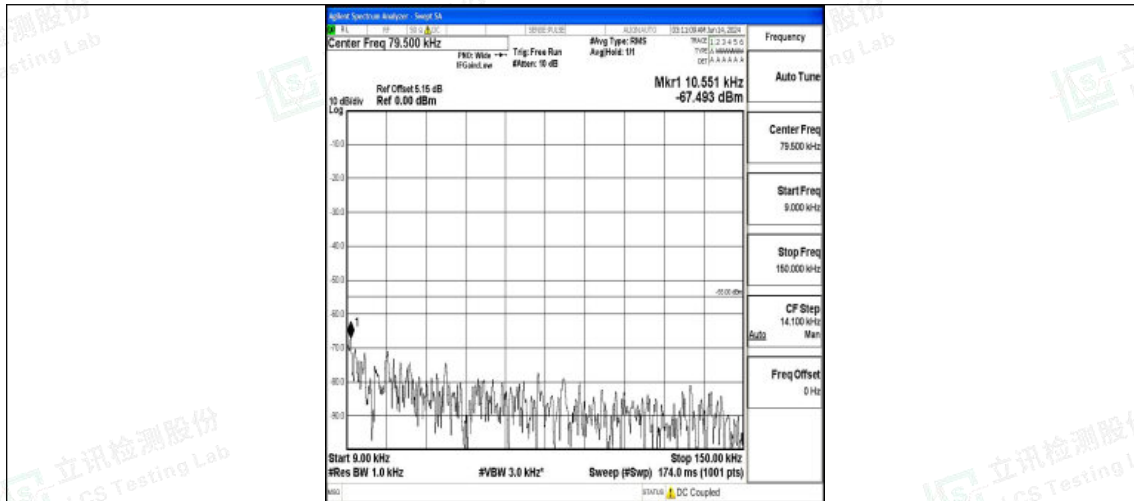
Band7_10MHz_16QAM_20800_1RB#0_0.009~0.15_0.009~0.15
