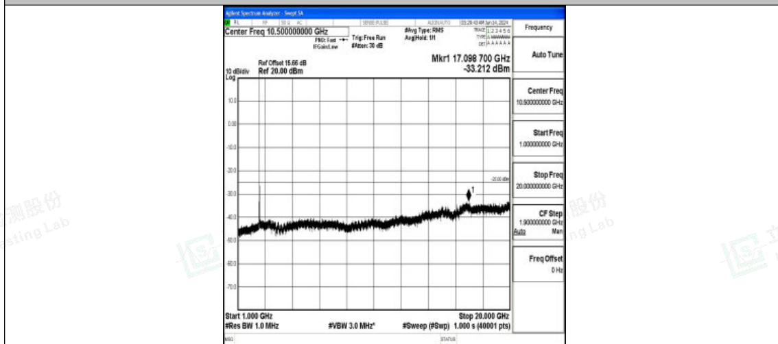
Band7_15MHz_QPSK_20825_1RB#0_1000~20000_1000~20000
