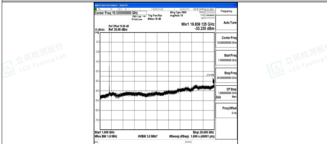
Band7_15MHz_16QAM_21375_1RB#0_1000~20000_1000~20000
