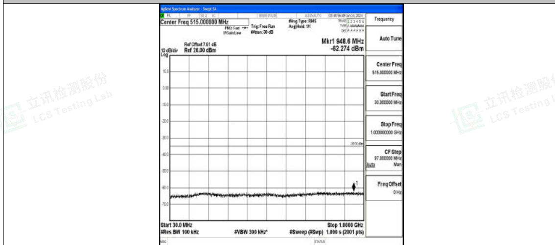
Band7_20MHz_QPSK_21350_1RB#0_30~1000_30~1000
