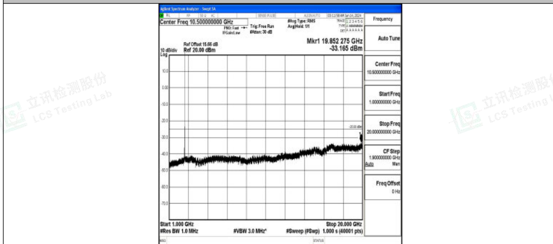
Band7_10MHz_QPSK_21100_1RB#0_1000~20000_1000~20000
