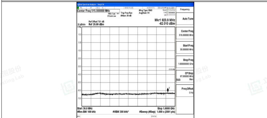
Band7_10MHz_QPSK_21100_1RB#0_30~1000_30~1000
