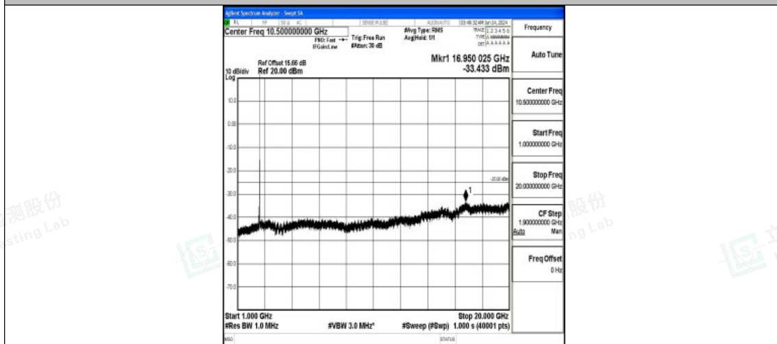
Band7_20MHz_16QAM_21100_1RB#0_1000~20000_1000~20000
