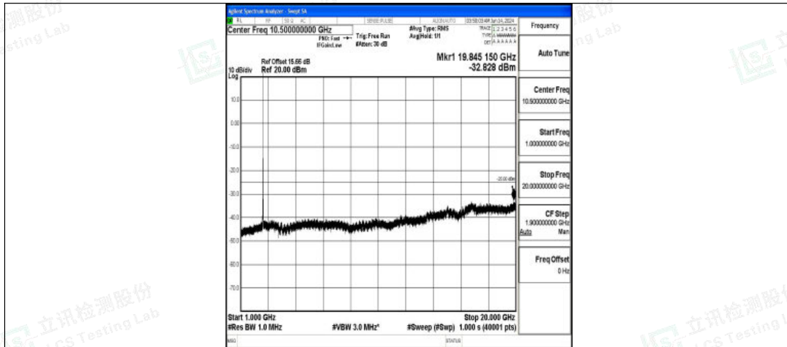
Band7_20MHz_QPSK_21350_1RB#0_1000~20000_1000~20000
