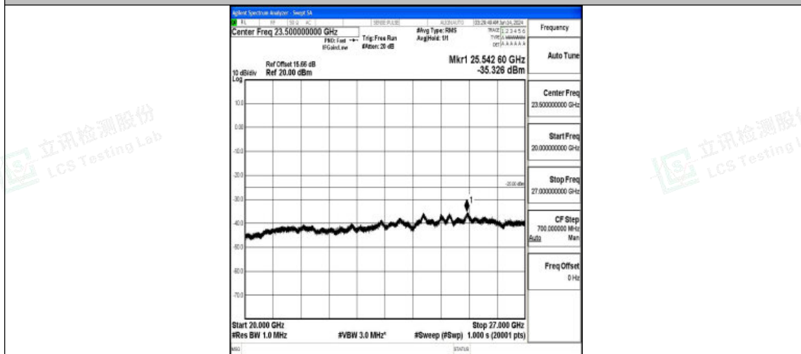
Band7_15MHz_QPSK_20825_1RB#0_20000~27000_20000~27000
