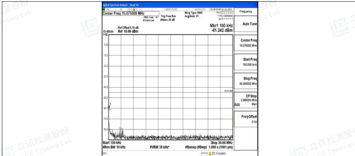
Band7_20MHz_QPSK_21100_1RB#0_0.15~30_0.15~30
