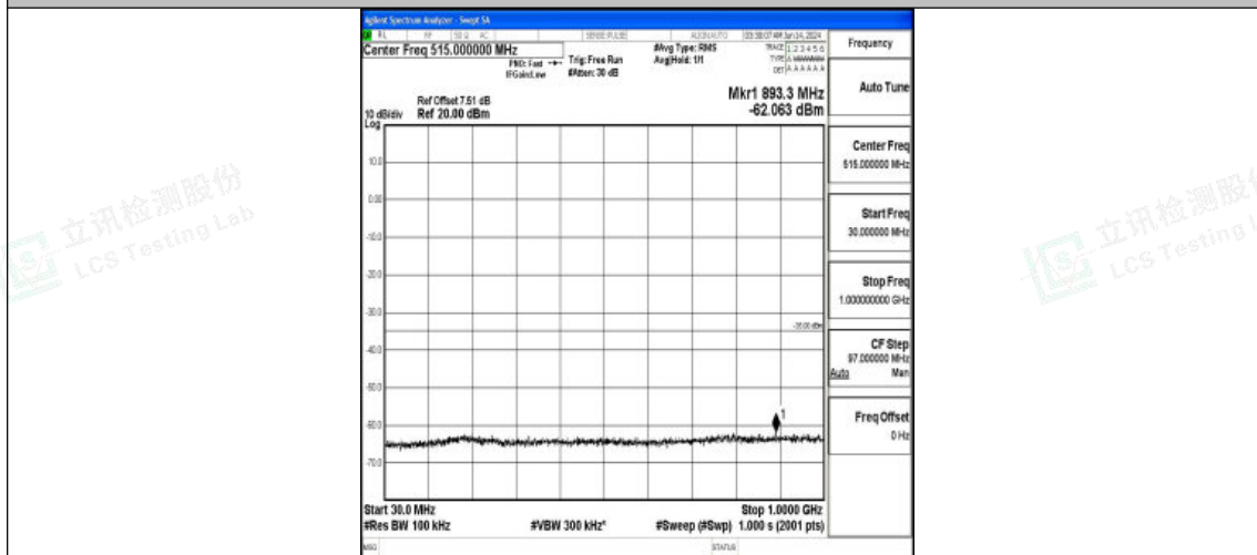
Band7_15MHz_16QAM_20825_1RB#0_30~1000_30~1000
