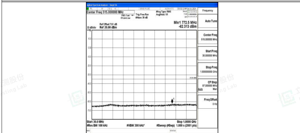
Band7_15MHz_16QAM_21375_1RB#0_30~1000_30~1000
