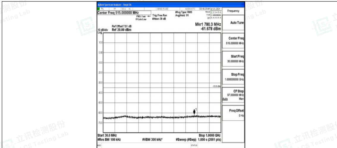
Band7_20MHz_16QAM_21100_1RB#0_30~1000_30~1000
