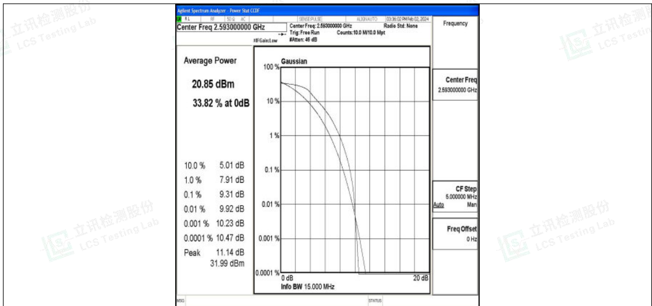
Band41-15MHz-QPSK-40620-75RB#0-PASS
