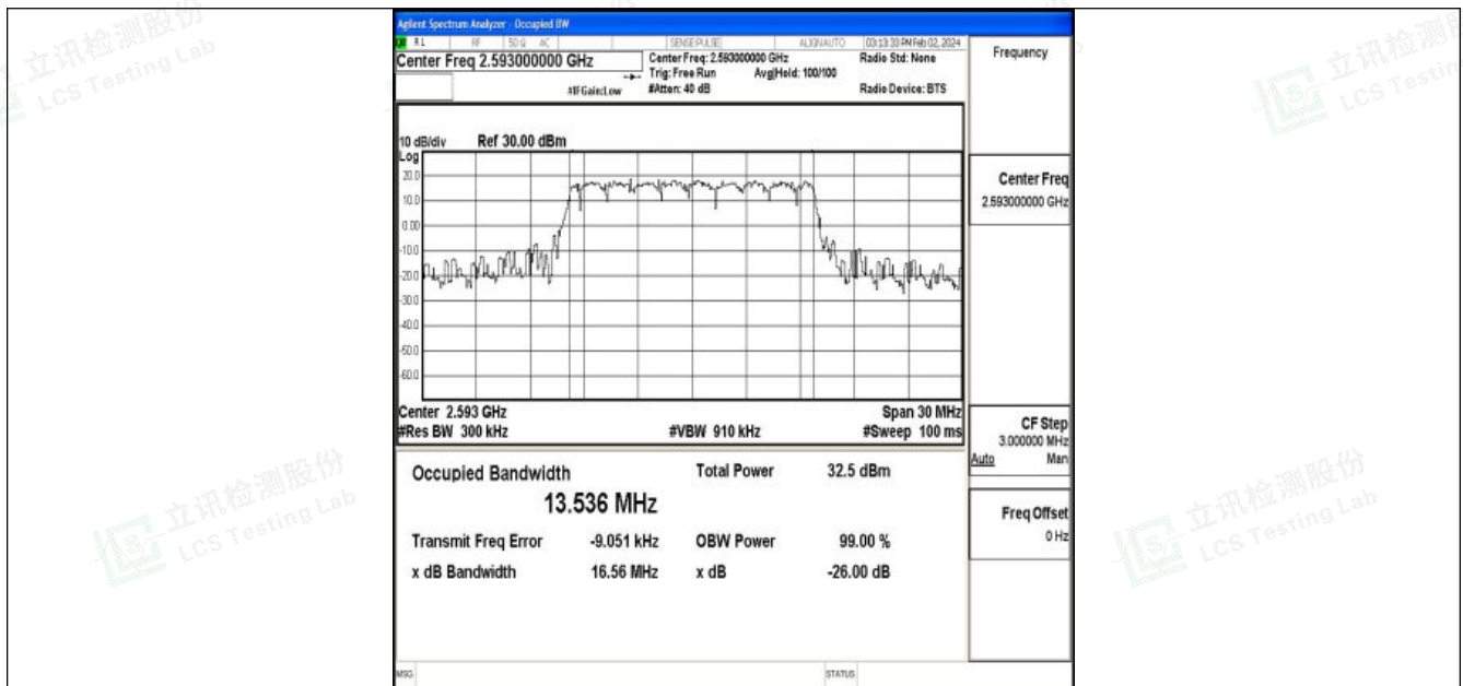
Band41-15MHz-QPSK-40620-75RB#0-PASS
