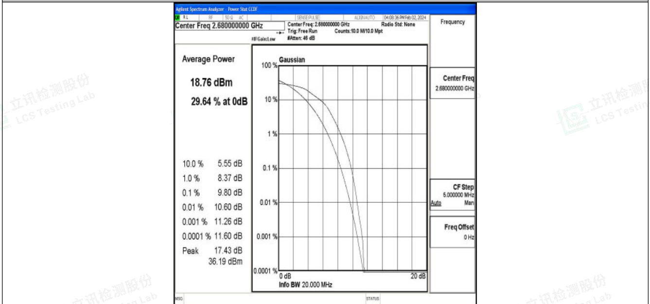
Band41-20MHz-16QAM-41490-100RB#0-PASS
