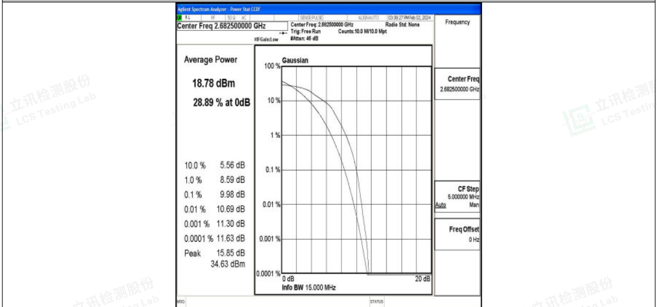
Band41-15MHz-16QAM-41515-75RB#0-PASS
