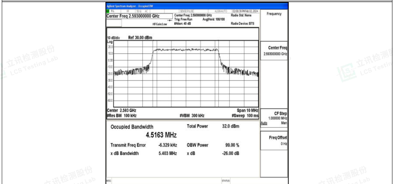
Band41-5MHz-16QAM-40620-25RB#0-PASS
