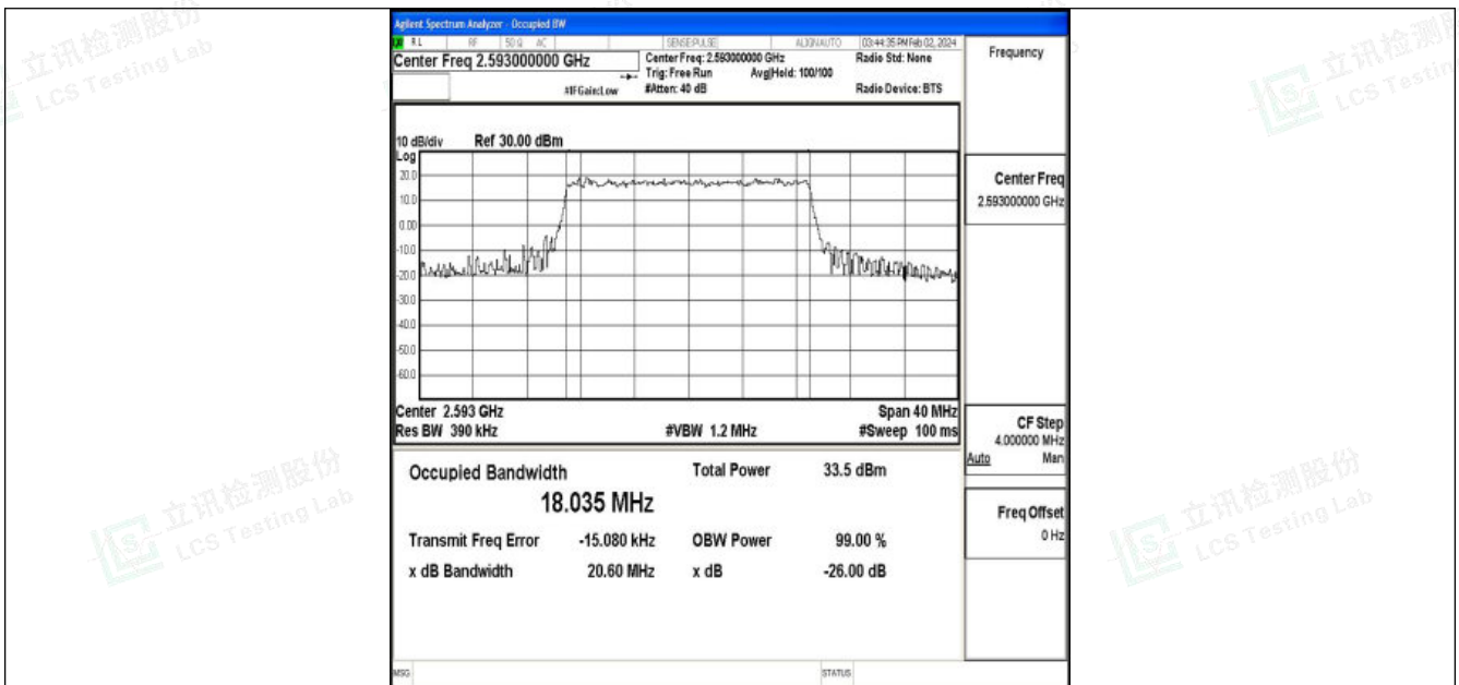
Band41-20MHz-QPSK-40620-100RB#0-PASS
