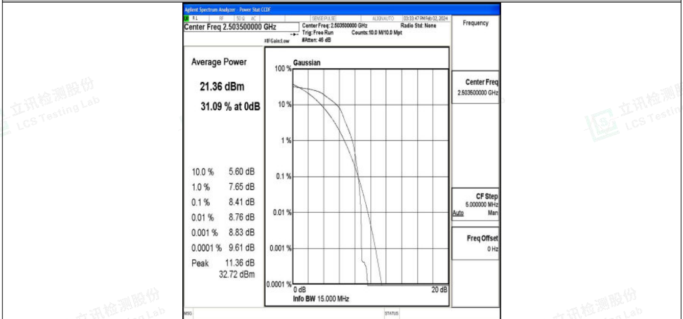
Band41-15MHz-16QAM-39725-1RB#0-PASS
