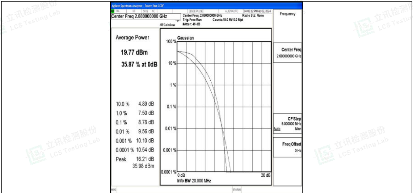
Band41-20MHz-QPSK-41490-100RB#0-PASS
