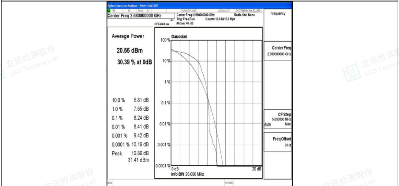
Band41-20MHz-16QAM-41490-1RB#0-PASS
