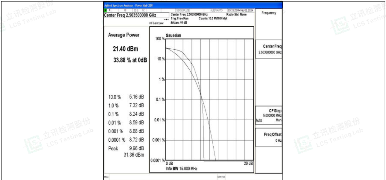
Band41-15MHz-QPSK-39725-1RB#0-PASS
