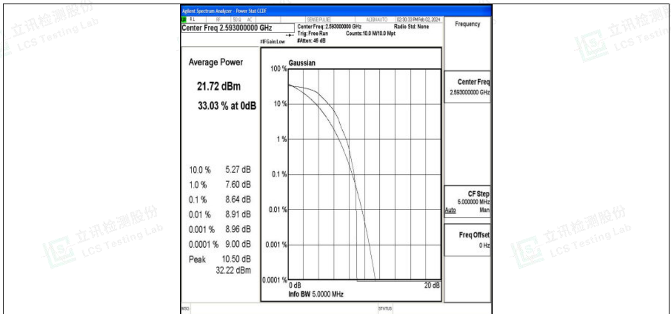
Band41-5MHz-QPSK-40620-1RB#0-PASS
