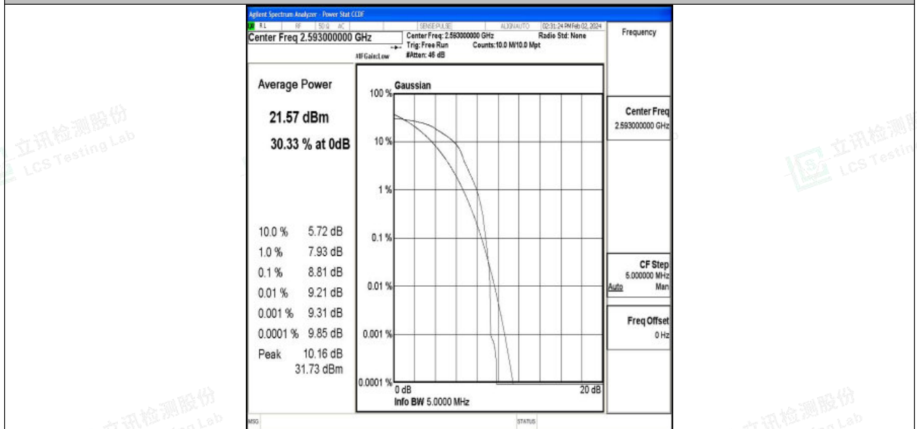
Band41-5MHz-16QAM-40620-1RB#0-PASS
