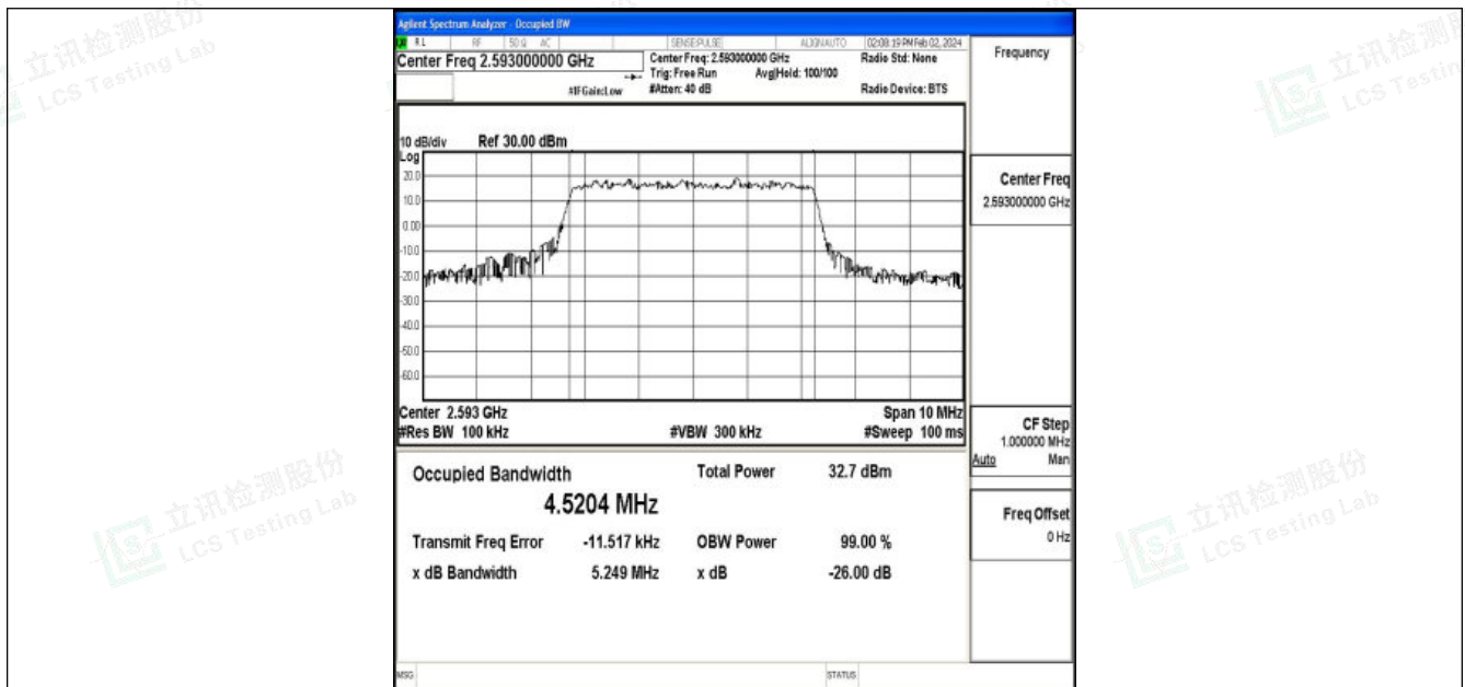
Band41-5MHz-QPSK-40620-25RB#0-PASS
