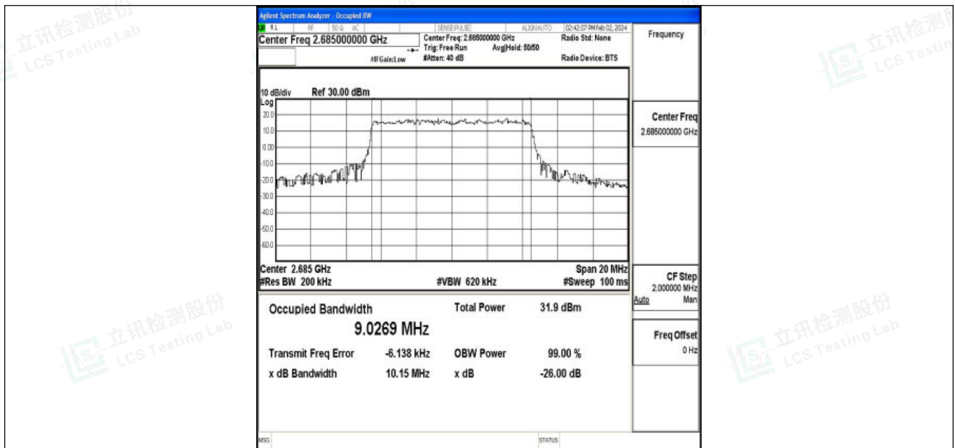
Band41-10MHz-QPSK-41540-50RB#0-PASS
