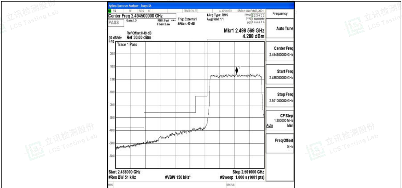
Band41_5MHz_16QAM_39675_25RB#0
