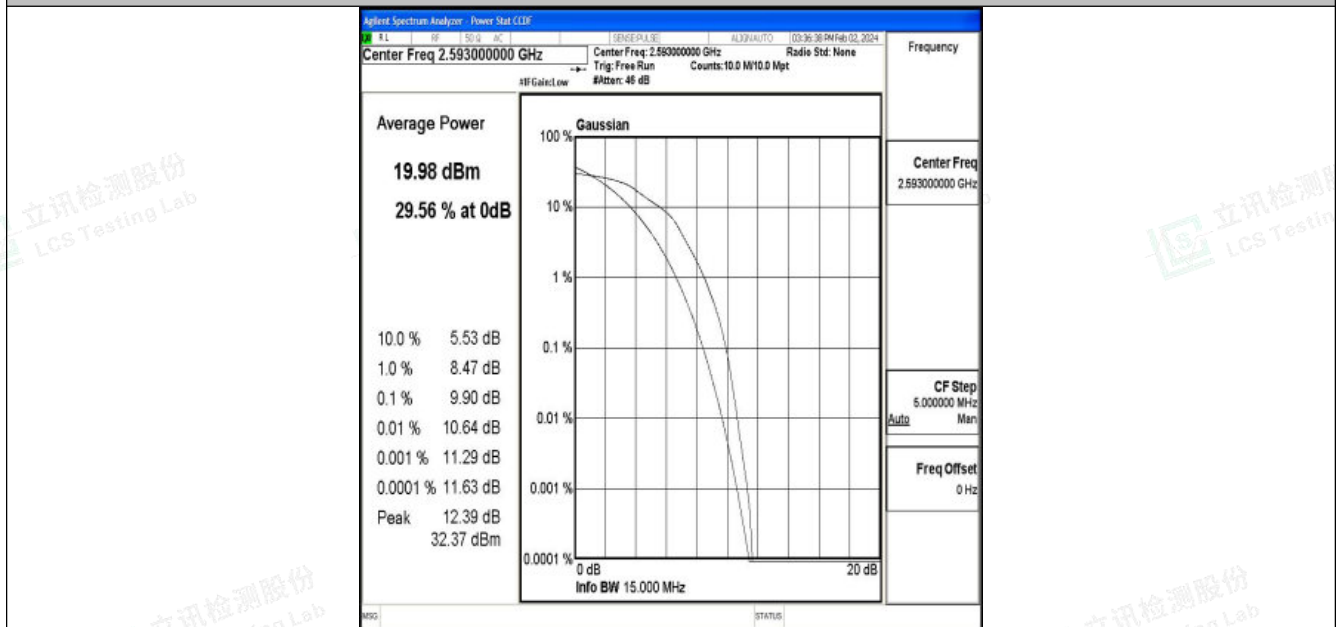
Band41-15MHz-16QAM-40620-75RB#0-PASS
