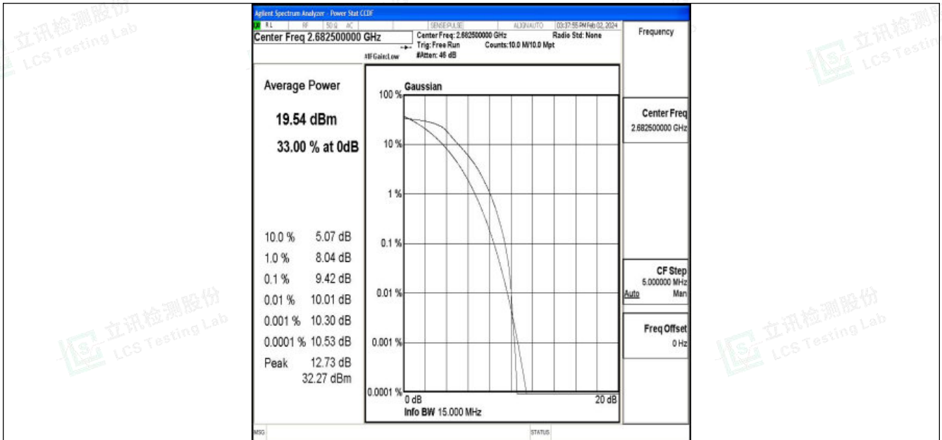
Band41-15MHz-QPSK-41515-75RB#0-PASS
