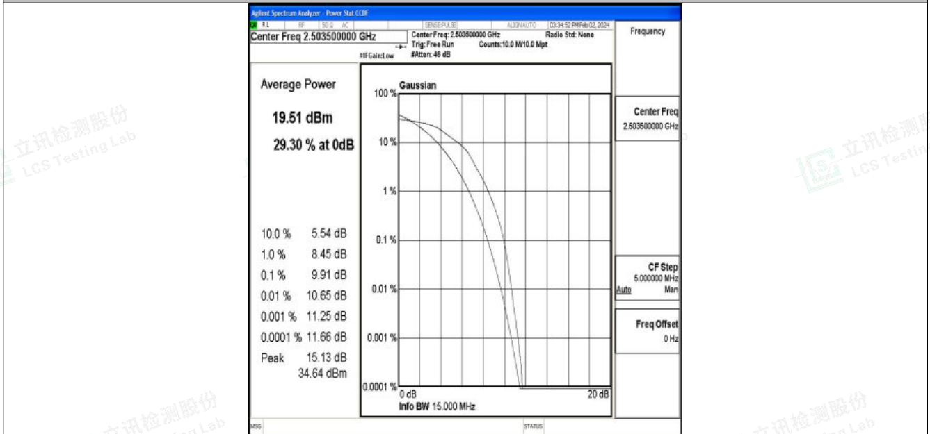
Band41-15MHz-16QAM-39725-75RB#0-PASS
