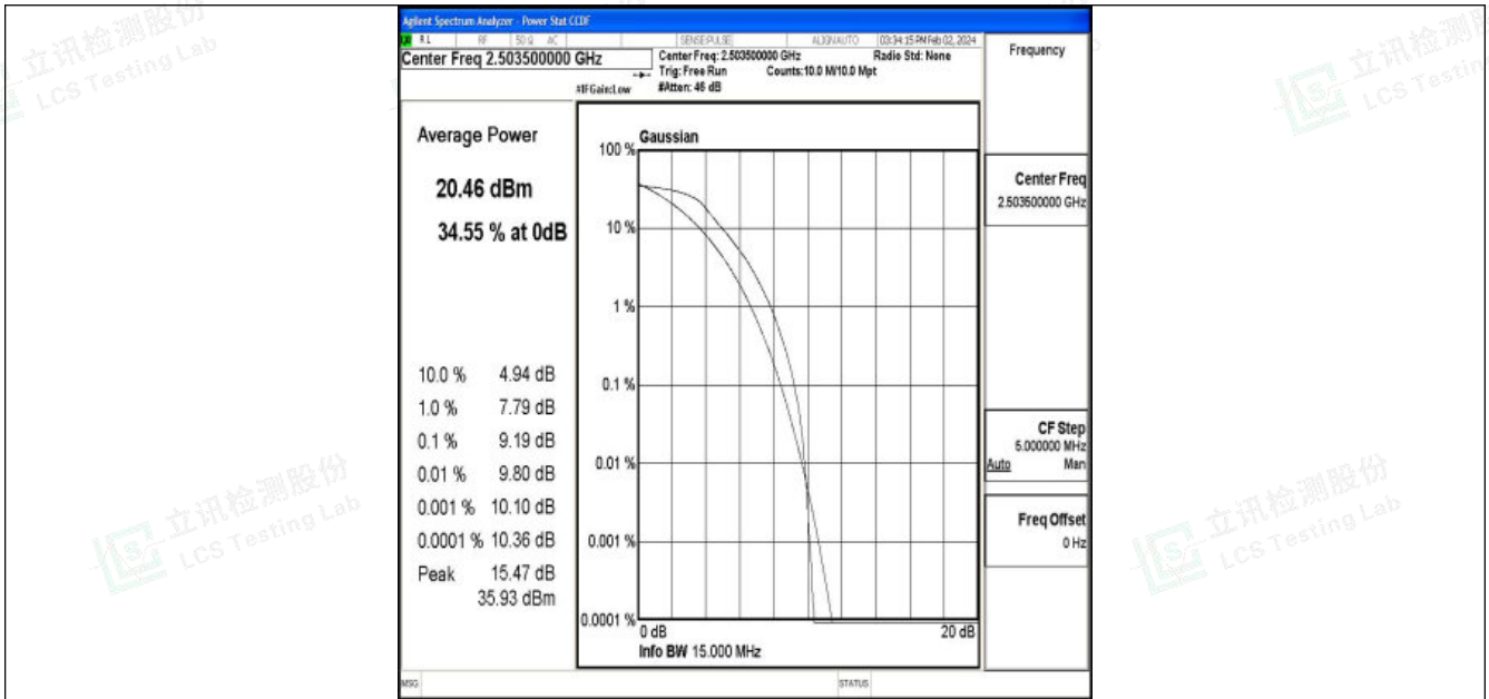
Band41-15MHz-QPSK-39725-75RB#0-PASS
