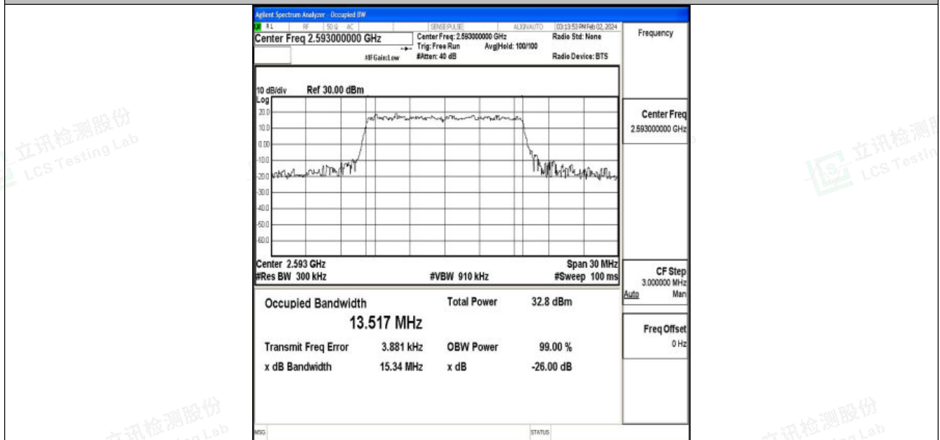
Band41-15MHz-16QAM-40620-75RB#0-PASS
