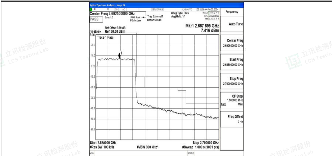
Band41_5MHz_QPSK_41565_25RB#0
