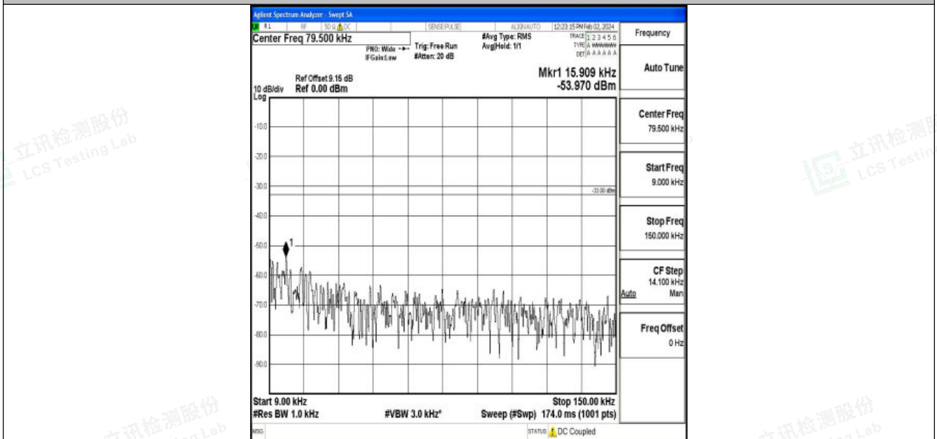
Band26_10MHz_16QAM_26990_1RB#0_0.009~0.15_0.009~0.15
