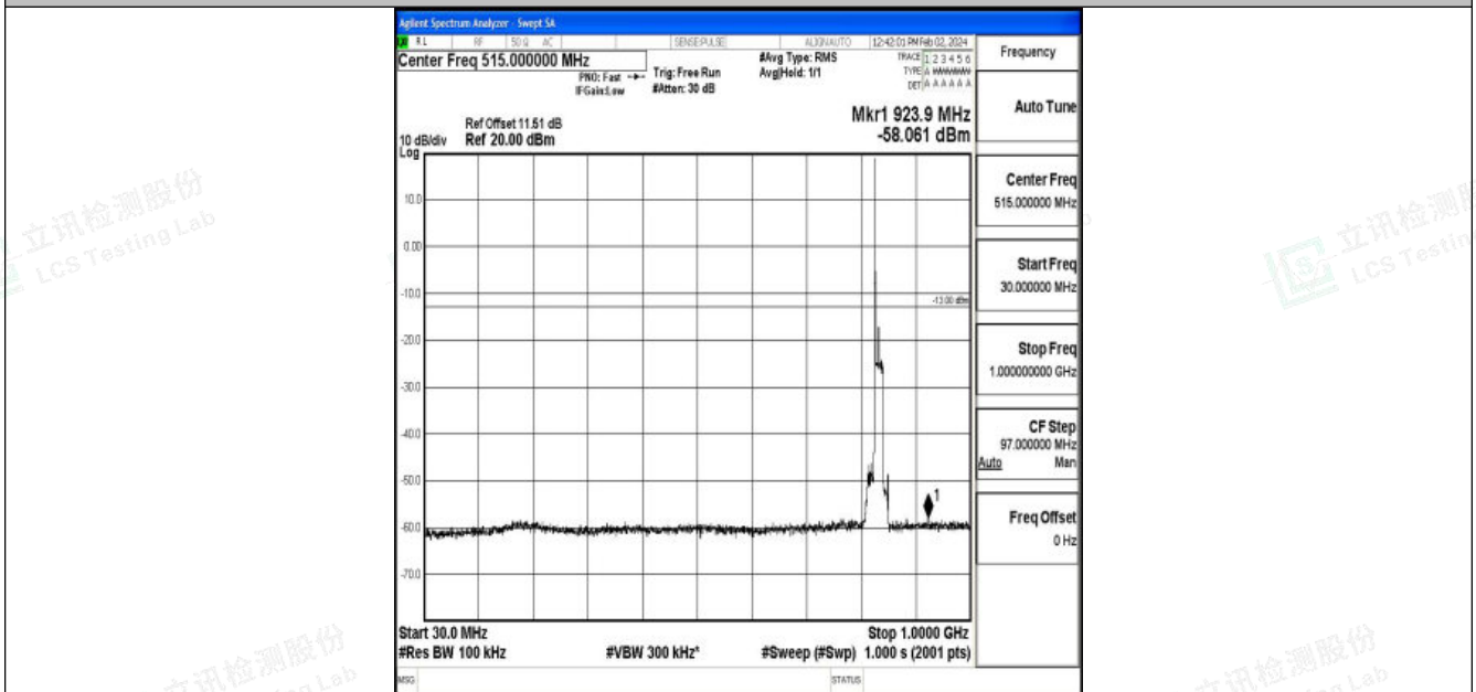
Band26_15MHz_16QAM_26915_1RB#0_30~1000_30~1000
