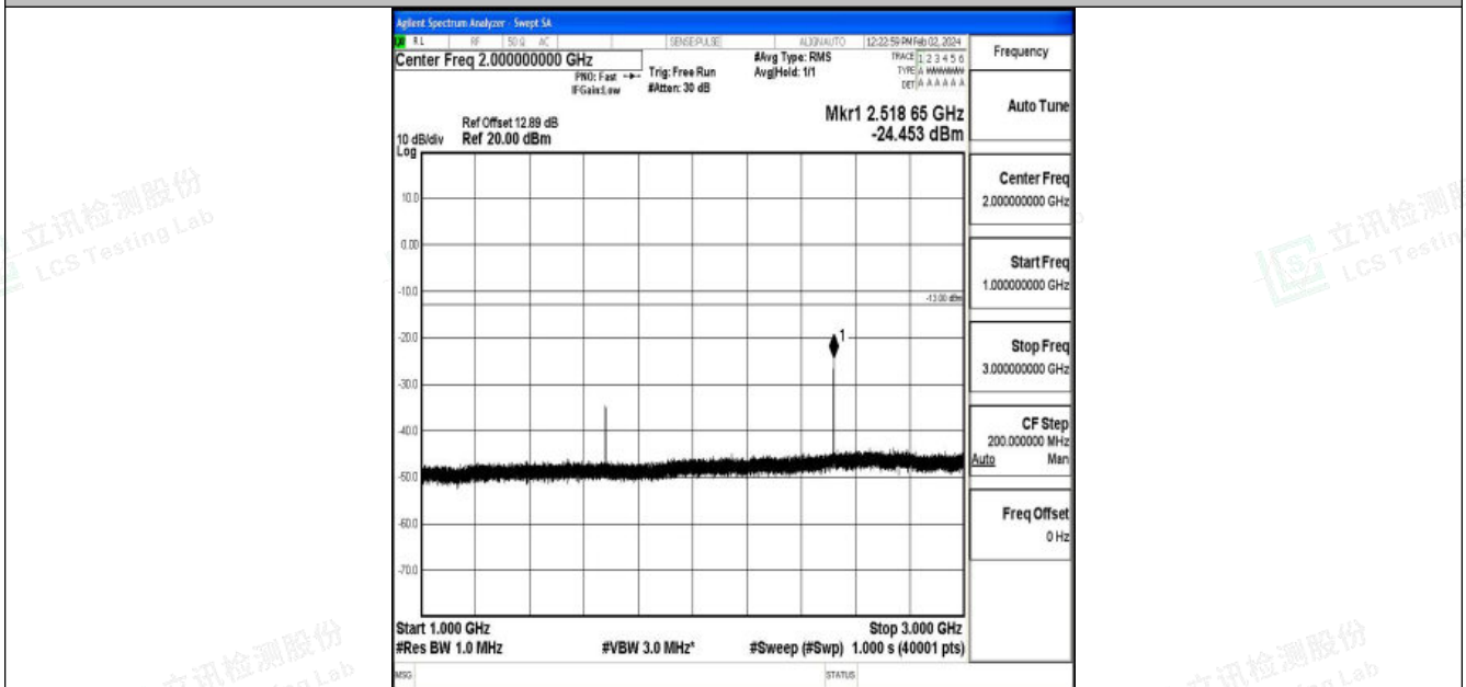
Band26_10MHz_QPSK_26990_1RB#0_1000~3000_1000~3000
