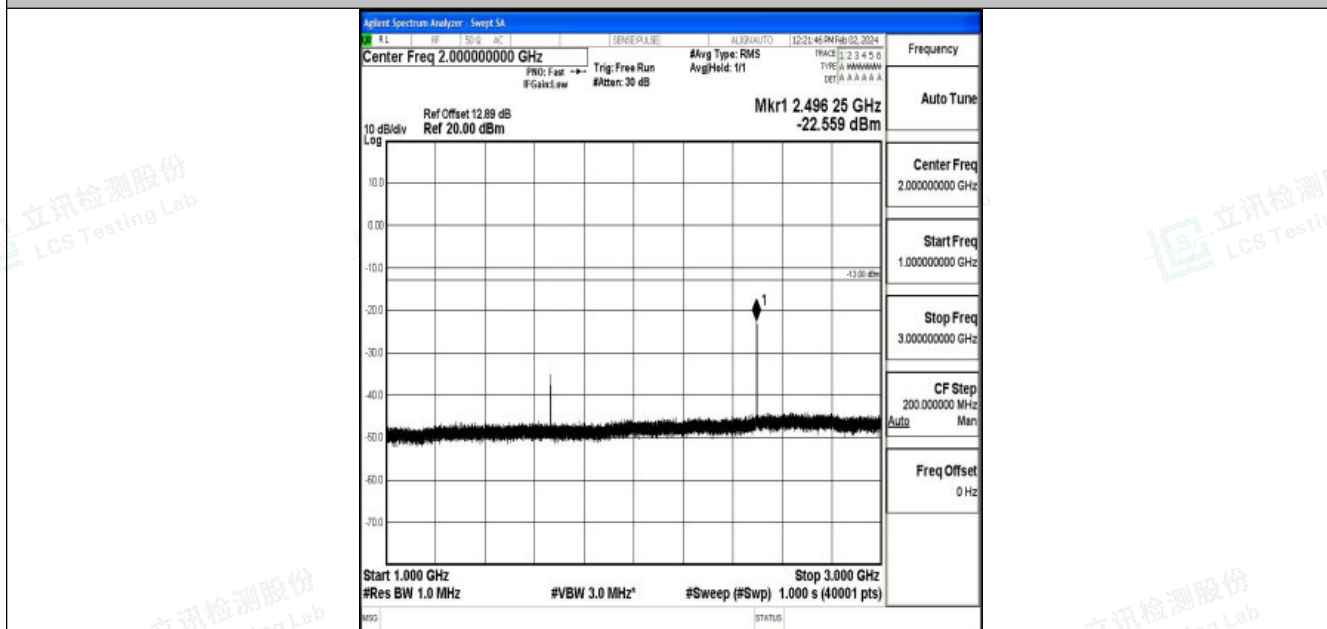
Band26_10MHz_QPSK_26915_1RB#0_1000~3000_1000~3000
