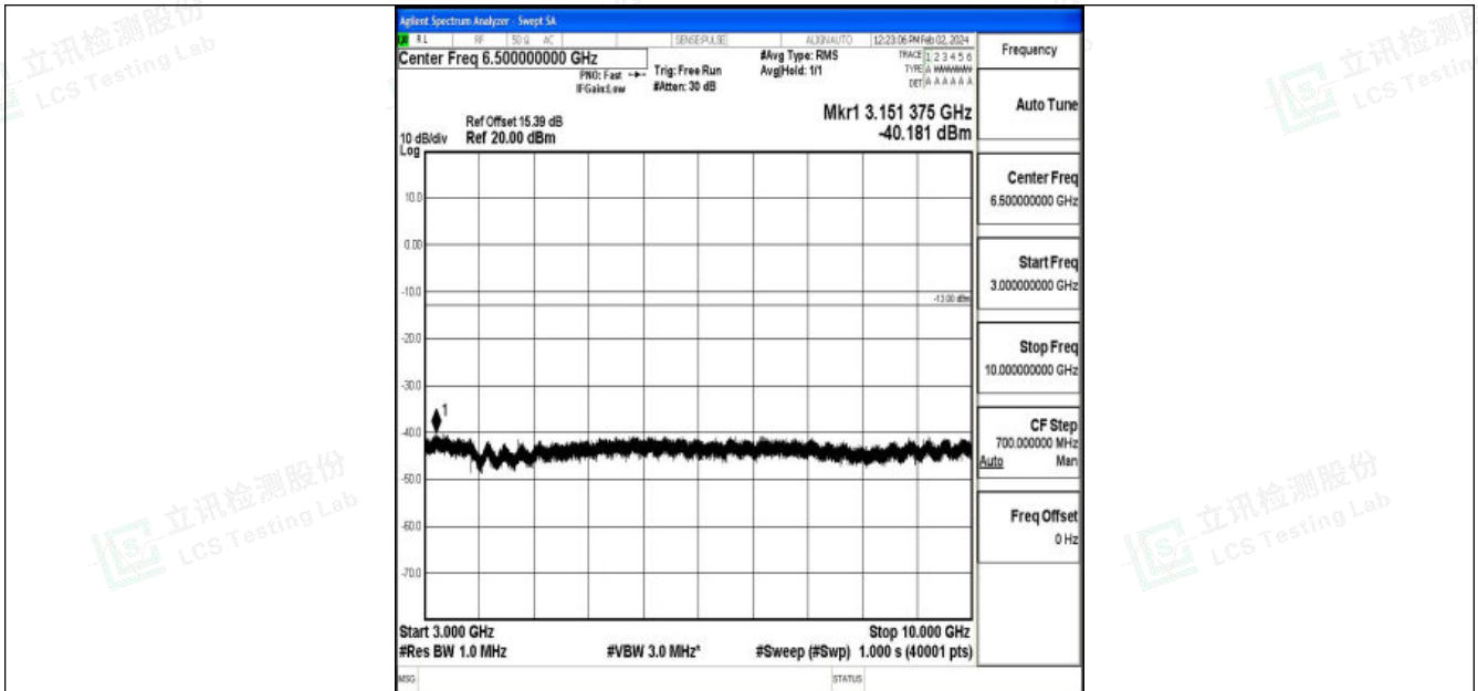
Band26_10MHz_QPSK_26990_1RB#0_3000~10000_3000~10000
