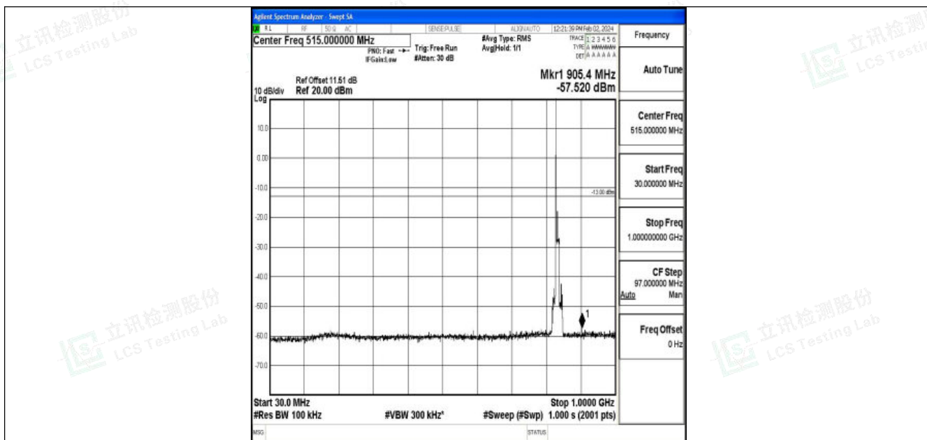
Band26_10MHz_QPSK_26915_1RB#0_30~1000_30~1000
