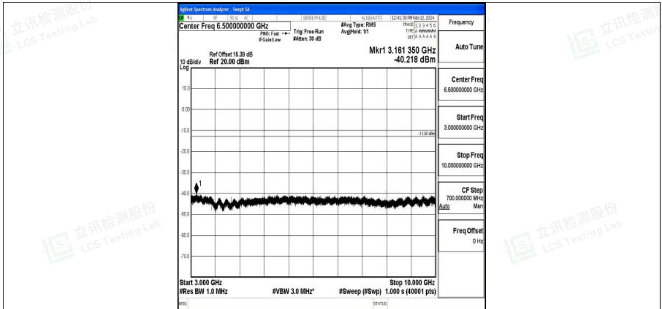
Band26_15MHz_QPSK_26915_1RB#0_3000~10000_3000~10000
