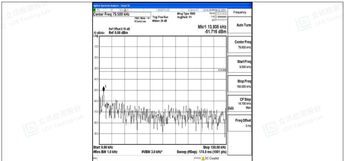
Band26_15MHz_QPSK_26915_1RB#0_0.009~0.15_0.009~0.15
