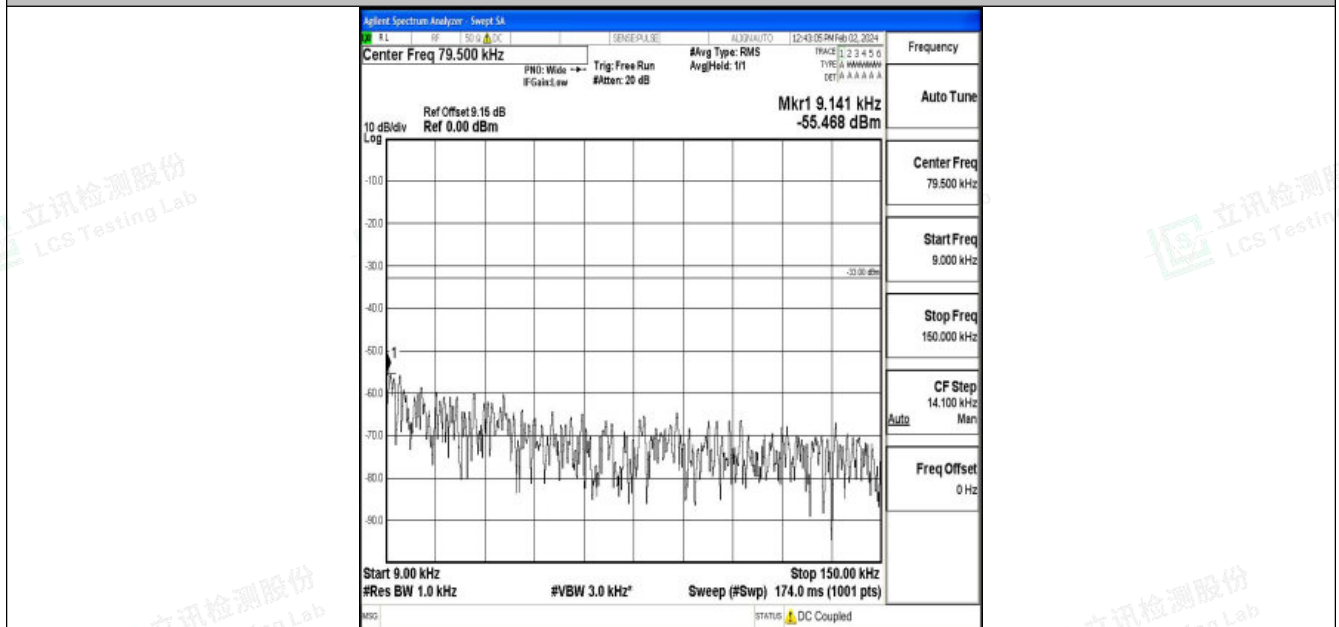
Band26_15MHz_16QAM_26965_1RB#0_0.009~0.15_0.009~0.15
