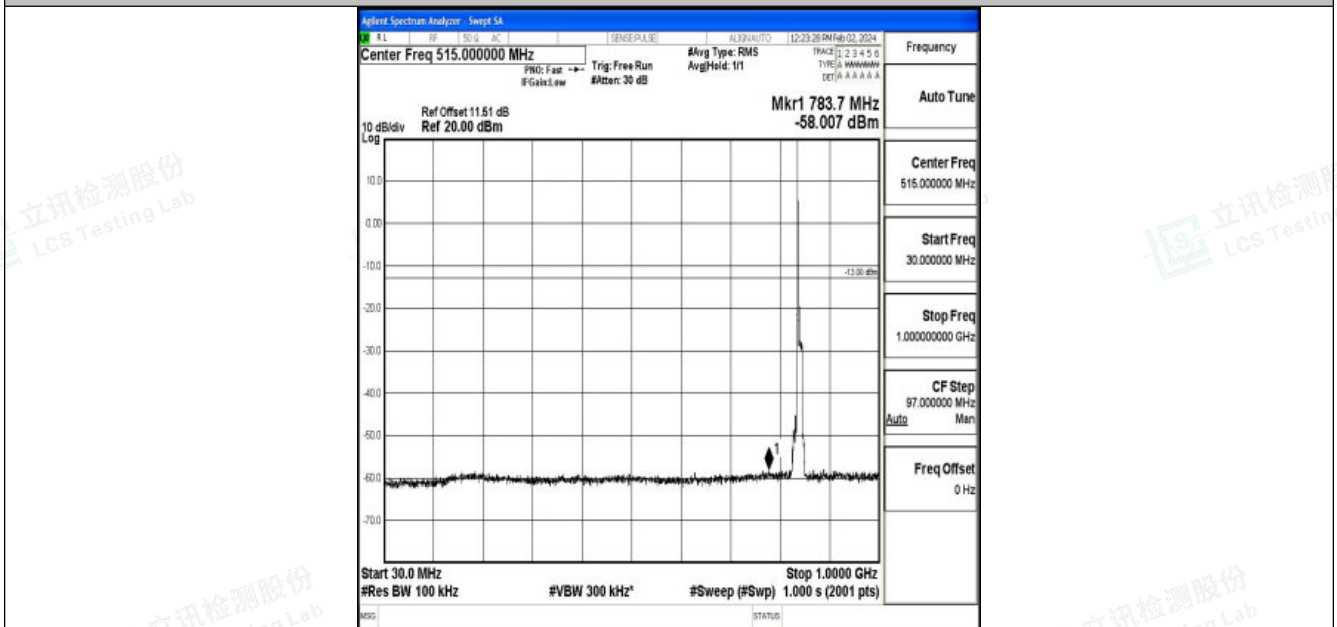
Band26_10MHz_16QAM_26990_1RB#0_30~1000_30~1000
