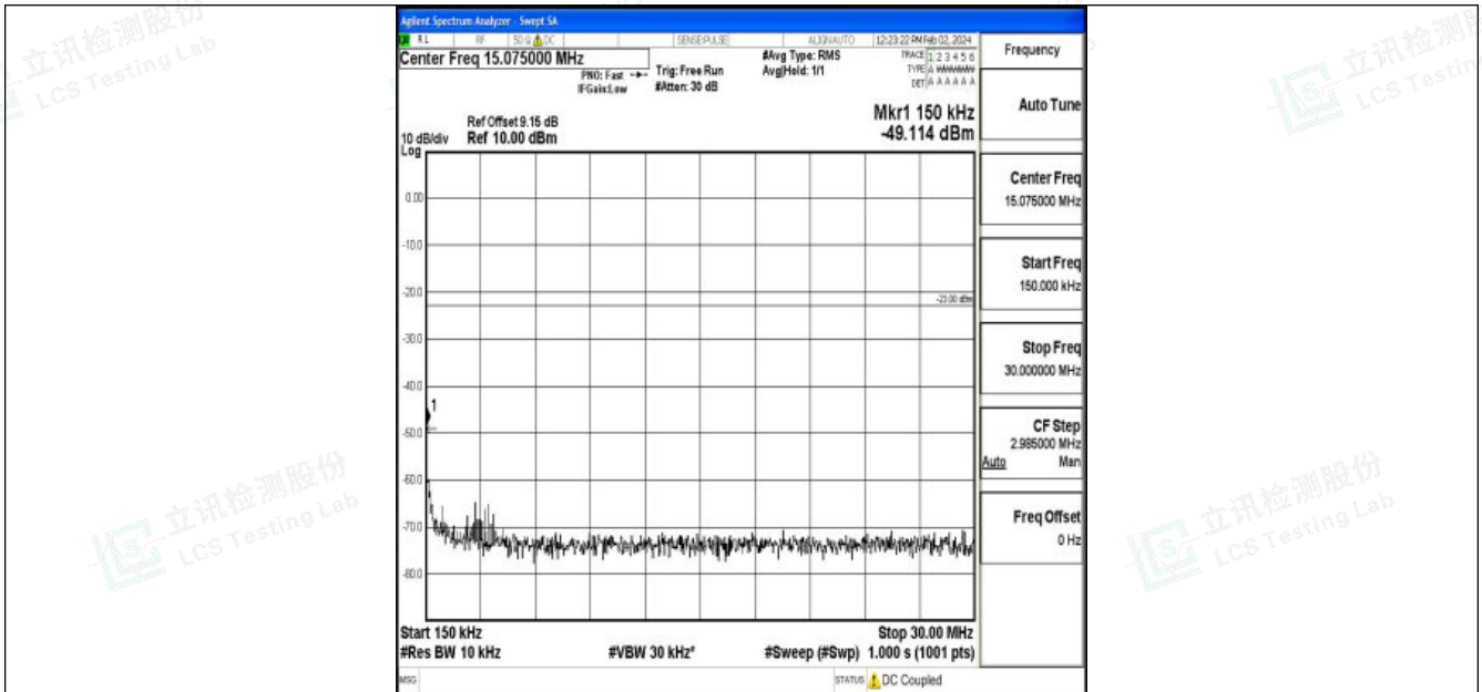
Band26_10MHz_16QAM_26990_1RB#0_0.15~30_0.15~30
