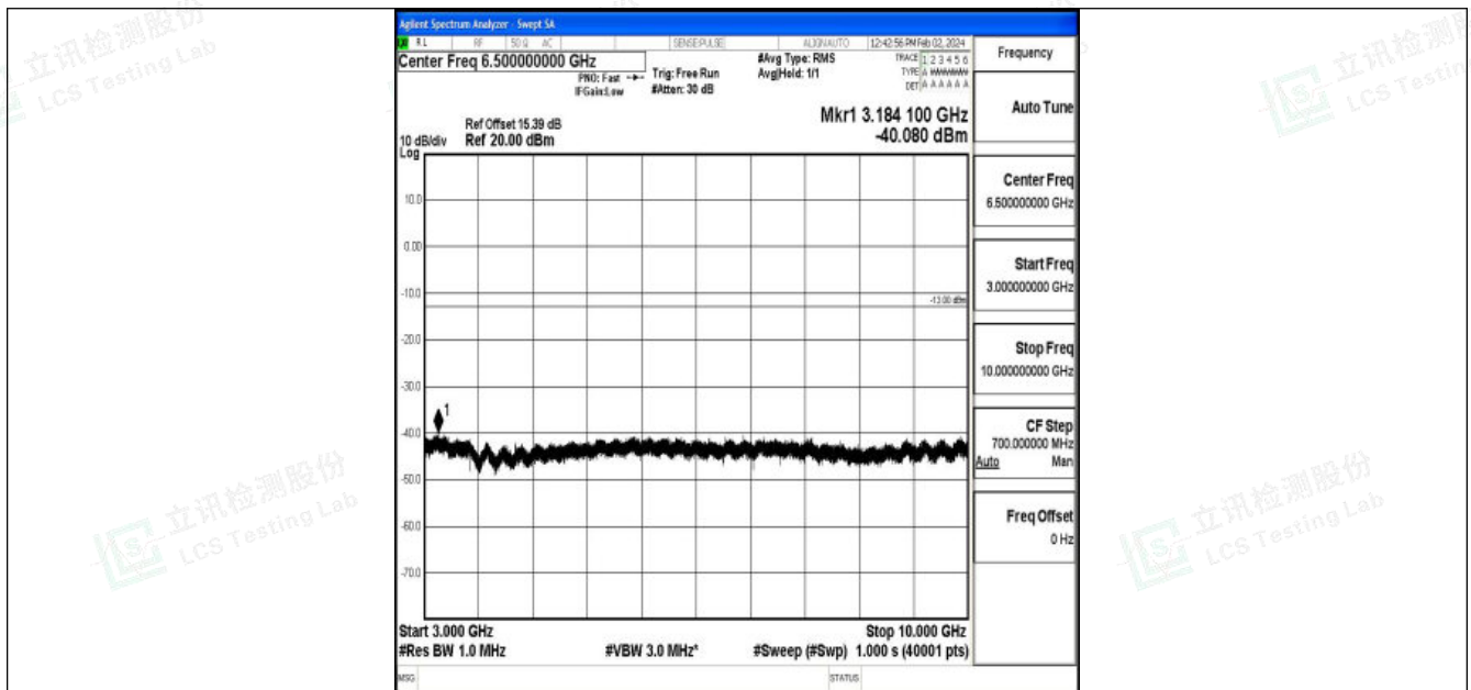
Band26_15MHz_QPSK_26965_1RB#0_3000~10000_3000~10000
