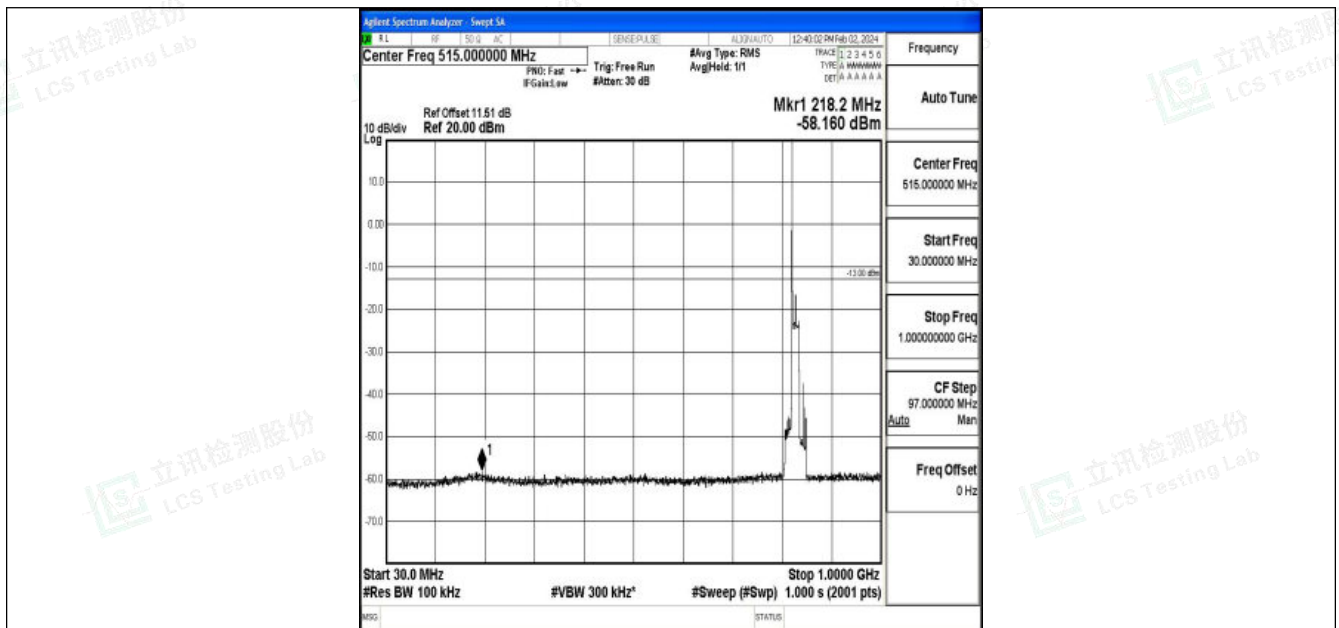
Band26_15MHz_QPSK_26865_1RB#0_30~1000_30~1000
