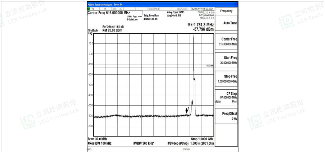
Band26_15MHz_QPSK_26965_1RB#0_30~1000_30~1000
