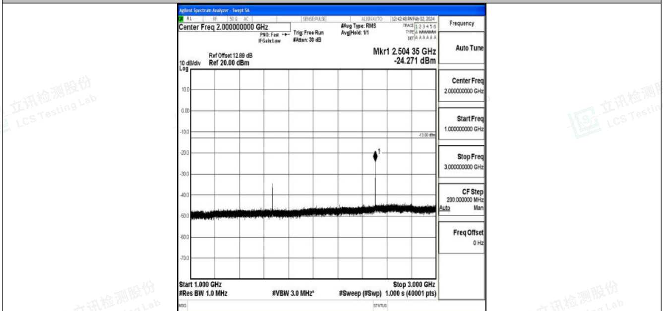
Band26_15MHz_QPSK_26965_1RB#0_1000~3000_1000~3000
