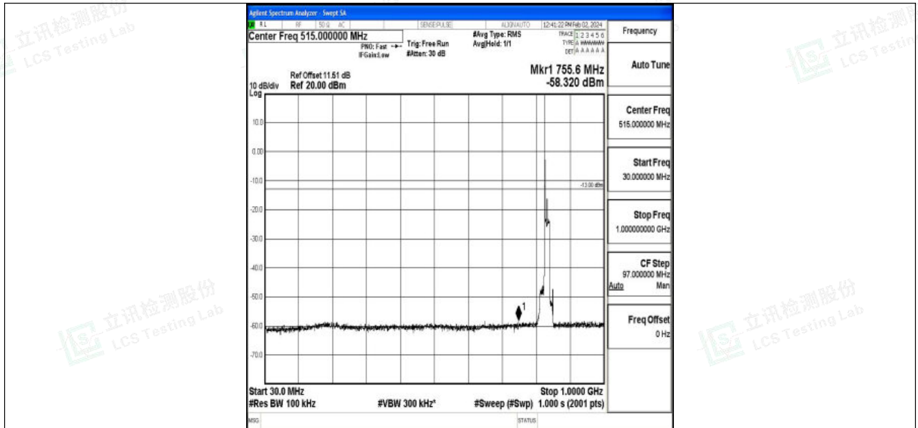
Band26_15MHz_QPSK_26915_1RB#0_30~1000_30~1000
