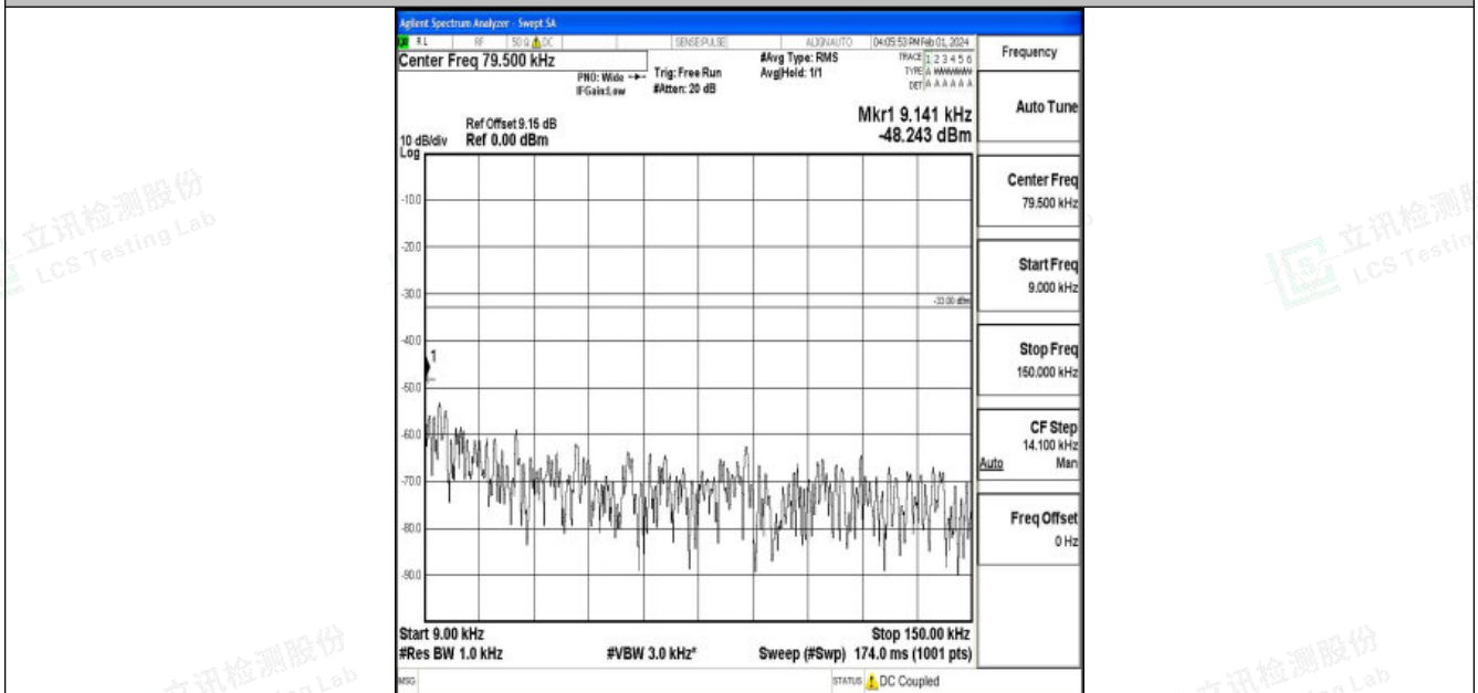
Band12_3MHz_16QAM_23165_1RB#0_0.009~0.15_0.009~0.15
