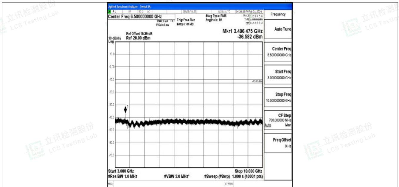
Band12_5MHz_QPSK_23035_1RB#0_3000~10000_3000~10000
