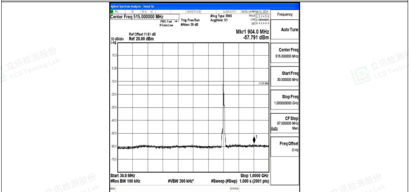
Band12_10MHz_16QAM_23130_1RB#0_30~1000_30~1000
