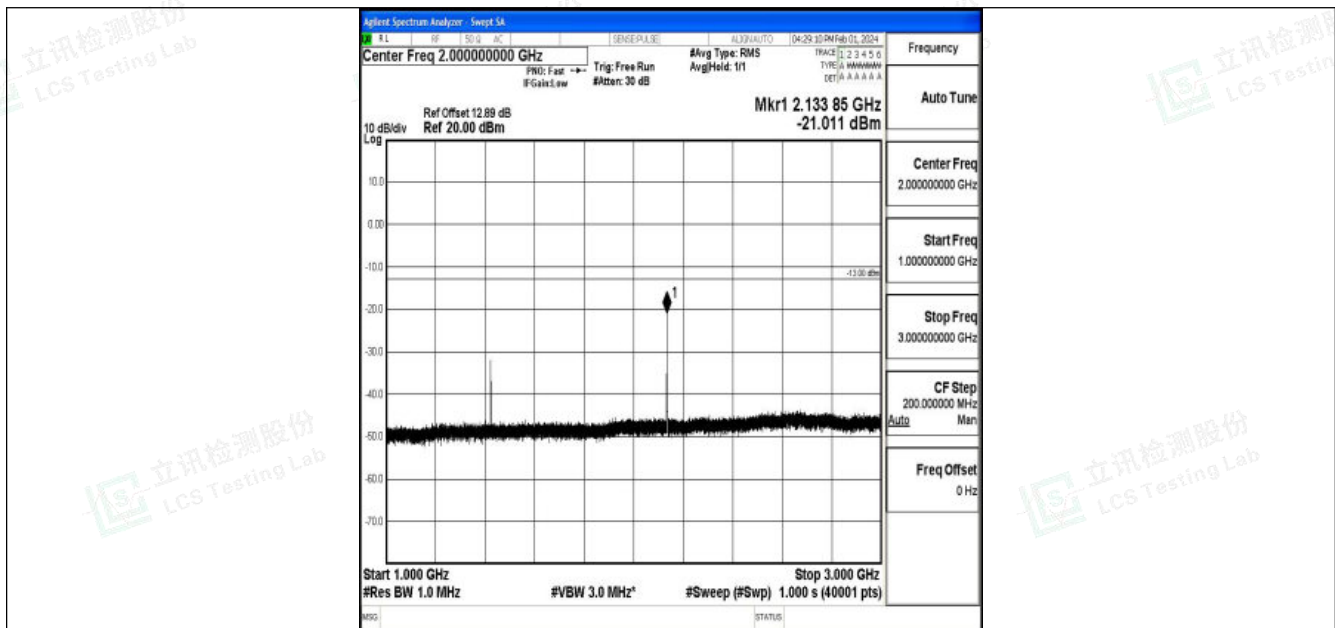
Band12_5MHz_16QAM_23155_1RB#0_1000~3000_1000~3000
