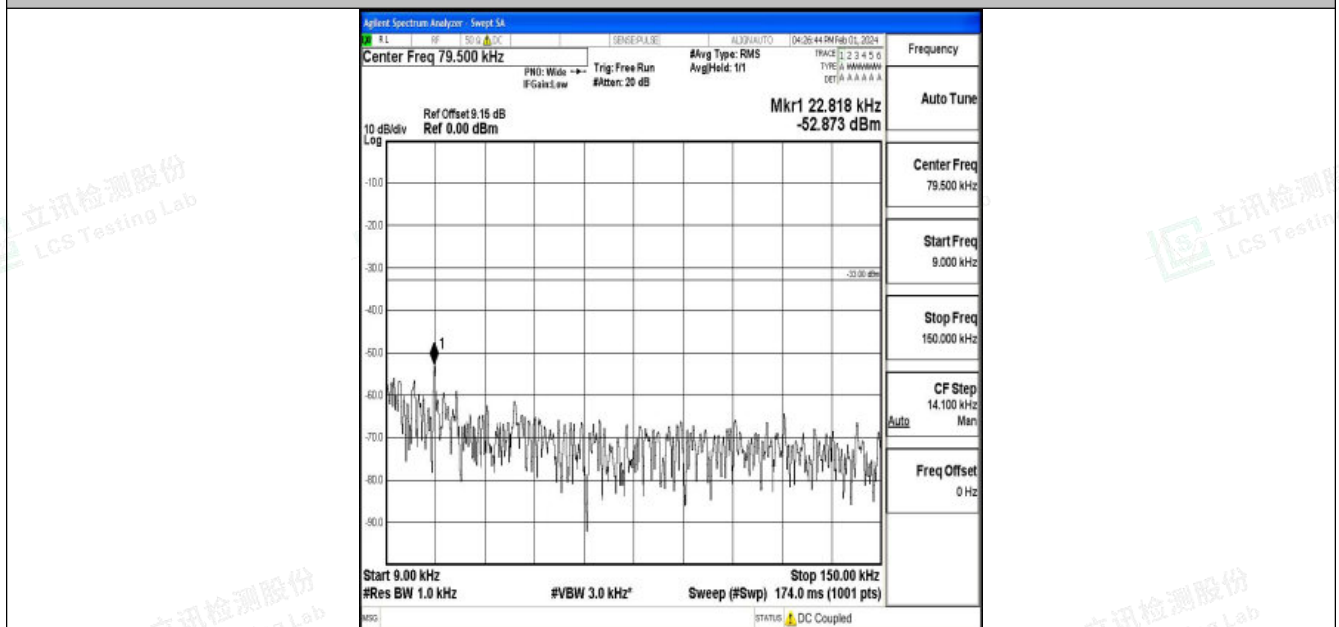
Band12_5MHz_16QAM_23035_1RB#0_0.009~0.15_0.009~0.15
