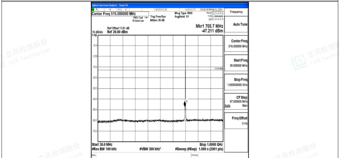
Band12_1.4MHz_16QAM_23095_1RB#0_30~1000_30~1000
