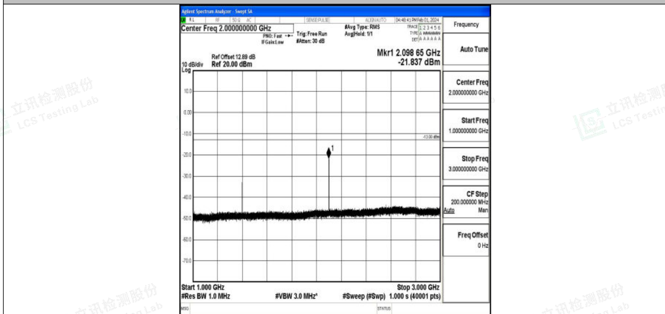
Band12_10MHz_QPSK_23060_1RB#0_1000~3000_1000~3000
