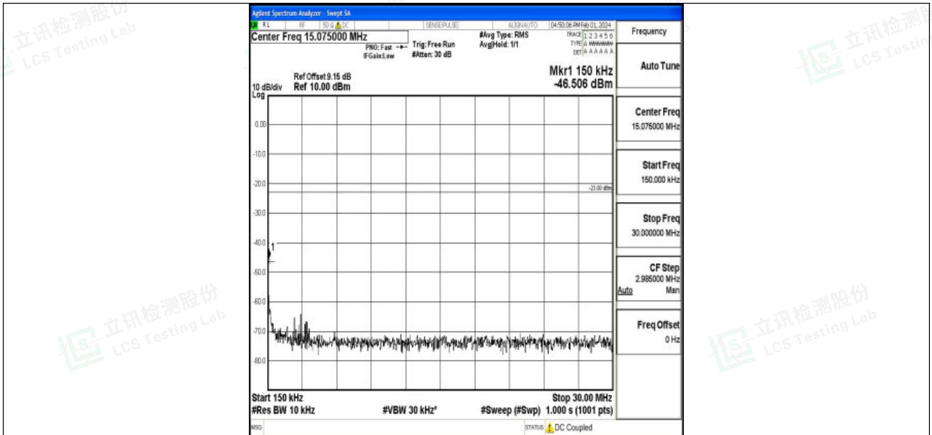
Band12_10MHz_16QAM_23095_1RB#0_0.15~30_0.15~30
