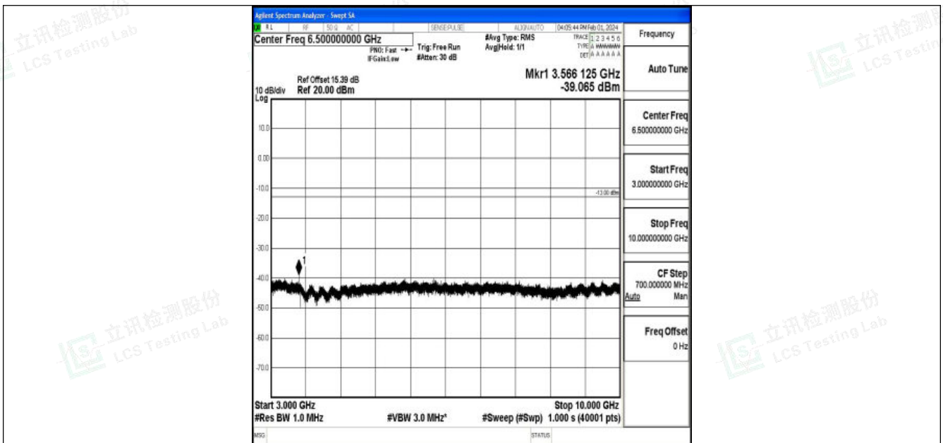
Band12_3MHz_QPSK_23165_1RB#0_3000~10000_3000~10000
