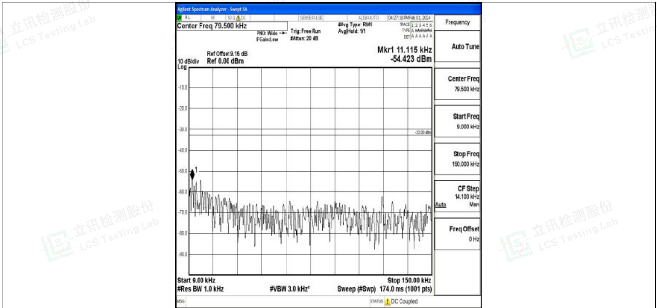
Band12_5MHz_QPSK_23095_1RB#0_0.009~0.15_0.009~0.15
