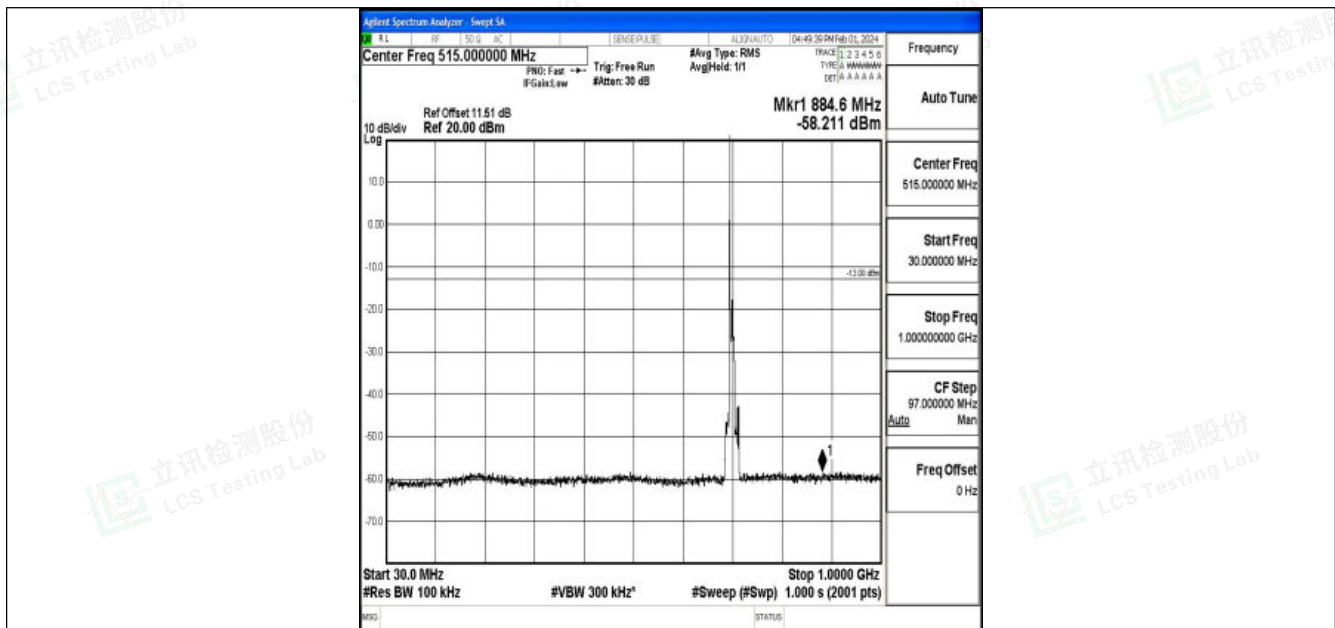
Band12_10MHz_QPSK_23095_1RB#0_30~1000_30~1000
