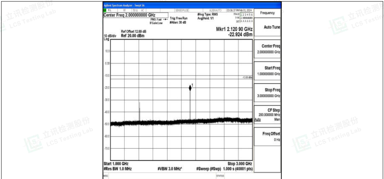
Band12_1.4MHz_16QAM_23095_1RB#0_1000~3000_1000~3000
