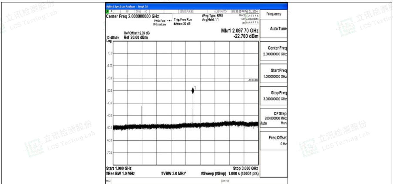
Band12_1.4MHz_16QAM_23017_1RB#0_1000~3000_1000~3000
