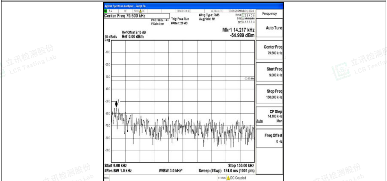
Band12_1.4MHz_16QAM_23095_1RB#0_0.009~0.15_0.009~0.15
