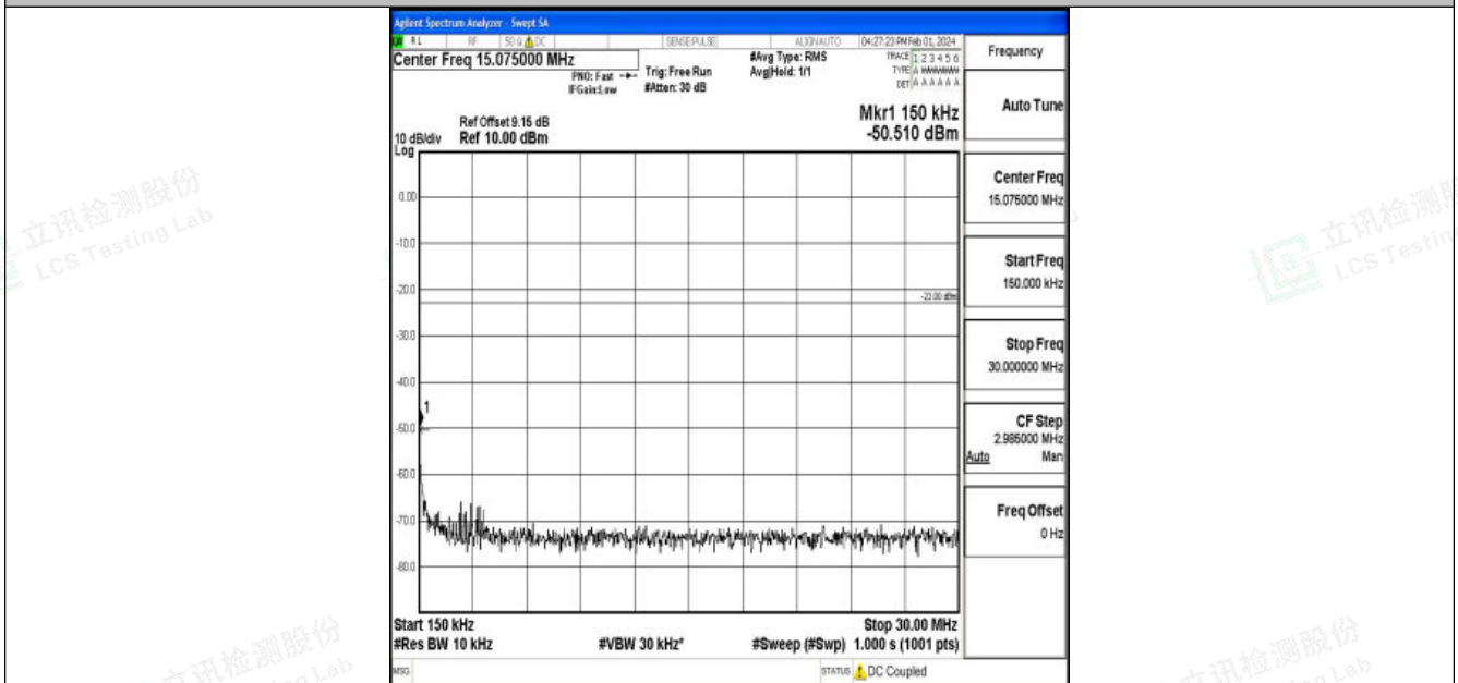
Band12_5MHz_QPSK_23095_1RB#0_0.15~30_0.15~30
