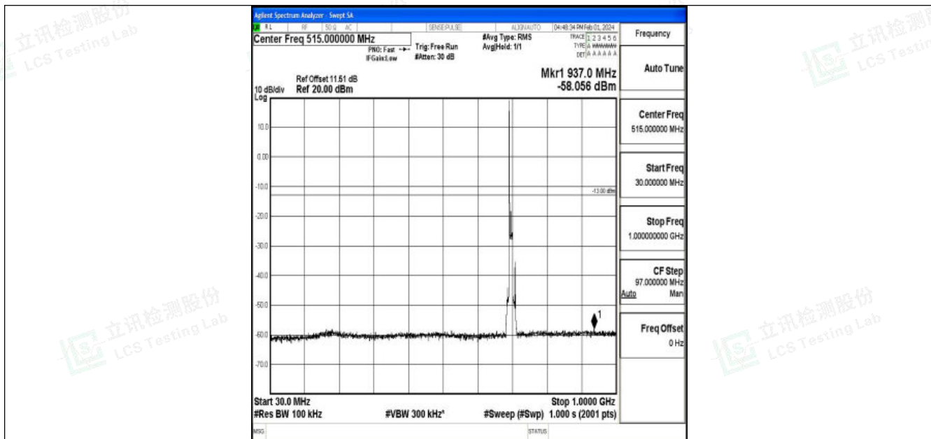
Band12_10MHz_QPSK_23060_1RB#0_30~1000_30~1000
