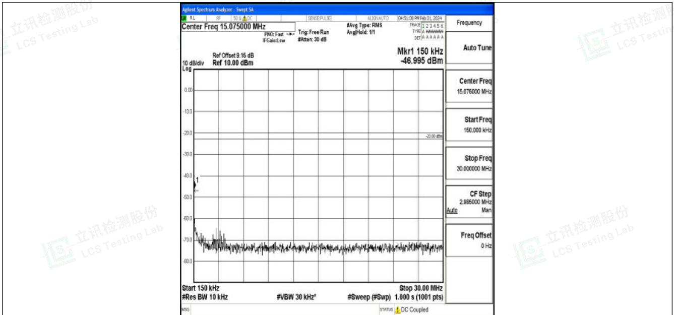
Band12_10MHz_16QAM_23130_1RB#0_0.15~30_0.15~30
