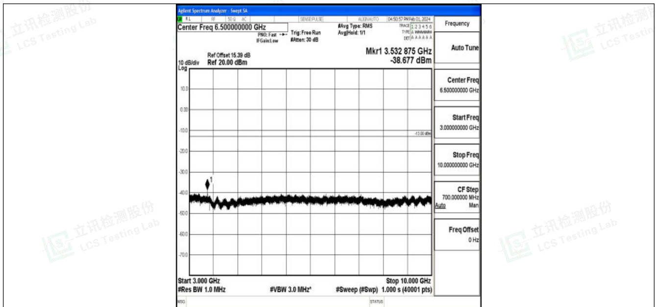
Band12_10MHz_QPSK_23130_1RB#0_3000~10000_3000~10000
