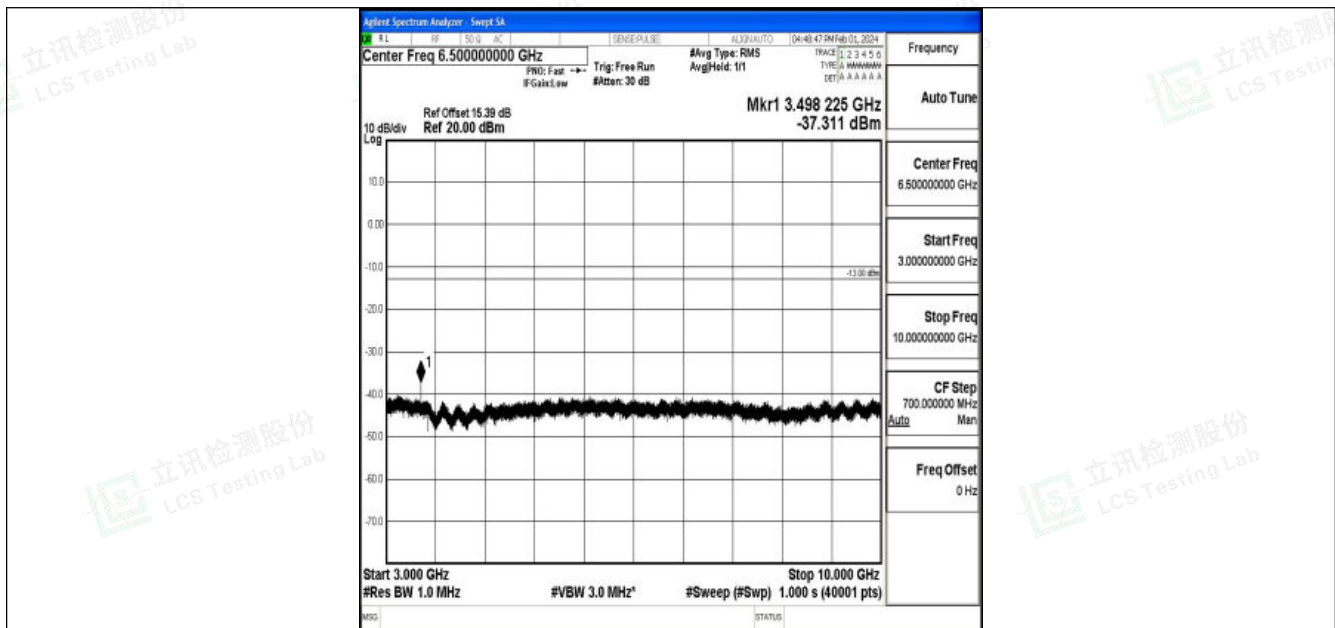
Band12_10MHz_QPSK_23060_1RB#0_3000~10000_3000~10000
