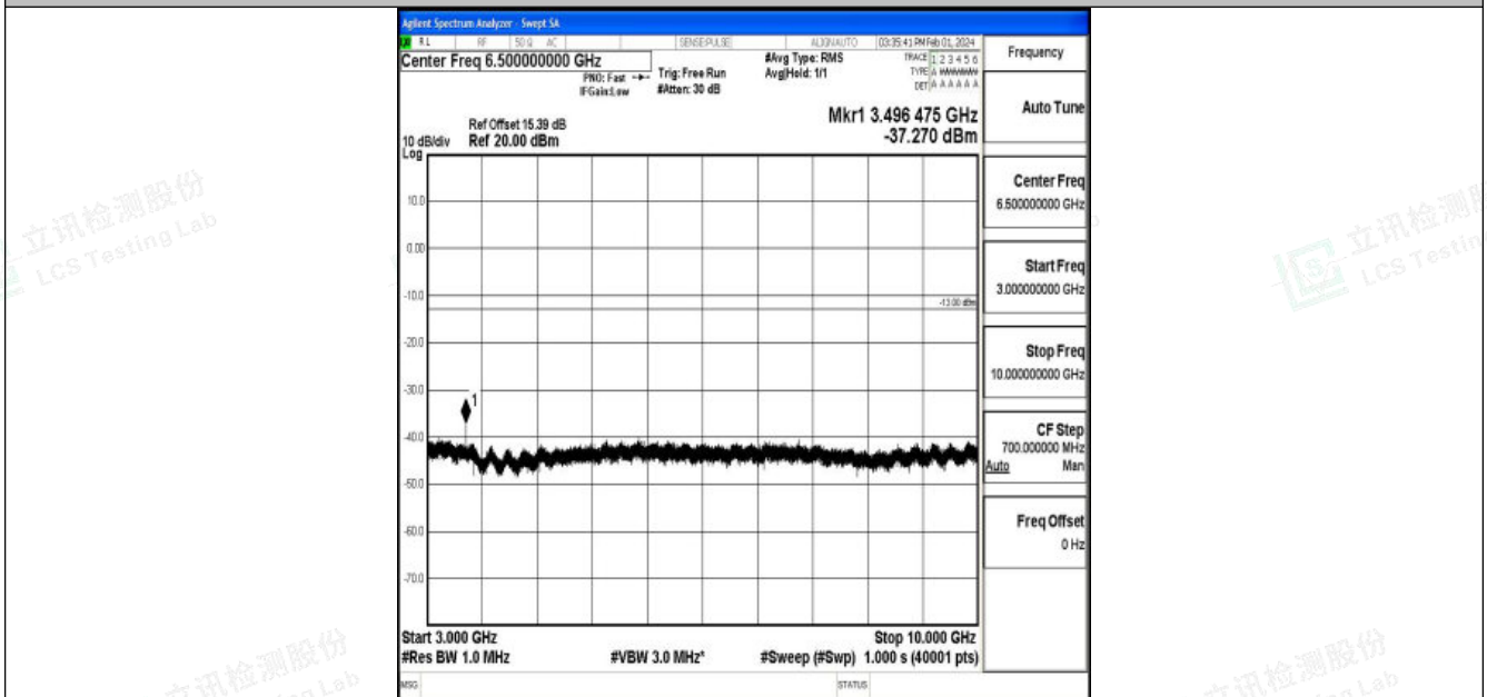
Band12_1.4MHz_16QAM_23017_1RB#0_3000~10000_3000~10000
