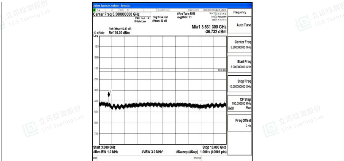
Band12_3MHz_QPSK_23095_1RB#0_3000~10000_3000~10000
