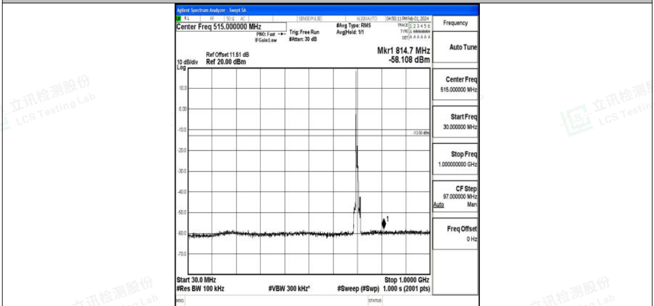
Band12_10MHz_16QAM_23095_1RB#0_30~1000_30~1000
