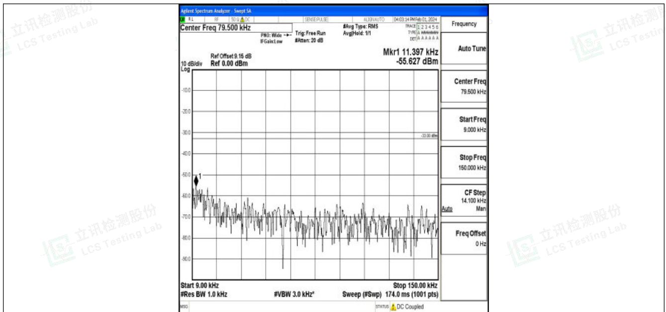
Band12_3MHz_QPSK_23025_1RB#0_0.009~0.15_0.009~0.15
