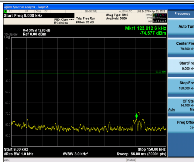
Band5-4233-1-0.009~0.15MHz
