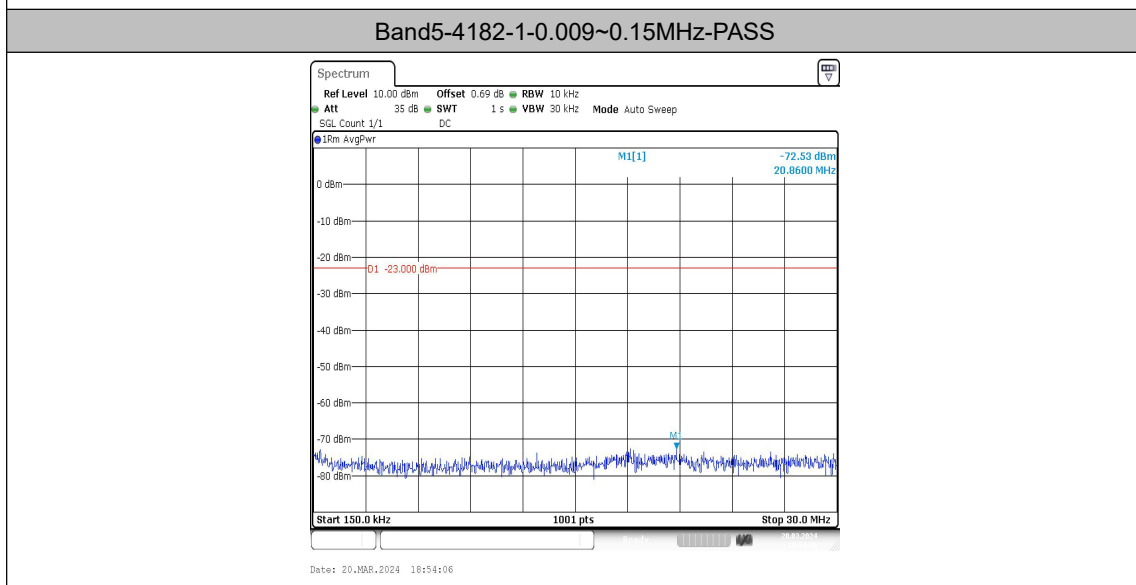
Band5-4182-1-0.15~30MHz-PASS
