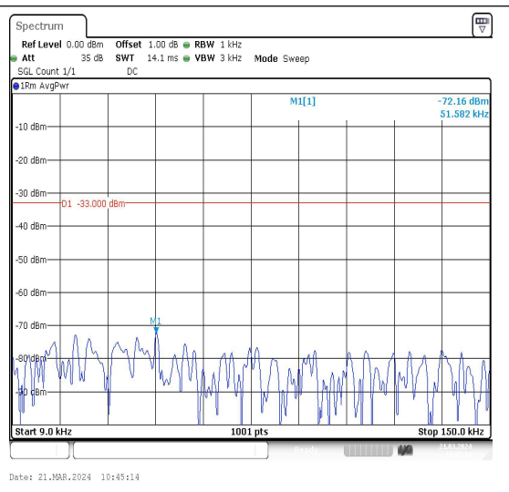
Band5_5MHz_16QAM_20425_1RB#0_0.009~0.15 _0.009~0.15
