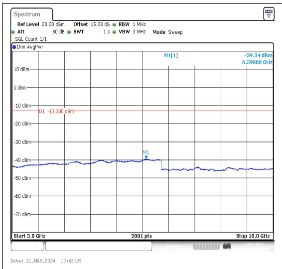
Band5_5MHz_QPSK_20425_1RB#0_3000~1000 0_3000~10000
