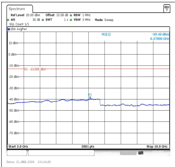
Band5_3MHz_QPSK_20415_1RB#0_3000~1000 0_3000~10000
