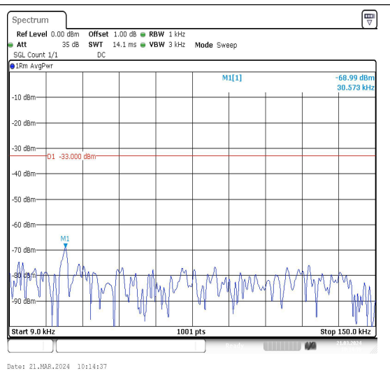
Band5_3MHz_16QAM_20415_1RB#0_0.009~0.15 _0.009~0.15
