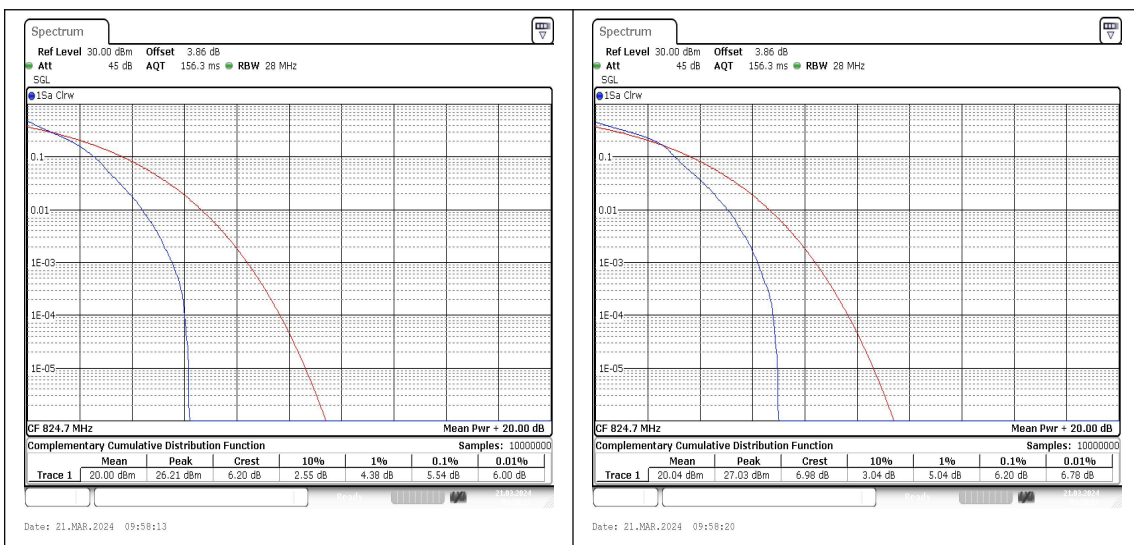
Band5-1.4MHz-QPSK-20407-1RB#0-PASS Band5-1.4MHz-16QAM-20407-1RB#0-PASS
