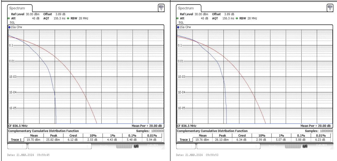
Band5-1.4MHz-QPSK-20525-1RB#0-PASS Band5-1.4MHz-16QAM-20525-1RB#0-PASS
