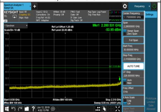
802.11n(HT40),2422MHz,Ant1,Plot 3,30MHz~2310MHz
