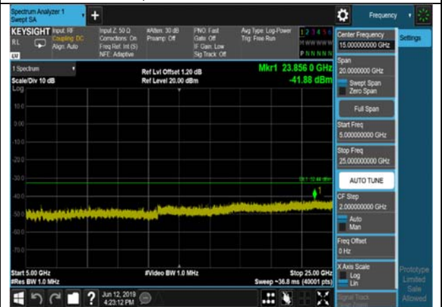
802.11n(HT40),2452MHz,Ant1,Plot 5,5000MHz~25000MHz
