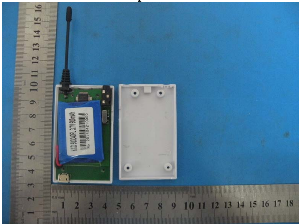
Internal photo of EUT
