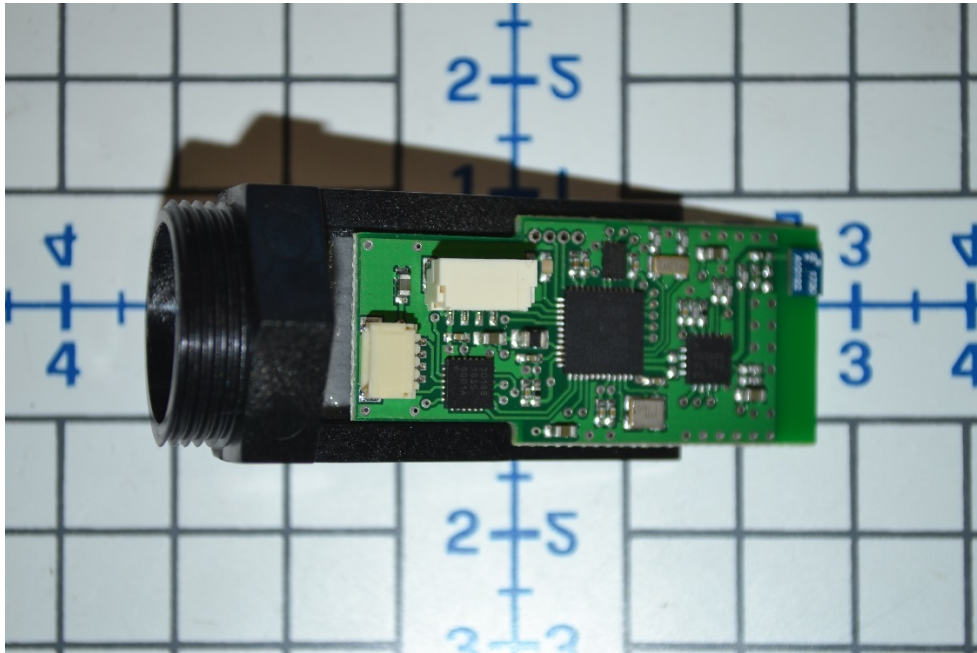
Internal - PCB Top View
