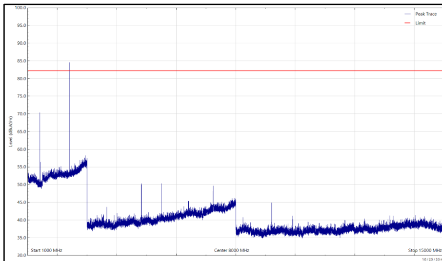
Figure 11 - BLE – 2480 MHz (CH39), LTE Band 12 – 707.5 MHz, SRD – 915 MHz, ISM – 16 MHz, 1 GHz to 15 GHz, Horizontal (Peak)
