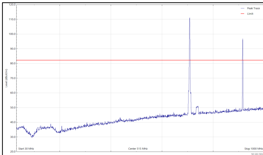
Figure 10 - BLE – 2480 MHz (CH39), LTE Band 12 – 707.5 MHz, SRD – 915 MHz, ISM – 16 MHz, 30 MHz to 1 GHz, Horizontal (Peak)
