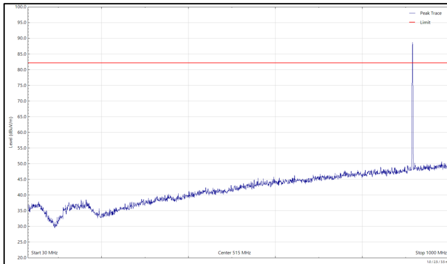
Figure 6 - 802.11b – 2412 MHz (CH1), UMTS FDDII – 1852.4 MHz, SRD – 915 MHz, ISM – 16 MHz, 30 MHz to 1 GHz, Horizontal (Peak)
