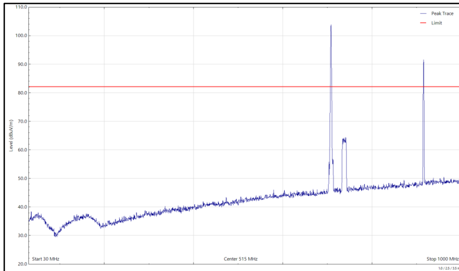
Figure 12 - BLE – 2480 MHz (CH39), LTE Band 12 – 707.5 MHz, SRD – 915 MHz, ISM – 16 MHz, 30 MHz to 1 GHz, Vertical (Peak)
