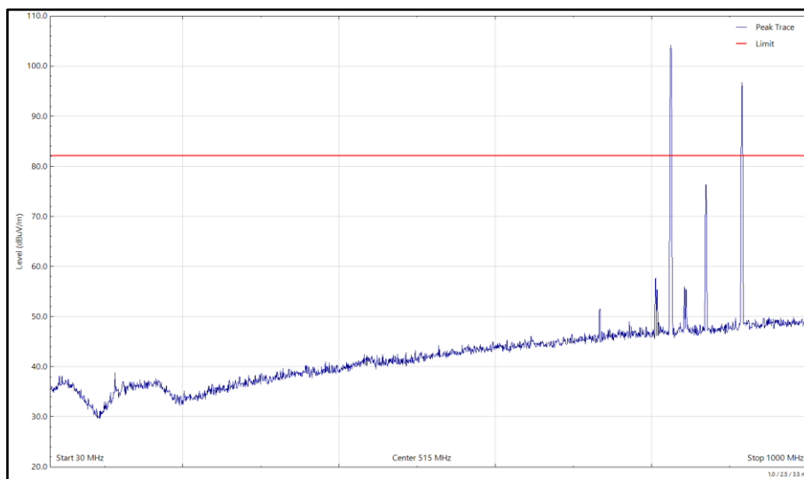
Figure 2 - 802.11b – 2412 MHz (CH1), GSM850 – 824.2 MHz, SRD – 915 MHz, ISM – 16 MHz, 30 MHz to 1 GHz, Horizontal (Peak)
