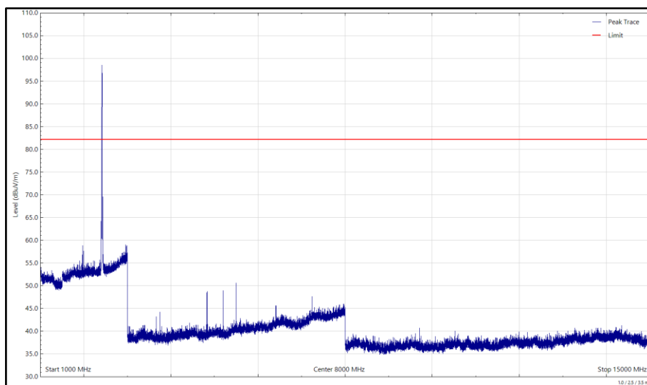
Figure 3 - 802.11b – 2412 MHz (CH1), GSM850 – 824.2 MHz, SRD – 915 MHz, ISM – 16 MHz, 1 GHz to 15 GHz, Horizontal (Peak)
