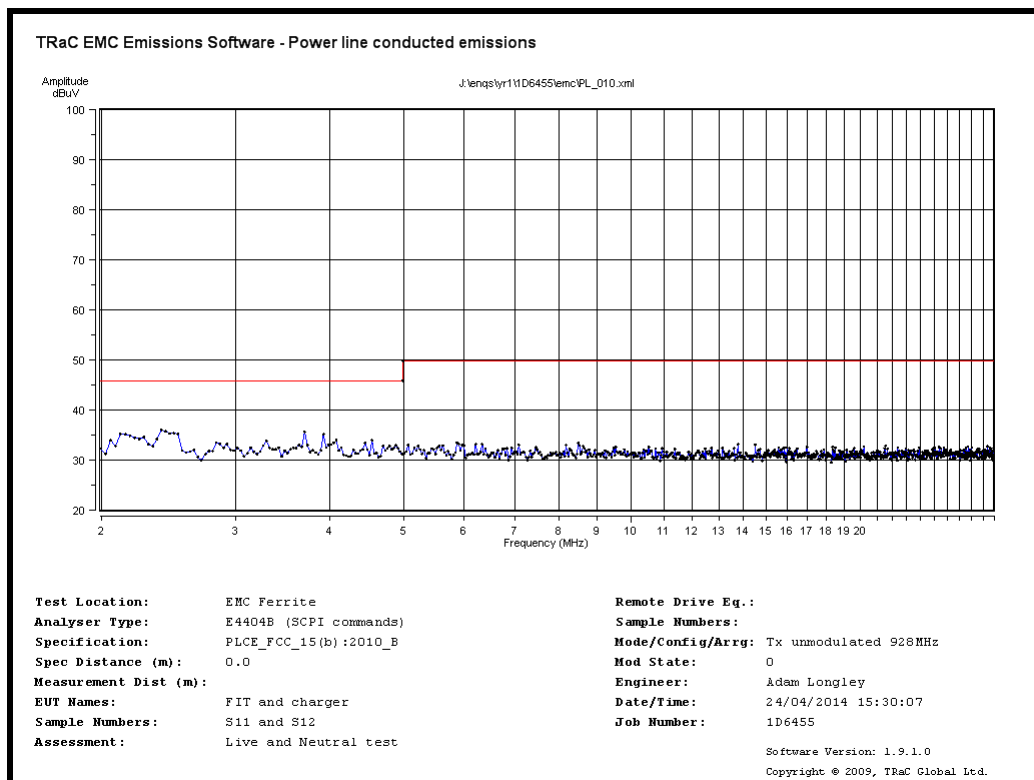
Transmitting at 927.6MHz – Power Line Conducted Spurious Emissions 2MHz to 30MHz
