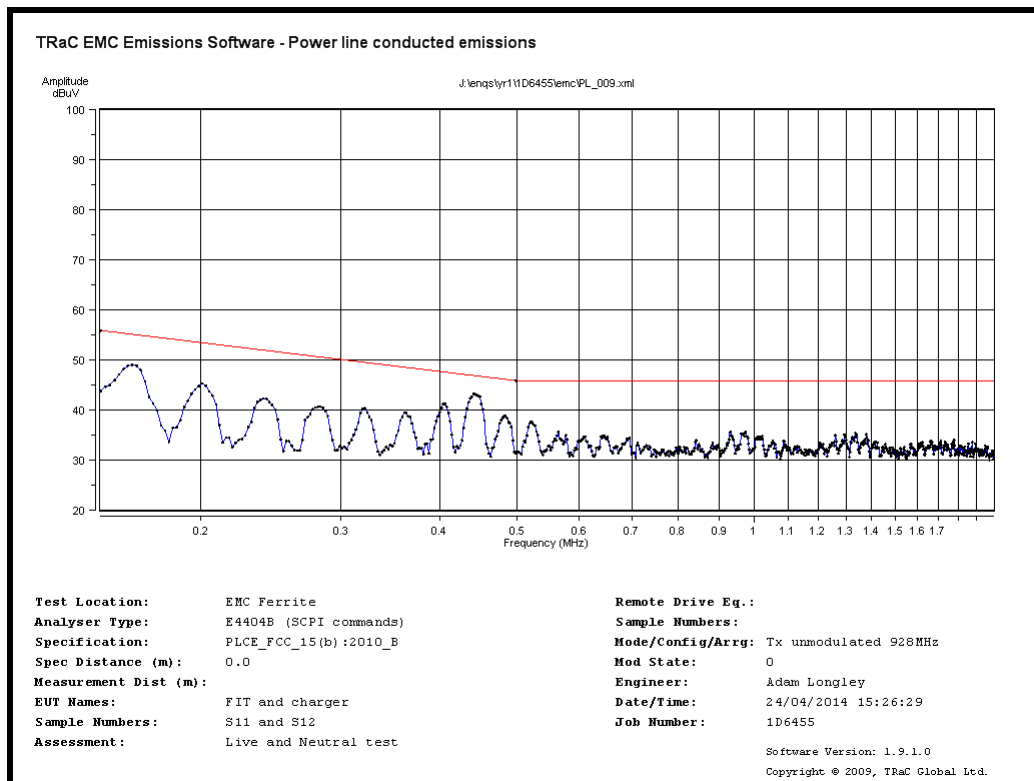
Transmitting at 927.6MHz – Power Line Conducted Spurious Emissions 150kHz to 2MHz
