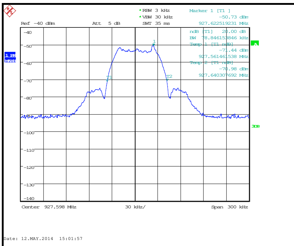
Fc = 927.6 MHz - 20dB Bandwidth
