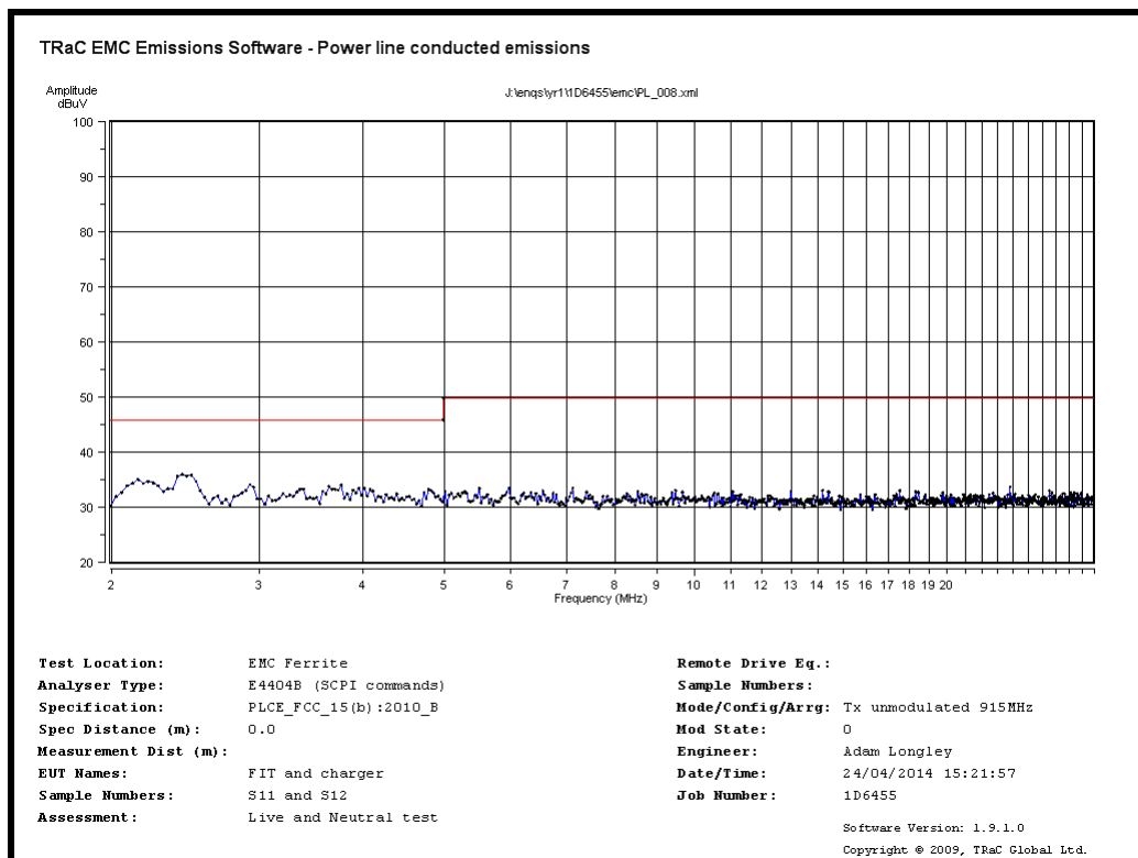
Transmitting at 915.25MHz – Power Line Conducted Spurious Emissions 2MHz to 30MHz
