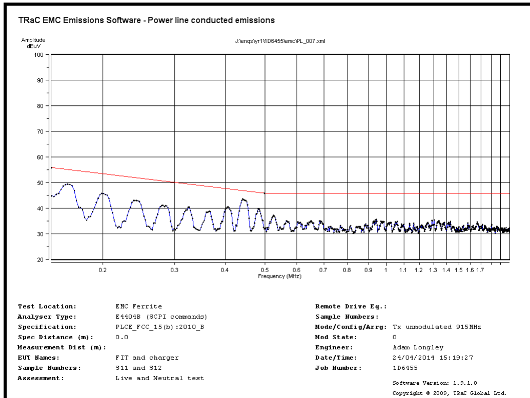
Transmitting at 915.25MHz – Power Line Conducted Spurious Emissions 150kHz to 2MHz
