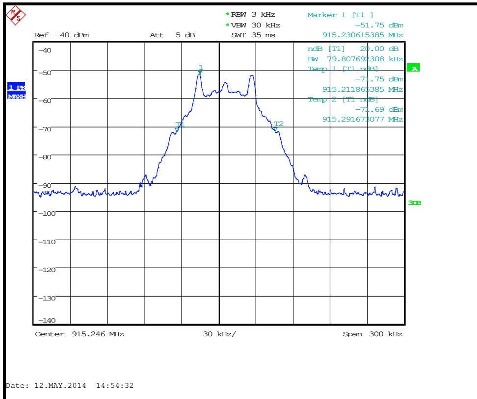
Fc = 915.25 MHz - 20dB Bandwidth
