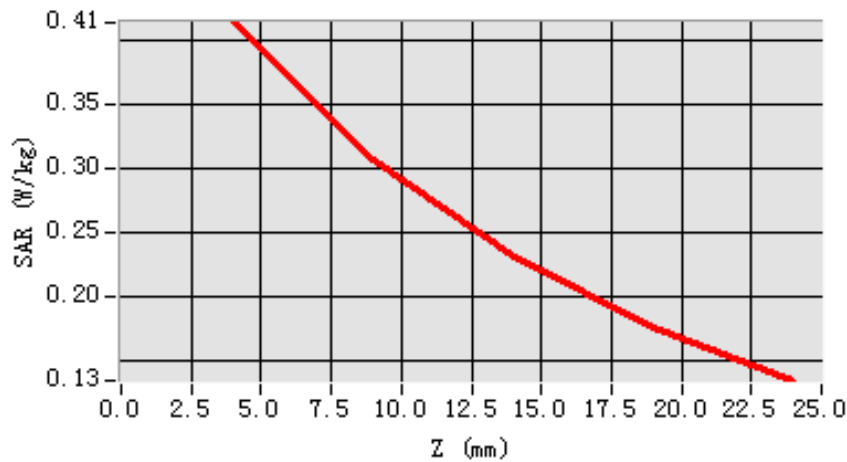
SAR, Z Axis Scan (X = -30, Y = -15)
