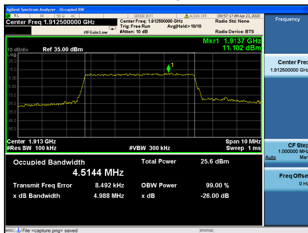
Band25 / 5MHz / High CH / 16QAM
