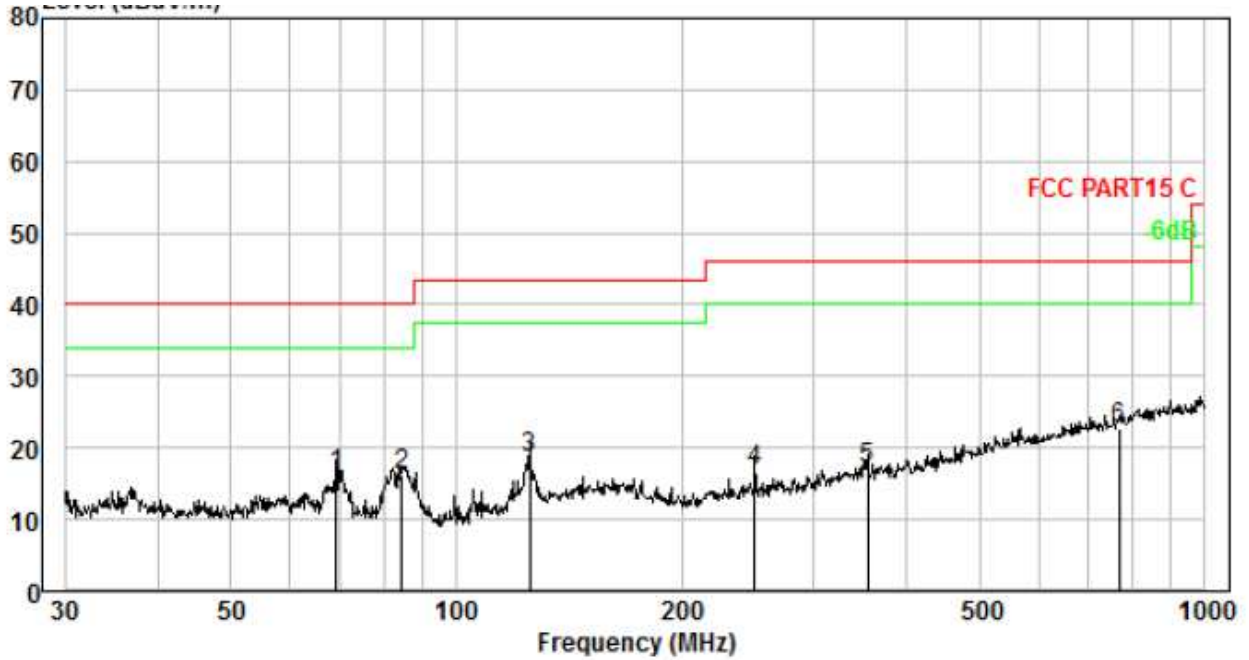
Test plot for Vertical: 2404MHz
