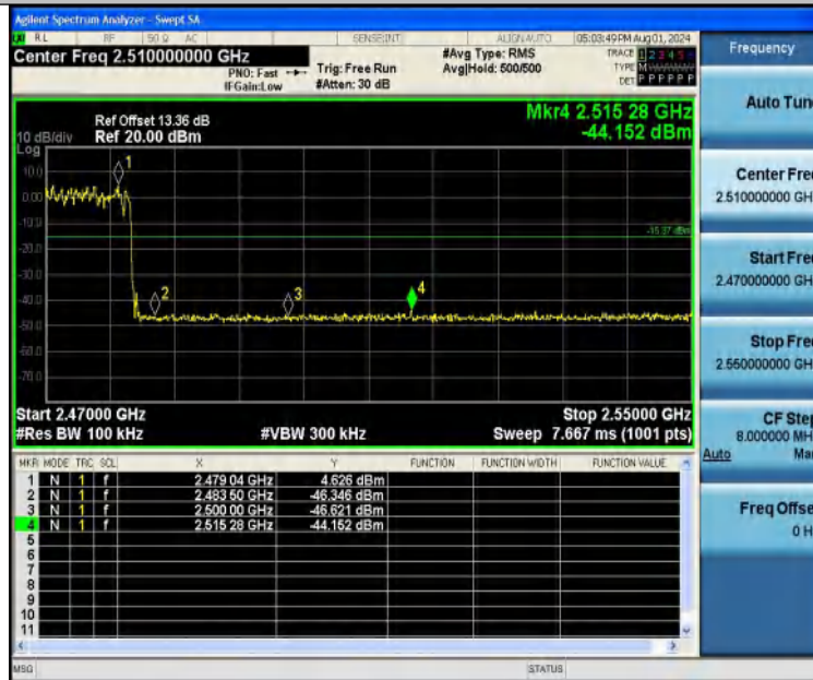
2DH5-Ant1-Hop_2480-PASS
