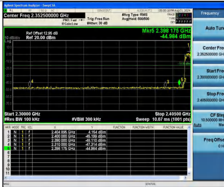
2DH5-Ant1-Hop_2402-PASS
