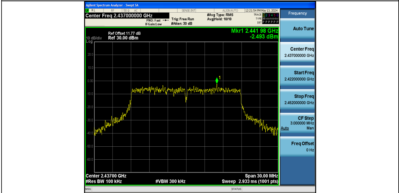
11N20SISO-Ant1-2437-0~Reference-PASS
