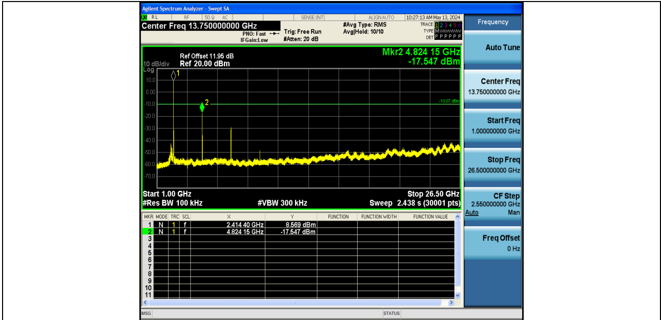
11B-Ant1-2412-1000~26500-PASS
