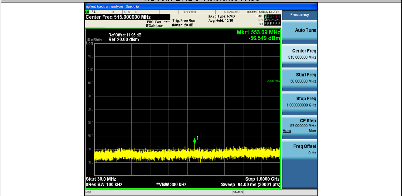
11B-Ant1-2412-30~1000-PASS
