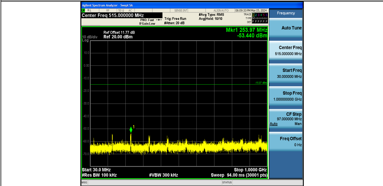
BLE_1M-Ant1-2440-30~1000-PASS
