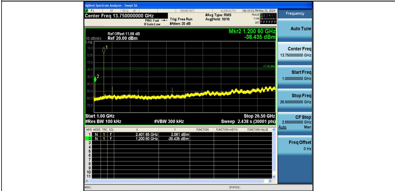
BLE_2M-Ant1-2402-1000~26500-PASS
