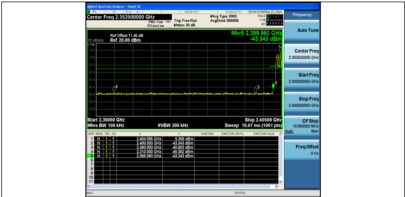
DH5-Ant1-Hop_2402-PASS
