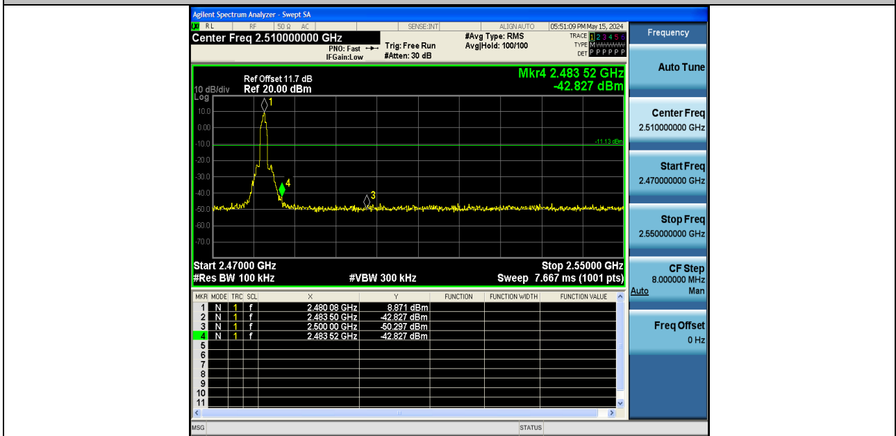
3DH5-Ant1-2480-PASS
