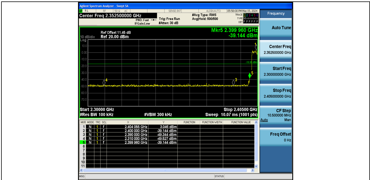
2DH5-Ant1-Hop_2402-PASS
