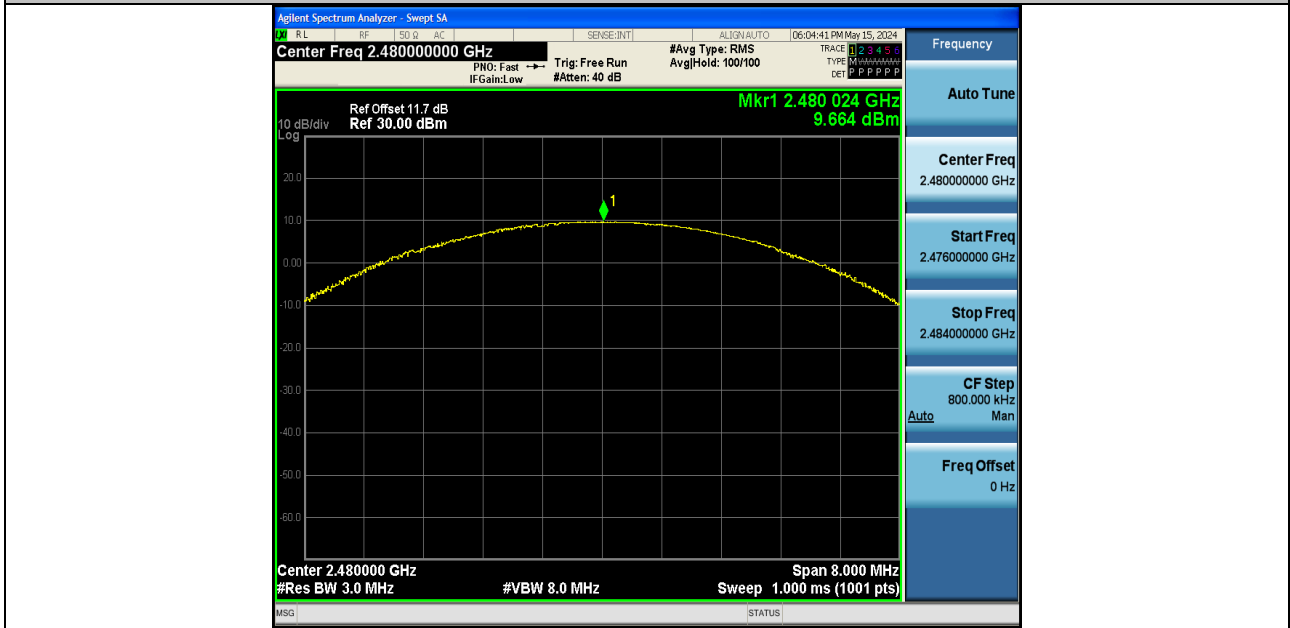
2DH5-Ant1-2480-PASS
