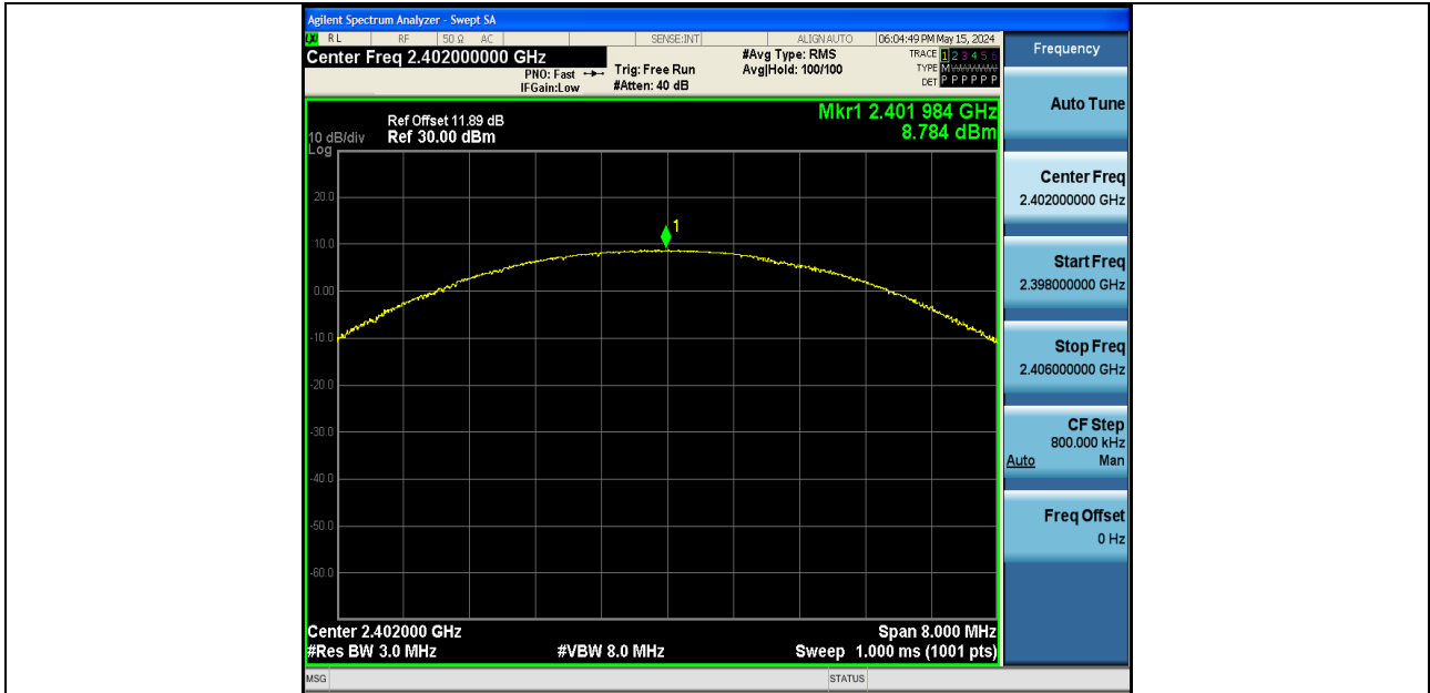
3DH5-Ant1-2402-PASS
