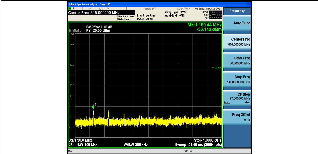
DH5-Ant1-2441-30~1000-PASS
