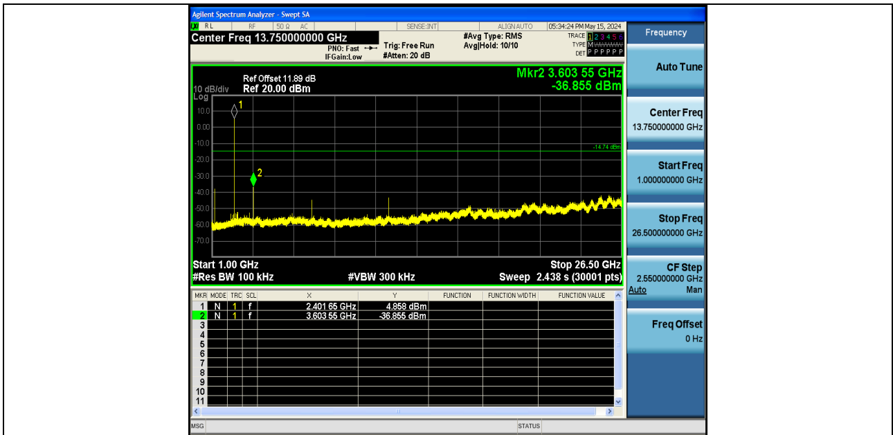
DH5-Ant1-2402-1000~26500-PASS
