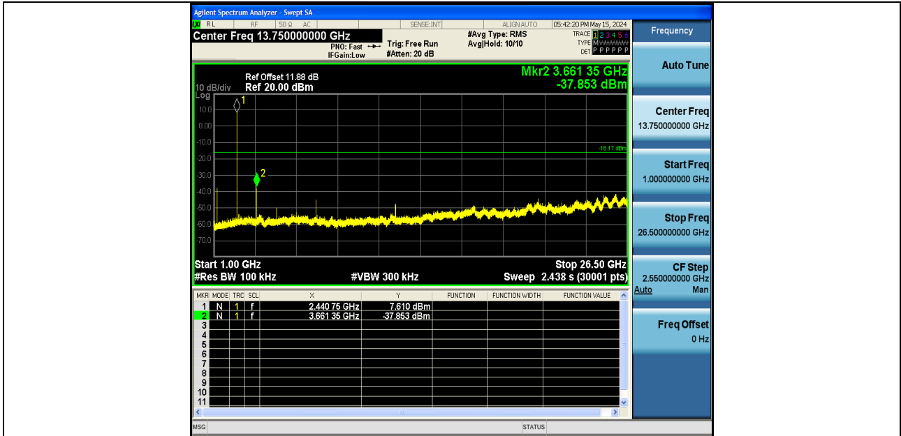
2DH5-Ant1-2441-1000~26500-PASS
