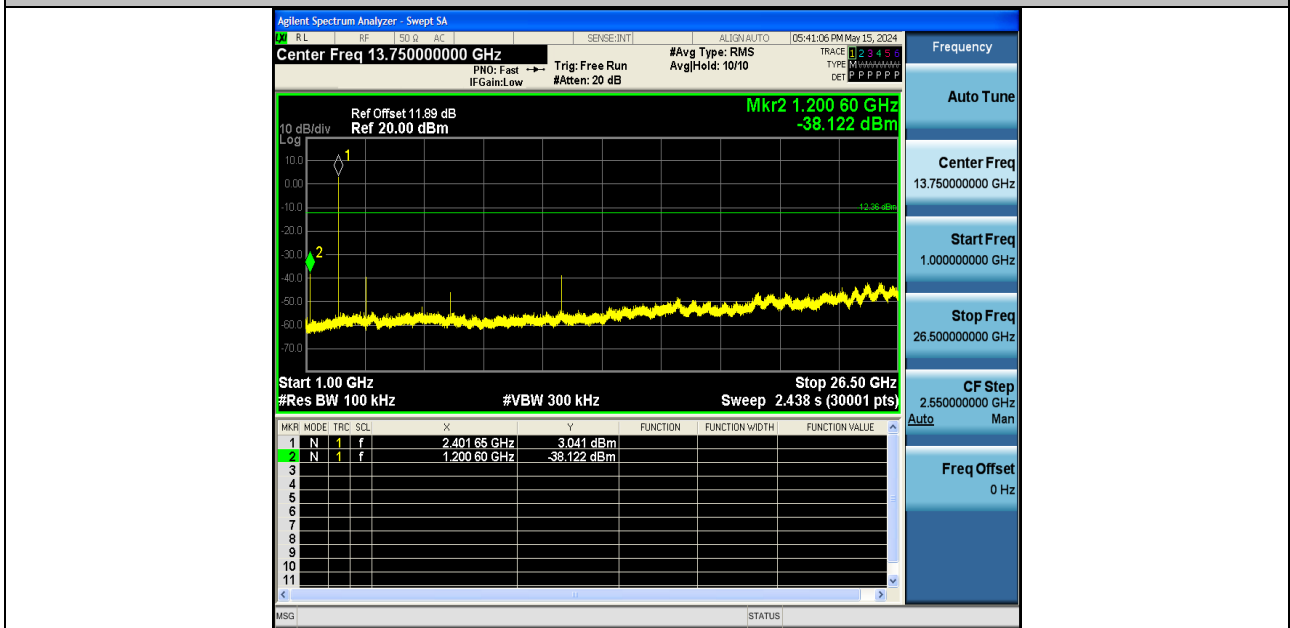
2DH5-Ant1-2402-1000~26500-PASS
