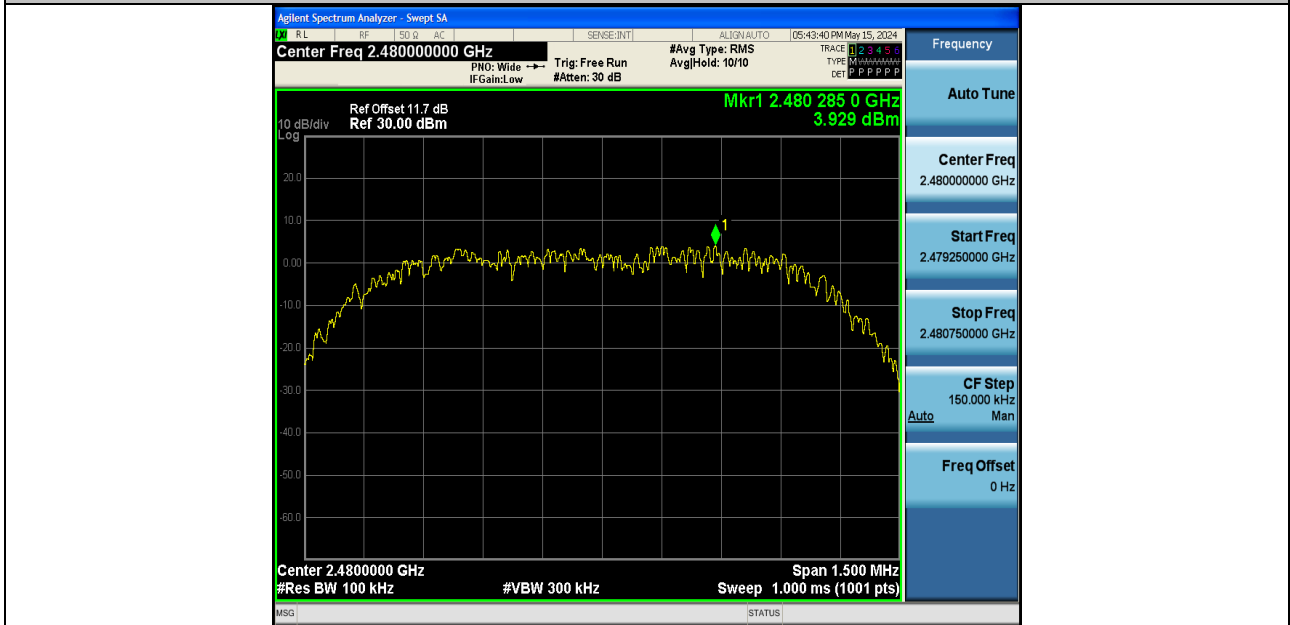
2DH5-Ant1-2480-0~Reference-PASS
