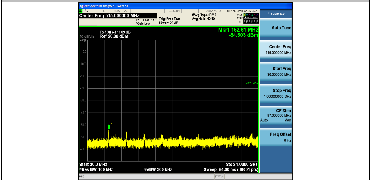
3DH5-Ant1-2402-30~1000-PASS
