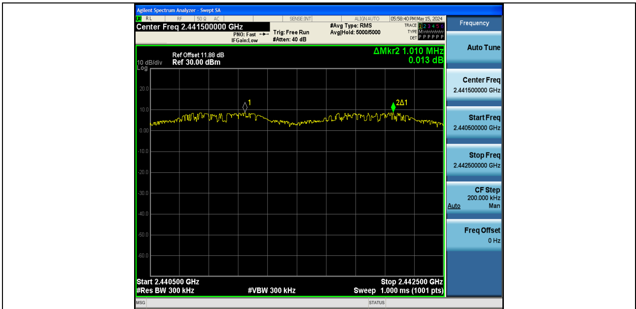
2DH5-Ant1-Hop-PASS
