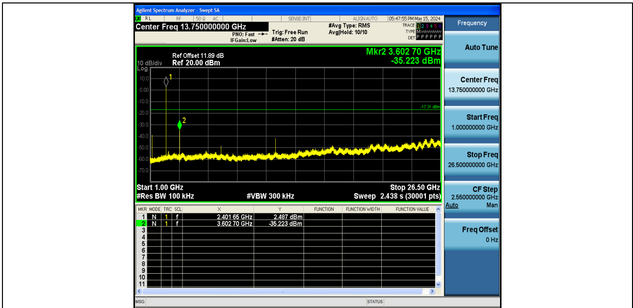
3DH5-Ant1-2402-1000~26500-PASS
