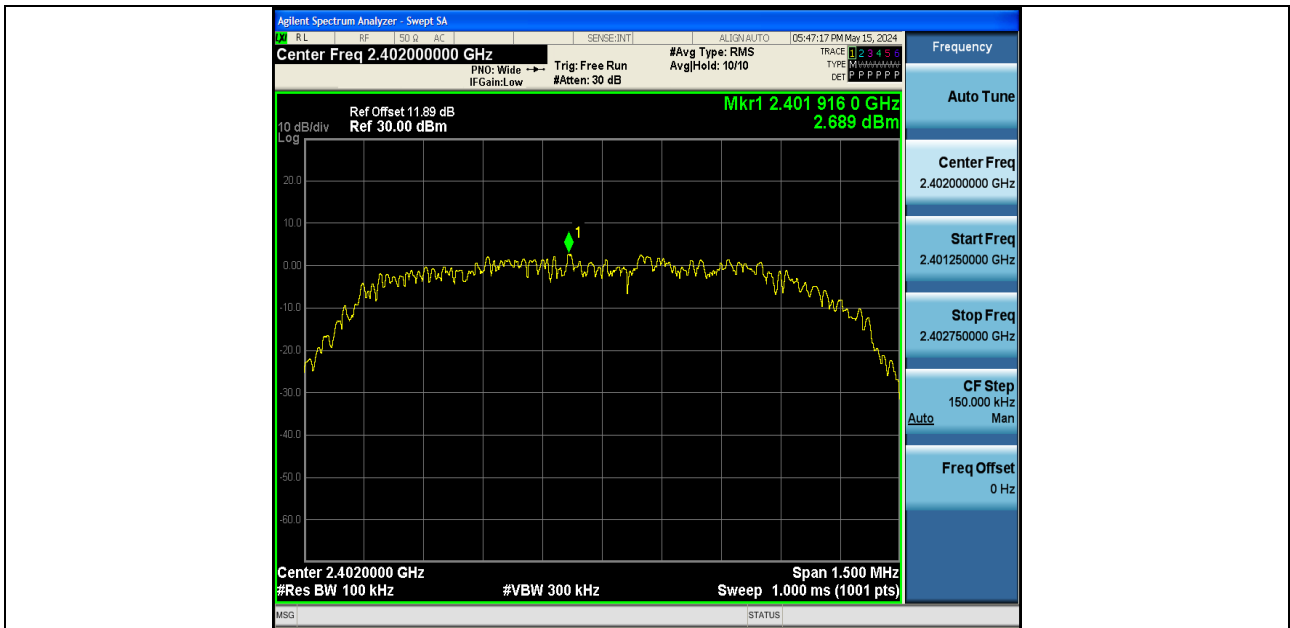
3DH5-Ant1-2402-0~Reference-PASS
