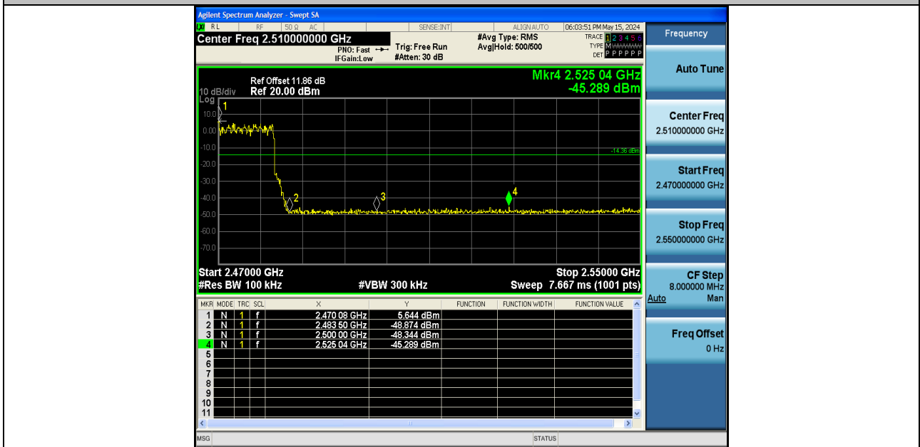
3DH5-Ant1-Hop_2480-PASS
