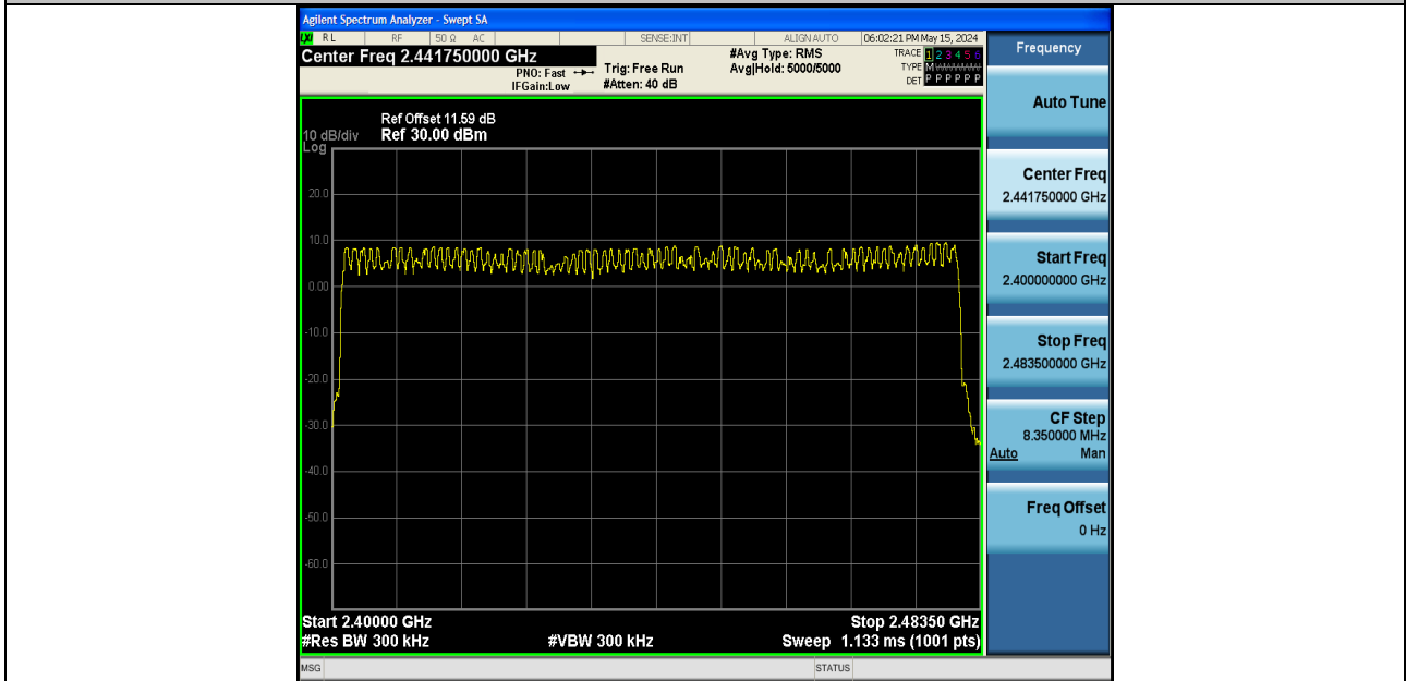
3DH5-Ant1-Hop-PASS
