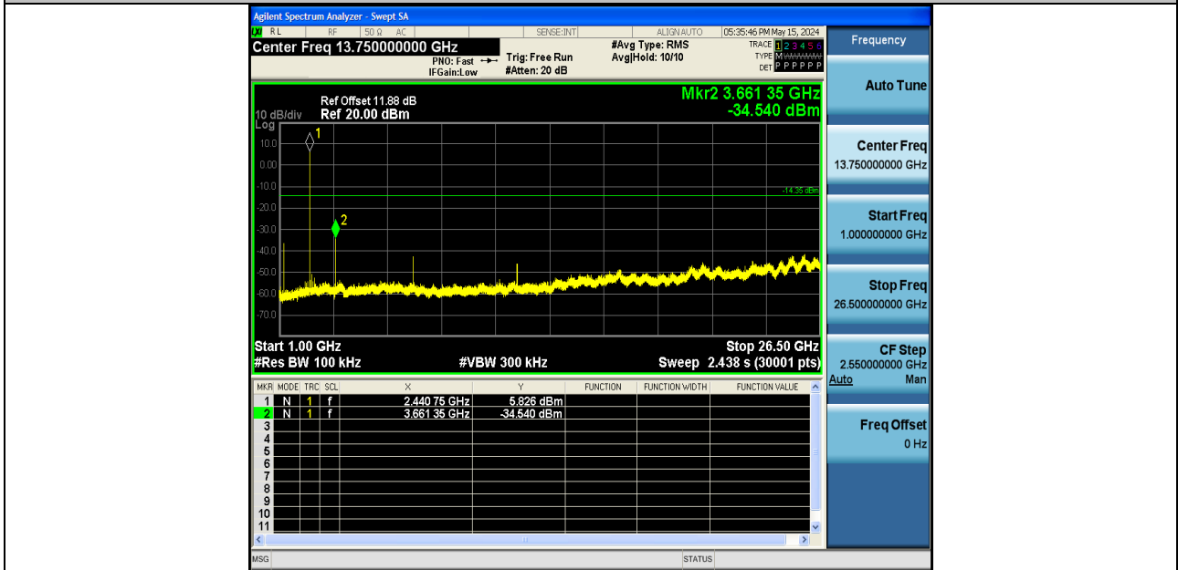
DH5-Ant1-2441-1000~26500-PASS
