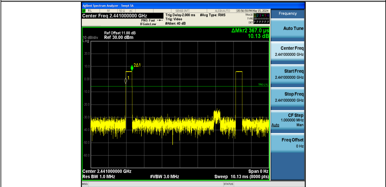
DH1-Ant1-Hop-PASS
