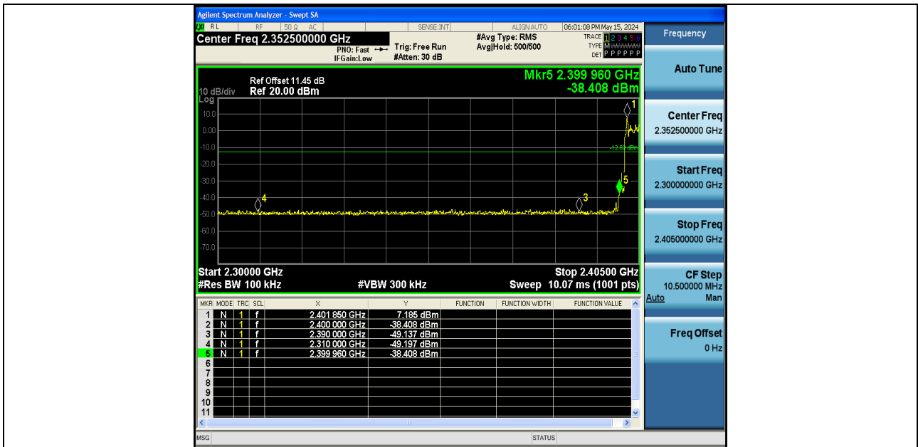
3DH5-Ant1-Hop_2402-PASS
