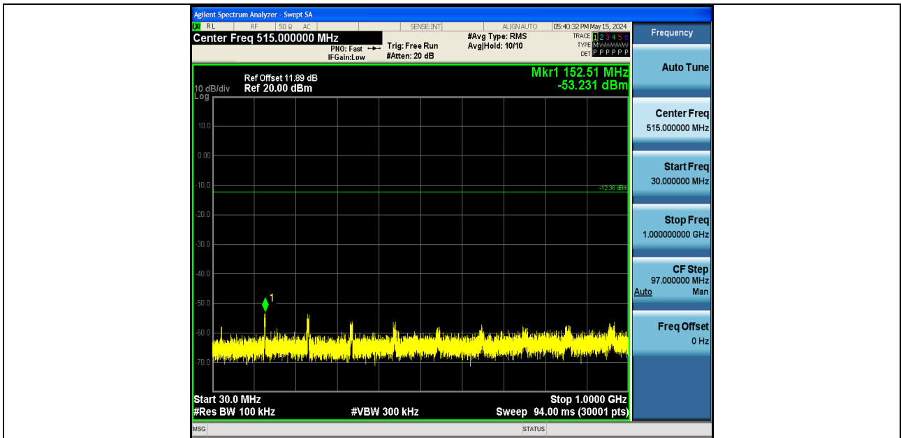
2DH5-Ant1-2402-30~1000-PASS
