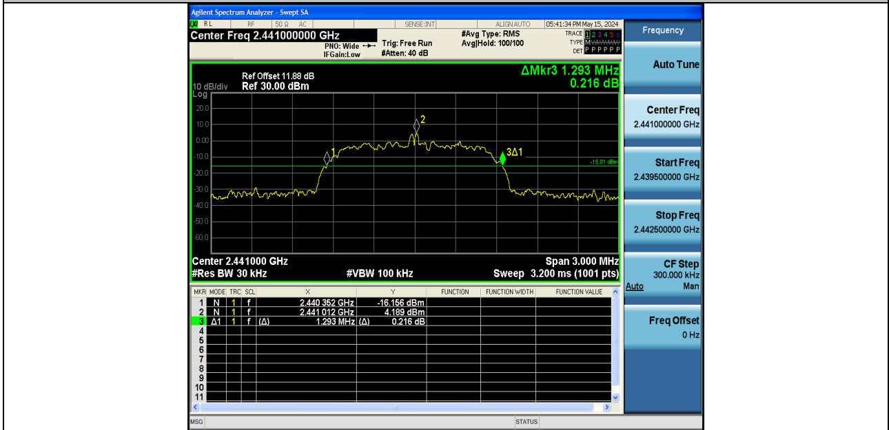
2DH5-Ant1-2441
