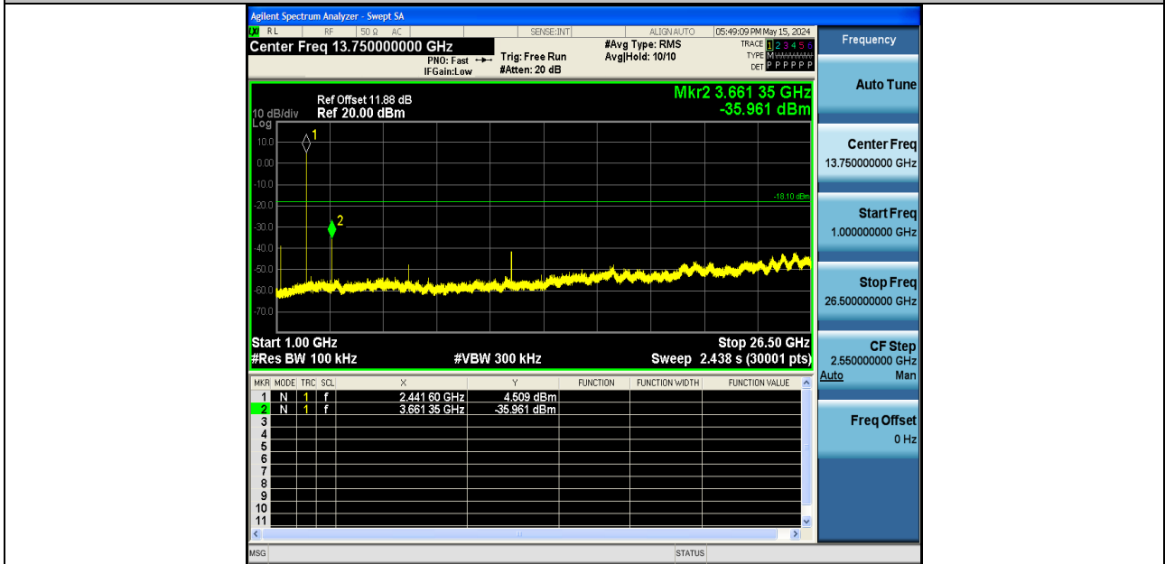
3DH5-Ant1-2441-1000~26500-PASS
