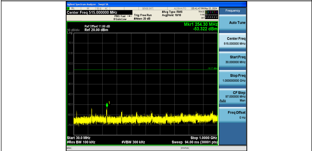
2DH5-Ant1-2441-30~1000-PASS
