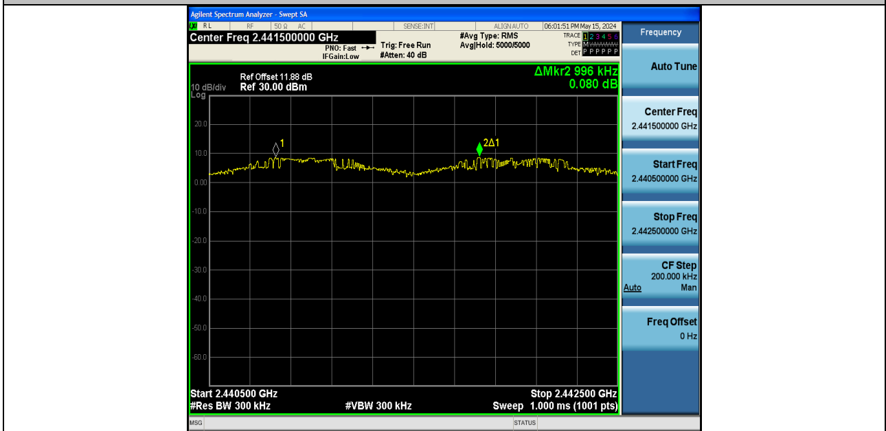
3DH5-Ant1-Hop-PASS
