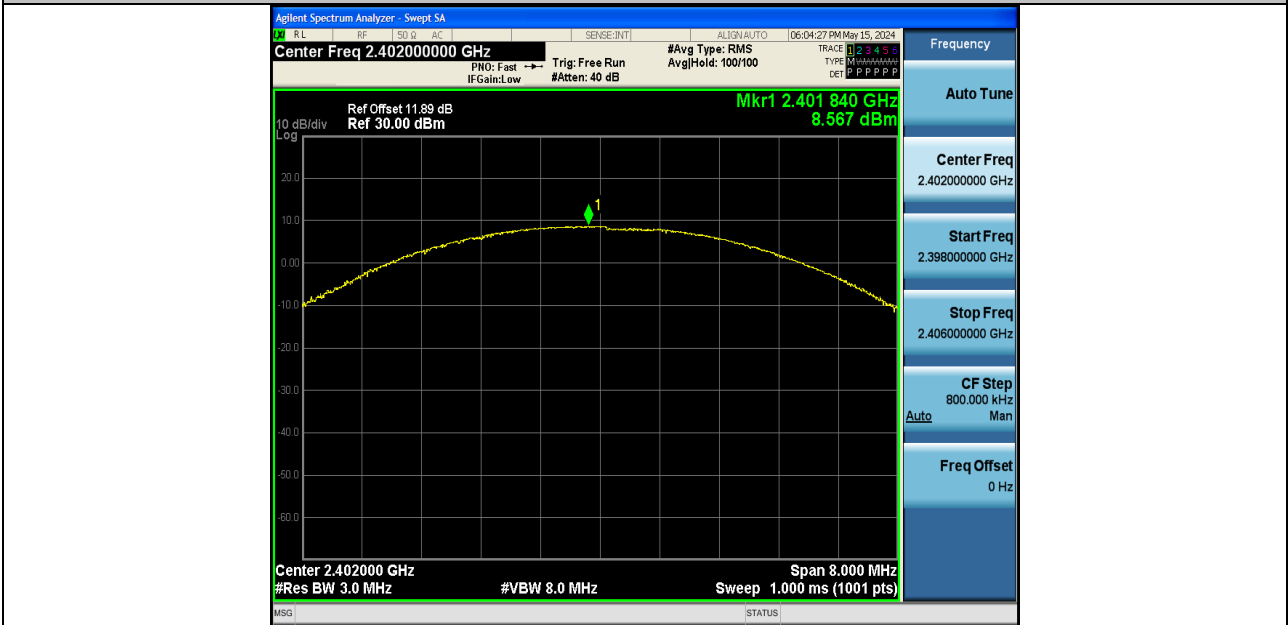
2DH5-Ant1-2402-PASS
