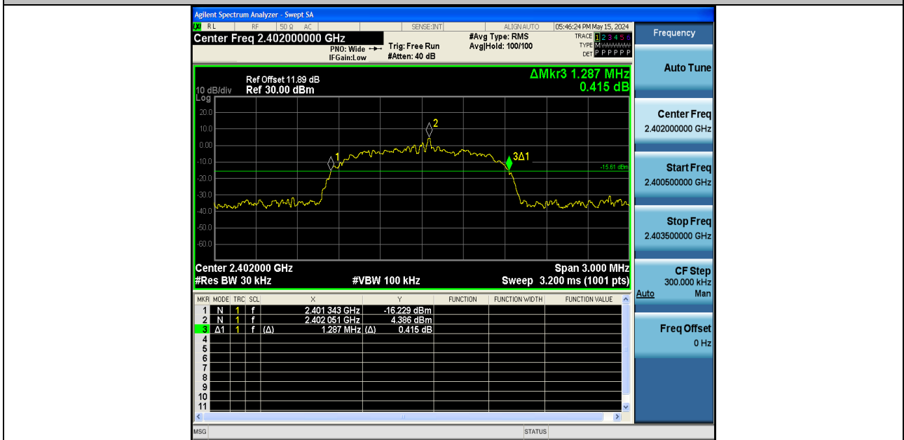
3DH5-Ant1-2402
