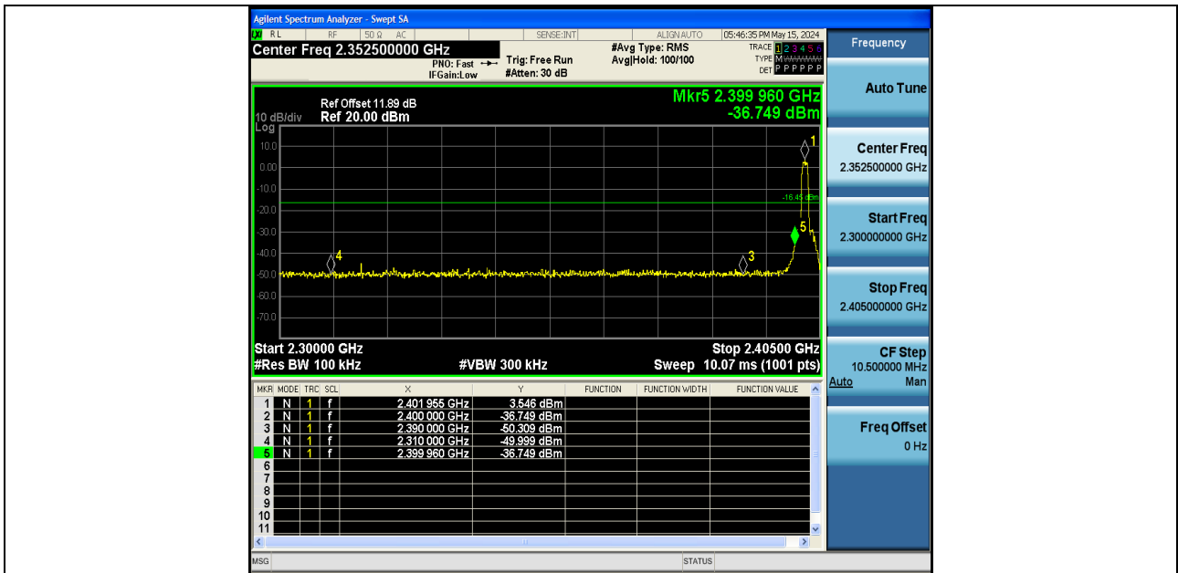
3DH5-Ant1-2402-PASS
