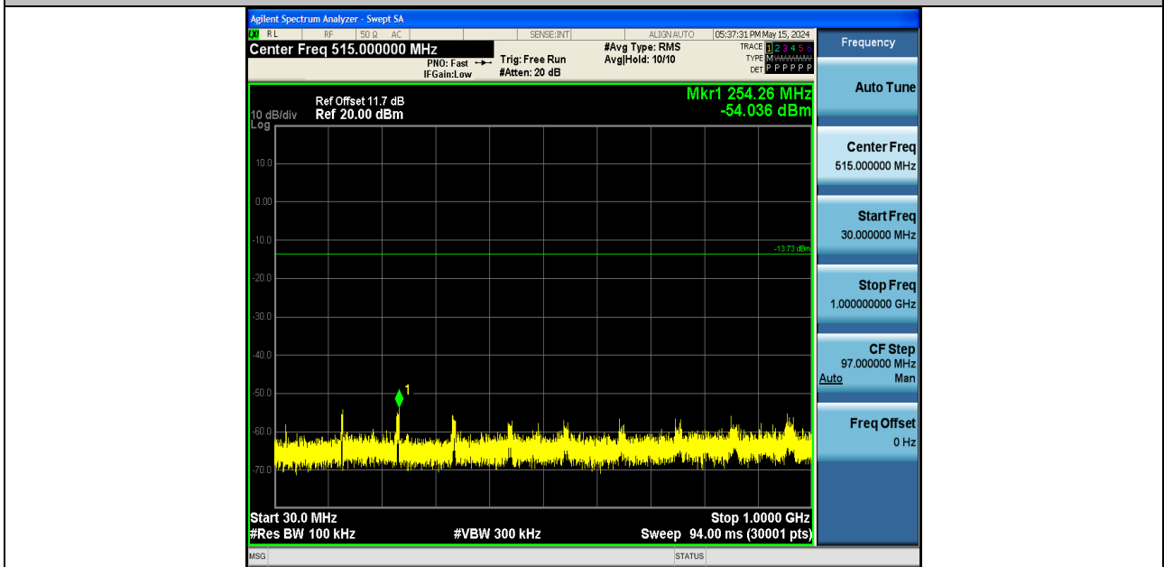
DH5-Ant1-2480-30~1000-PASS
