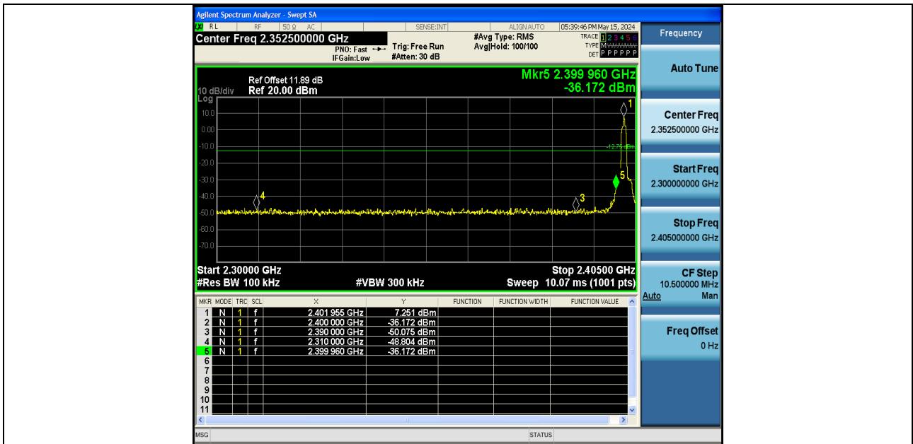
2DH5-Ant1-2402-PASS
