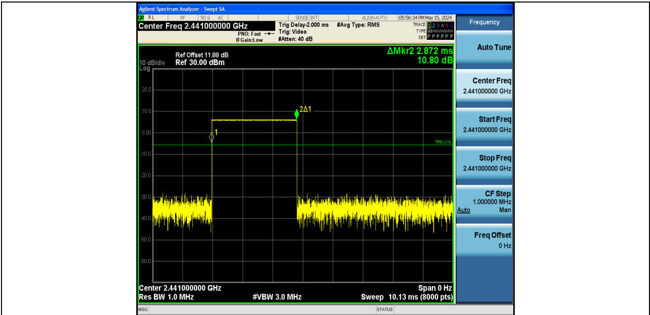
DH5-Ant1-Hop-PASS
