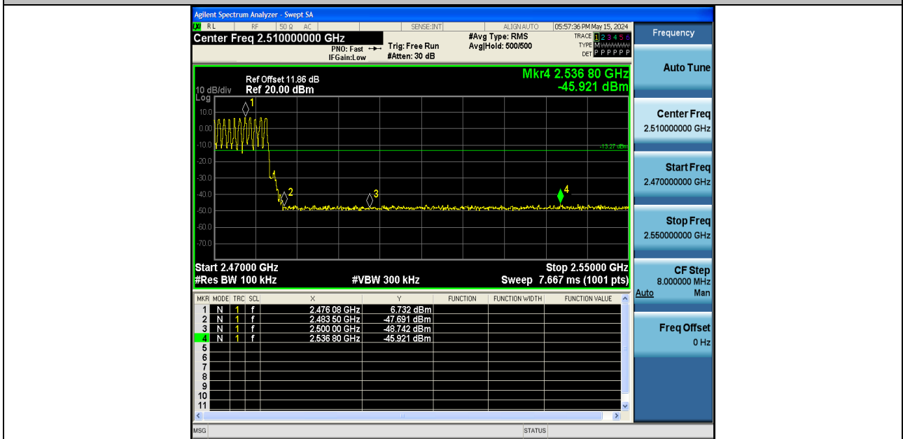
DH5-Ant1-Hop_2480-PASS
