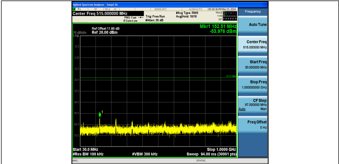
3DH5-Ant1-2441-30~1000-PASS
