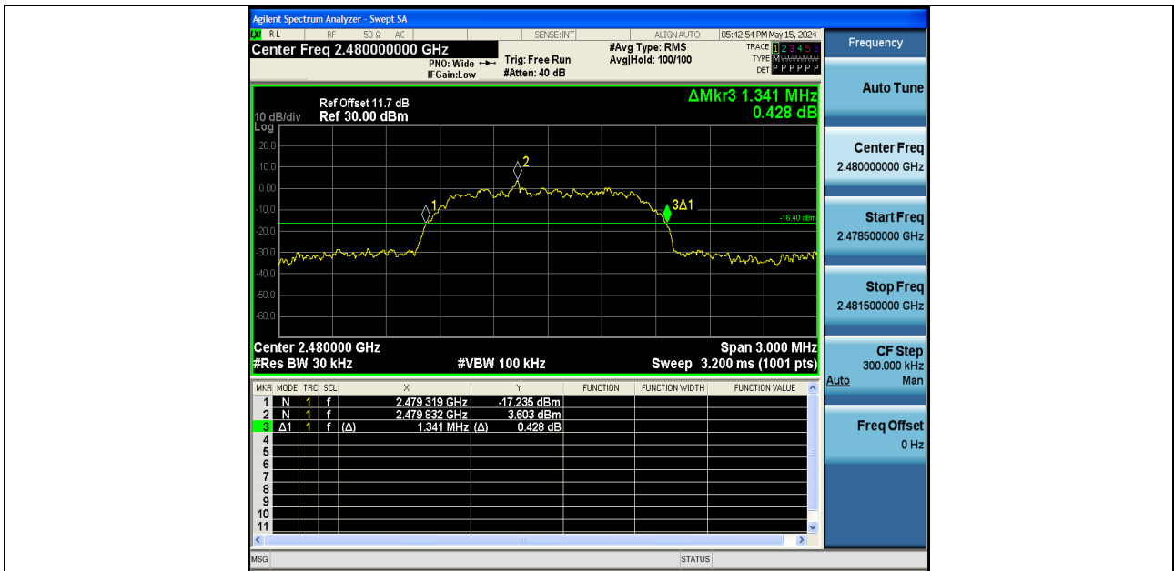
2DH5-Ant1-2480
