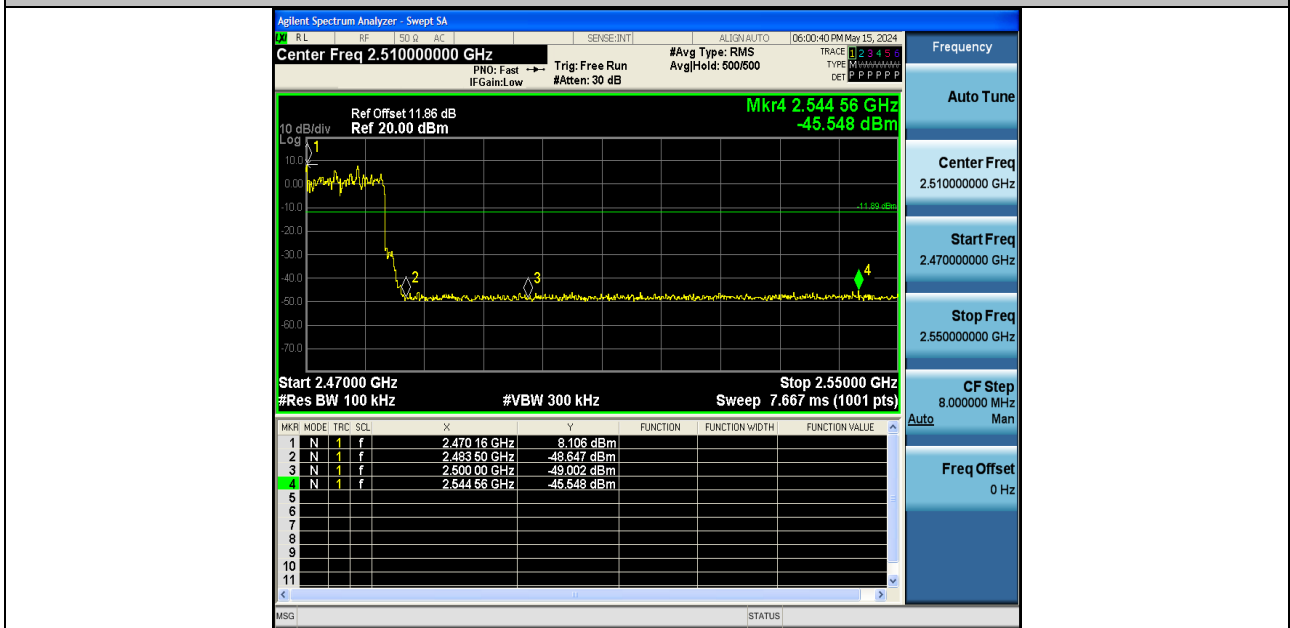
2DH5-Ant1-Hop_2480-PASS
