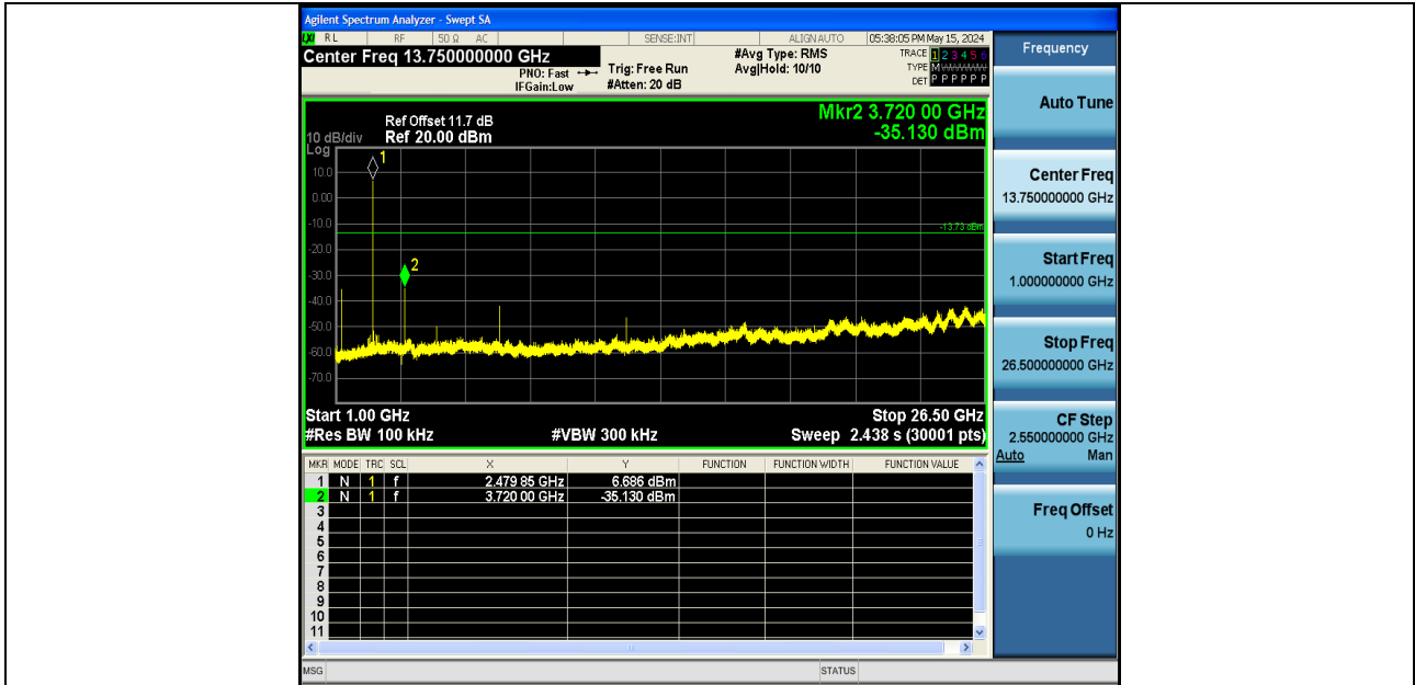
DH5-Ant1-2480-1000~26500-PASS
