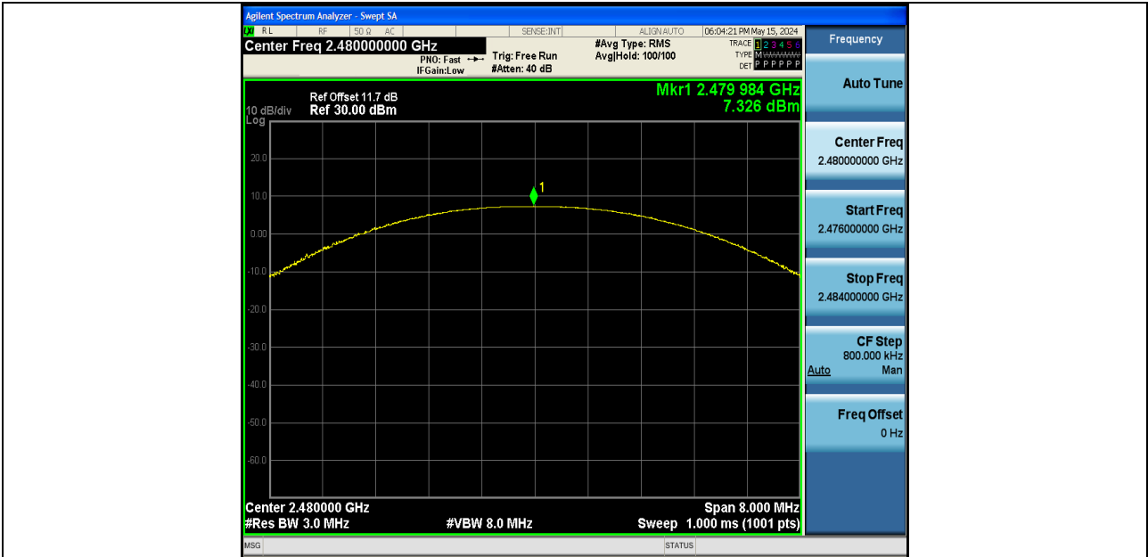
DH5-Ant1-2480-PASS
