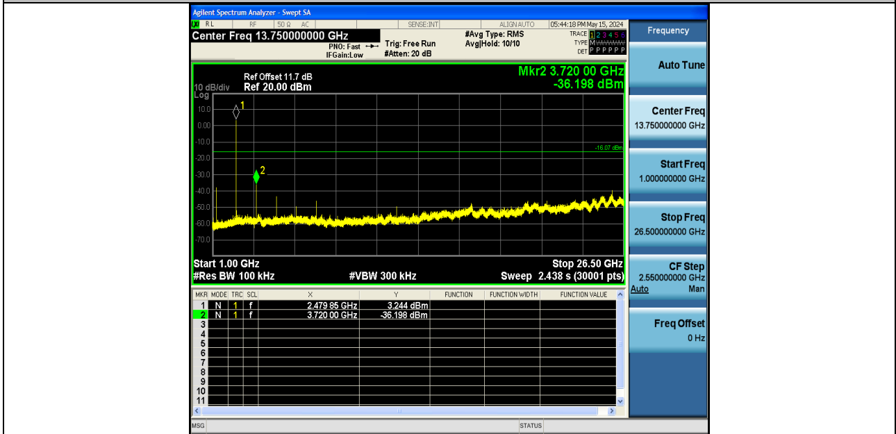
2DH5-Ant1-2480-1000~26500-PASS
