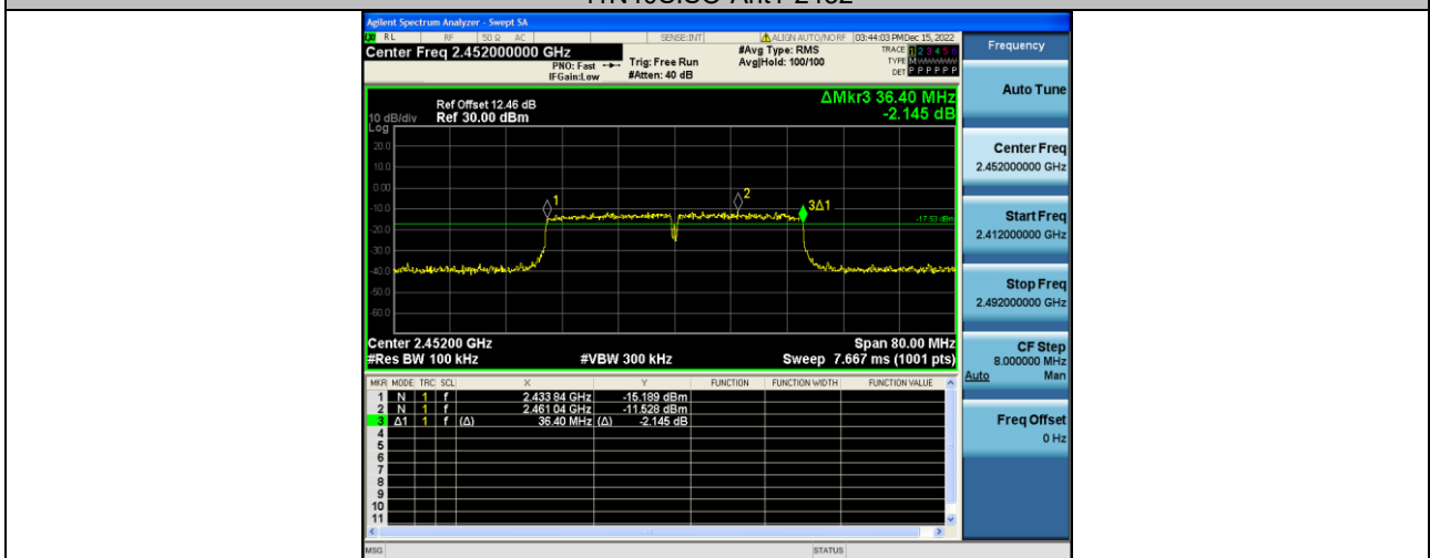
11N40SISO-Ant1-2452
