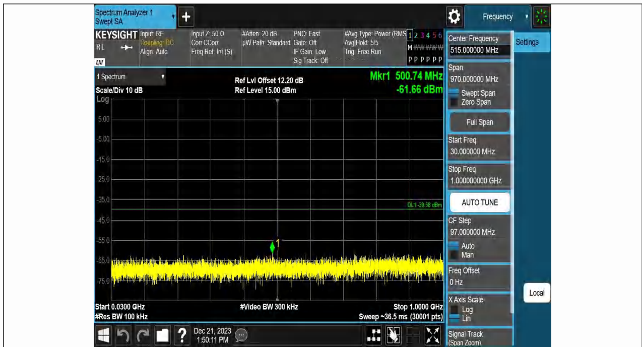
11N20SISO-Ant1-2437-30~1000-PASS
