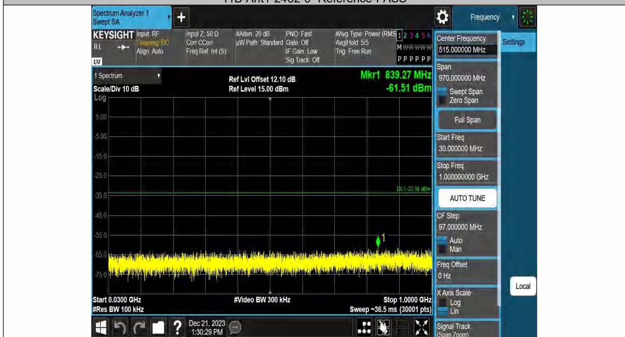
11B-Ant1-2462-30~1000-PASS
