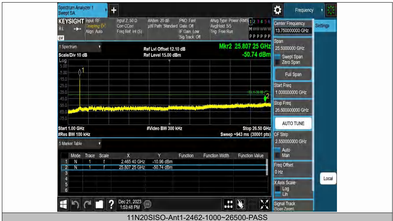
11N20SISO-Ant1-2462-1000~26500-PASS
