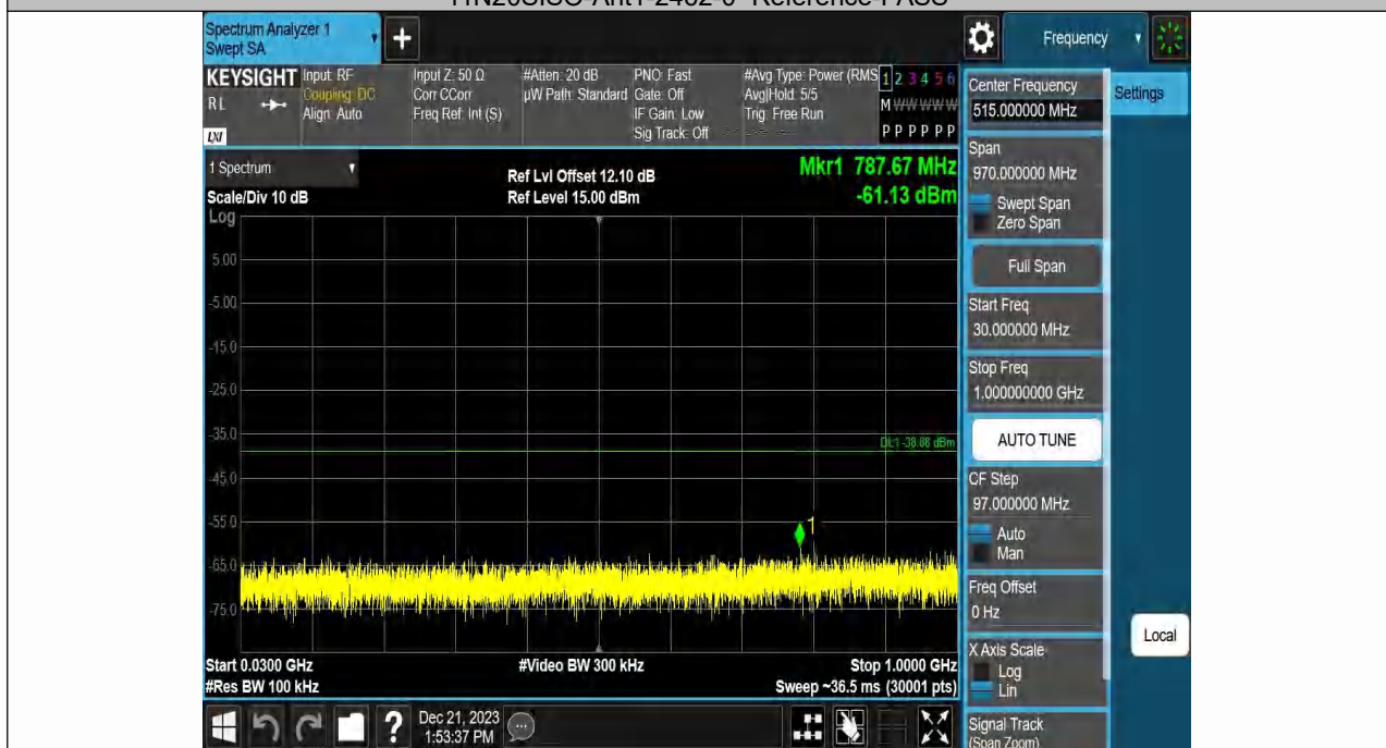
11N20SISO-Ant1-2462-30~1000-PASS
