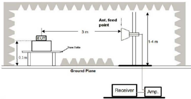
Above 1GHz
