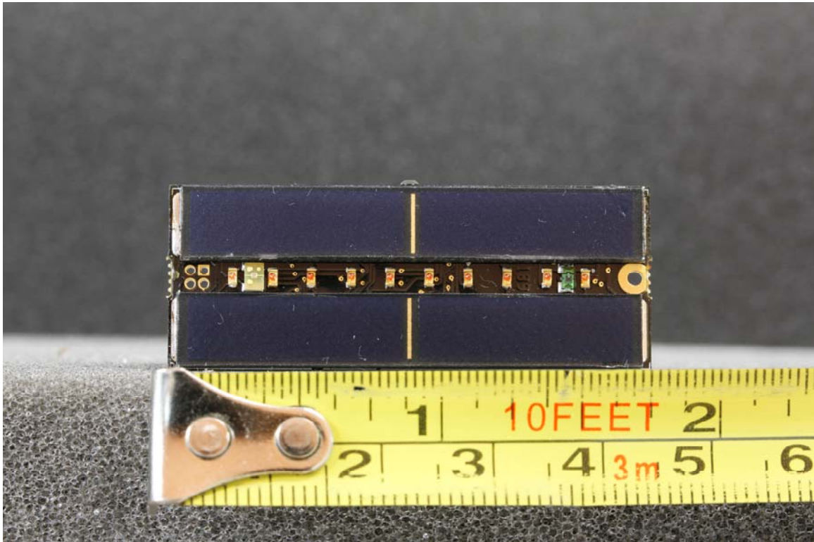
PCB Front with Solar Cells
