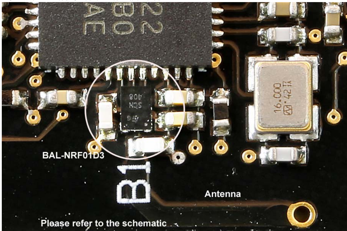
PCB with Printed Circuit Antenna circled
