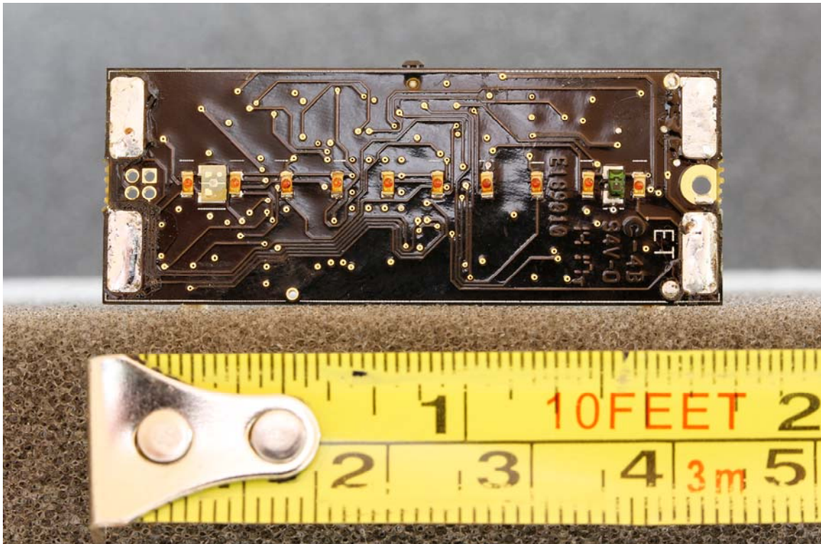
PCB Front without Solar Cells
