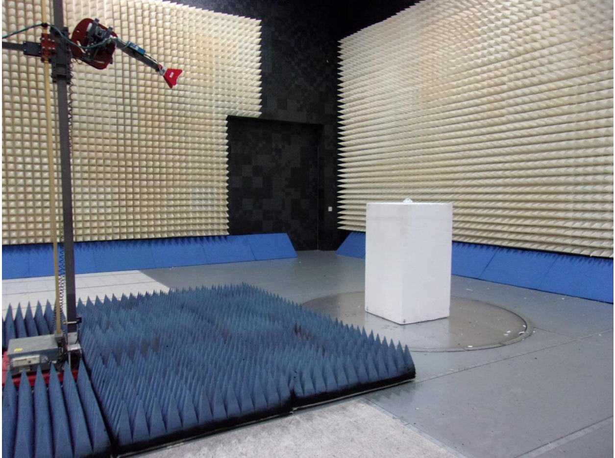
Radiated Emissions Above 1GHz (Transmitter Active)
