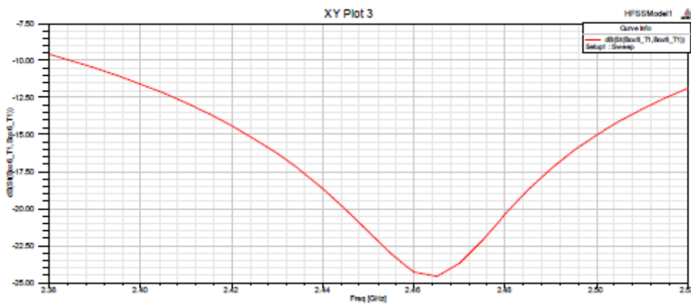
Figure 8. Antenna port S11 simulation curve
