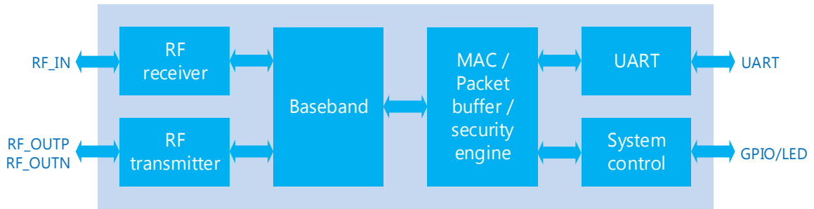
Figure 1. WT1FBS block diagram
