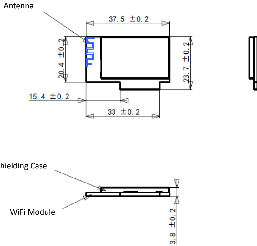
Figure3.WT1FBSview(Metricunits)
