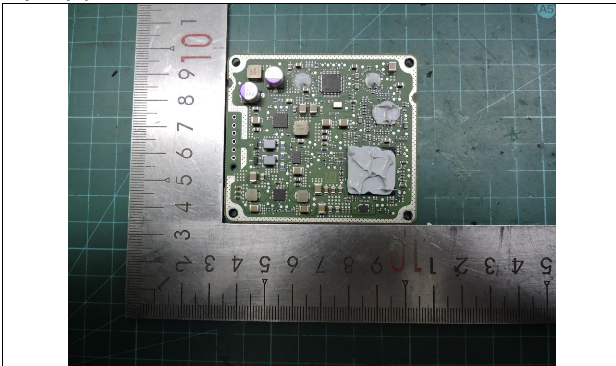
PCB Front
