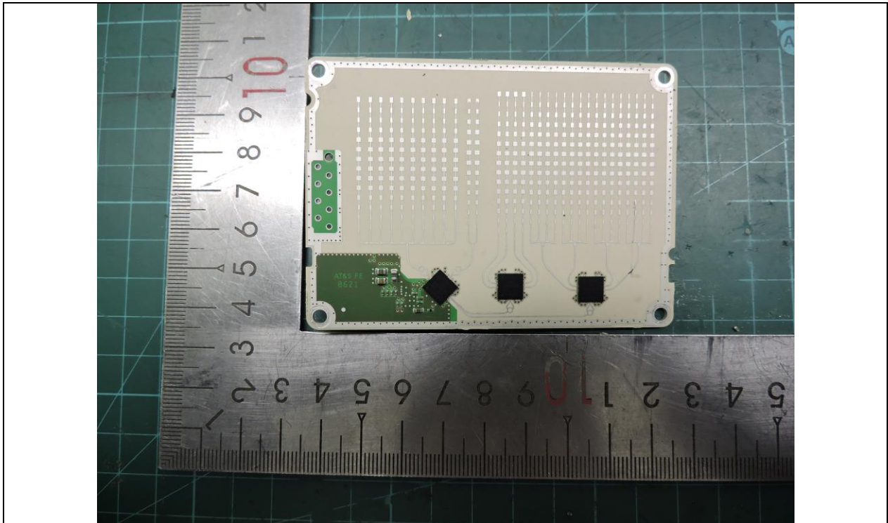
PCB Rear
