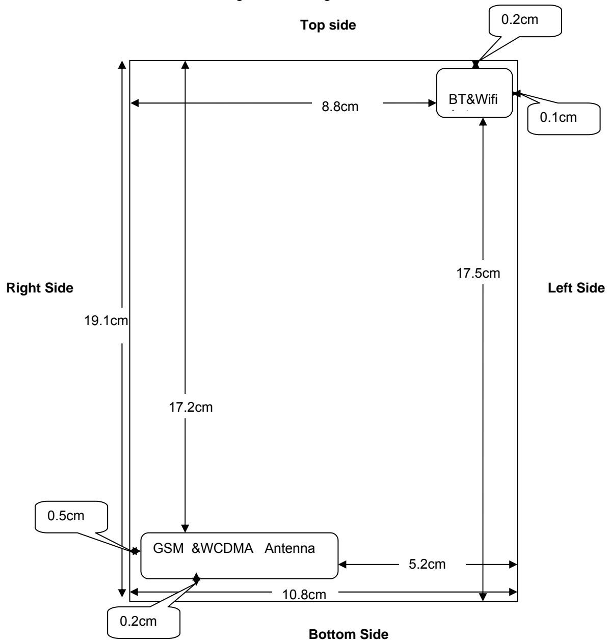
Figure 1: The diagonal dimension of the DUT
