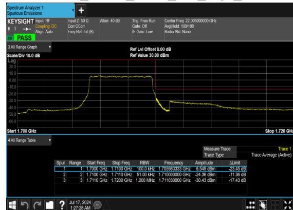
N70(5M)_DFT-s- OFDM_QPSK_Outer_Full_High_CH
