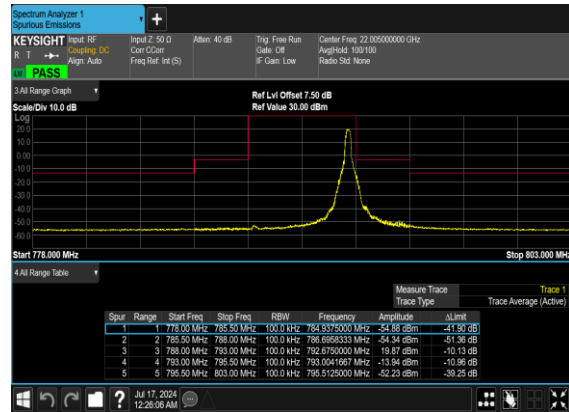
N14(5M)_DFT-s- OFDM_QPSK_Edge_1RB_Right_Low_CH
