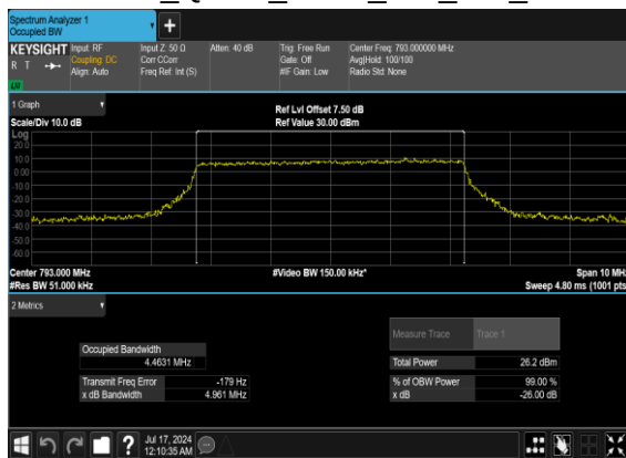
N14(5M)_CP- OFDM_QPSK_Outer_Full_Mid_CH
