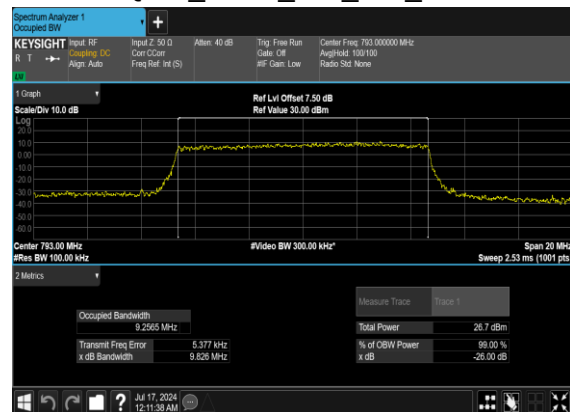
N14(10M)_CP-OFDM_16 QAM_Outer_Full_Mid_CH
