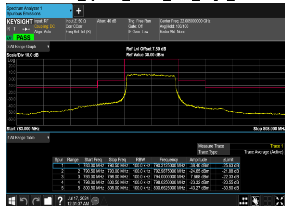
N14(5M)_DFT-s- OFDM_QPSK_Outer_Full_High_CH
