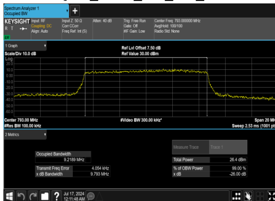
N14(10M)_CP-OFDM_64 QAM_Outer_Full_Mid_CH
