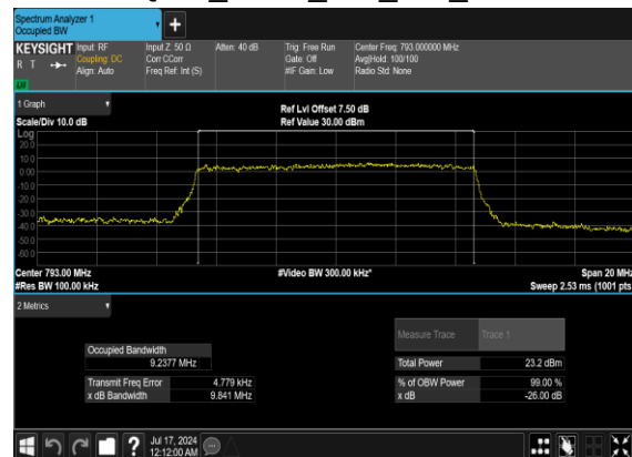
N14(10M)_CP-OFDM_256 QAM_Outer_Full_Mid_CH
