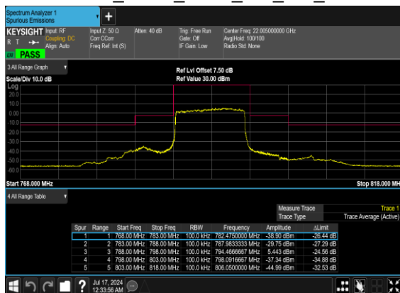
N14(10M)_DFT-s- OFDM_BPSK_Outer_Full_Mid_CH
