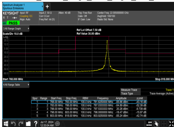
N14(10M)_DFT-s- OFDM_BPSK_Edge_1RB_Right_Mid_CH
