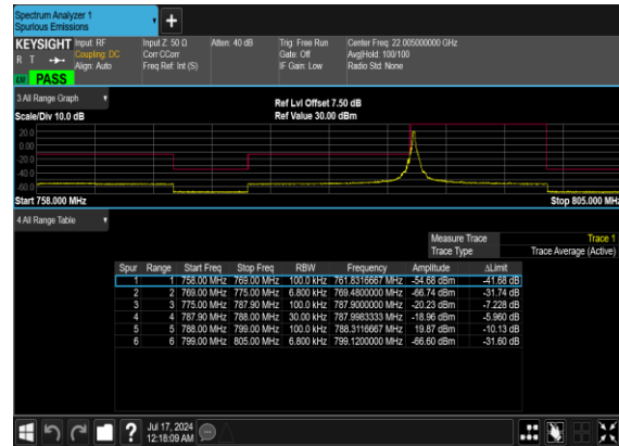
N14(5M)_DFT-s- OFDM_QPSK_Edge_1RB_Left_Low_CH
