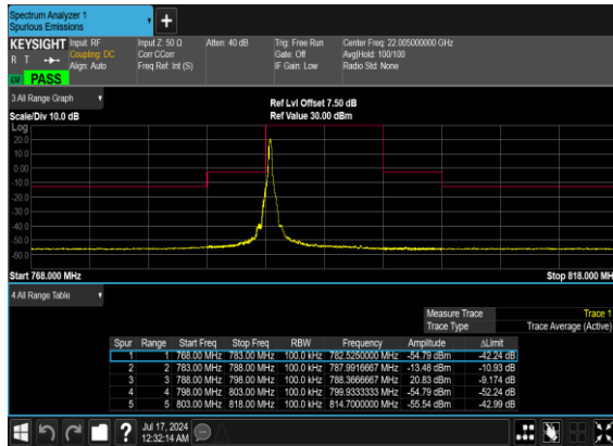
N14(10M)_DFT-s- OFDM_BPSK_Edge_1RB_Left_Mid_CH
