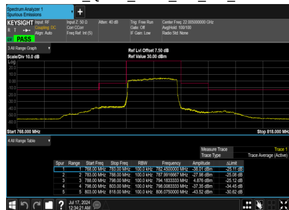
N14(10M)_DFT-s- OFDM_QPSK_Outer_Full_Mid_CH
