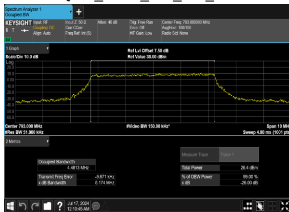
N14(5M)_CP-OFDM_16 QAM_Outer_Full_Mid_CH
