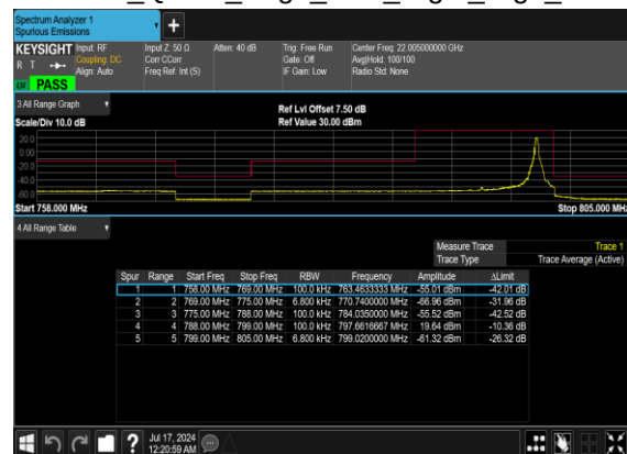
N14(5M)_DFT-s- OFDM_QPSK_Edge_1RB_Right_High_CH
