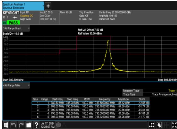
N14(5M)_DFT-s-OFDM_BPSK_Edge_1RB_Right_Mid_CH
