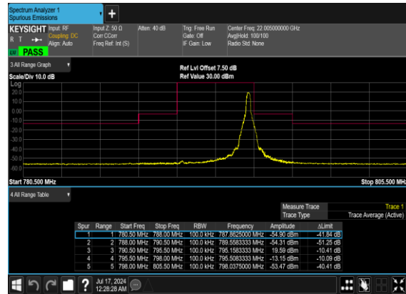
N14(5M)_DFT-s-OFDM_QPSK_Edge_1RB_Right_Mid_CH
