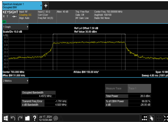
N14(5M)_CP-OFDM_64 QAM_Outer_Full_Mid_CH
