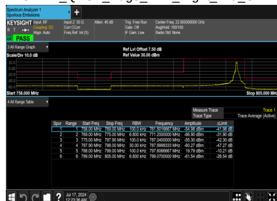
N14(10M)_DFT-s- OFDM_QPSK_Edge_1RB_Right_Mid_CH
