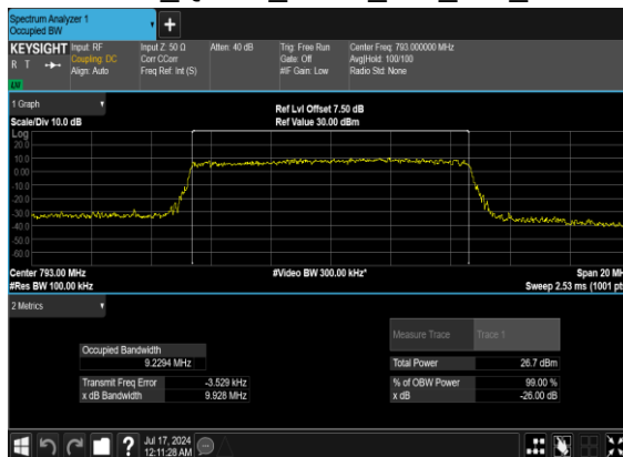
N14(10M)_CP- OFDM_QPSK_Outer_Full_Mid_CH
