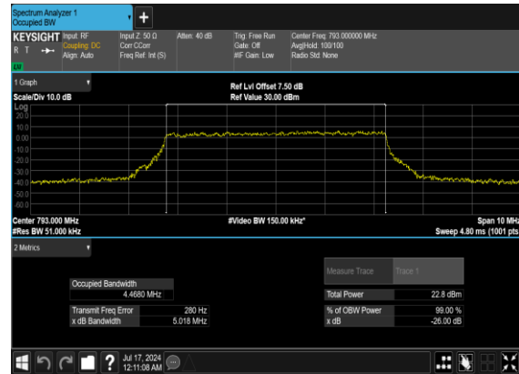
N14(5M)_CP-OFDM_256 QAM_Outer_Full_Mid_CH
