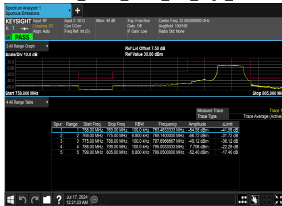
N14(5M)_DFT-s- OFDM_BPSK_Outer_Full_High_CH
