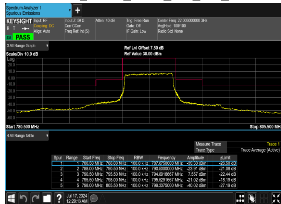
N14(5M)_DFT-s-OFDM_QPSK_Outer_Full_Mid_CH
