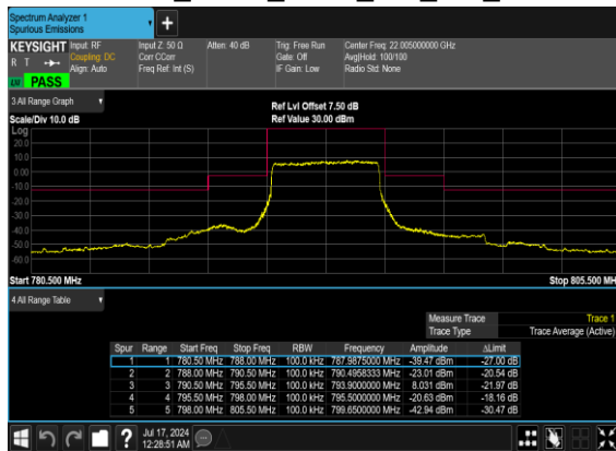
N14(5M)_DFT-s-OFDM_BPSK_Outer_Full_Mid_CH
