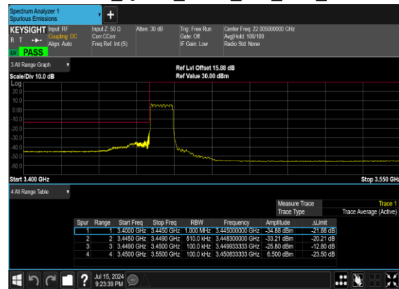
N77(10M)_DFT-s- OFDM_QPSK_Outer_Full_Low_CH
