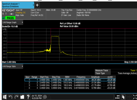
N77(10M)_DFT-s- OFDM_BPSK_Outer_Full_Low_CH
