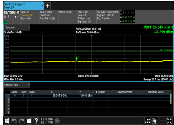
N77(100M)_DFT-s- OFDM_QPSK_Edge_1RB_Left_Mid_CH
