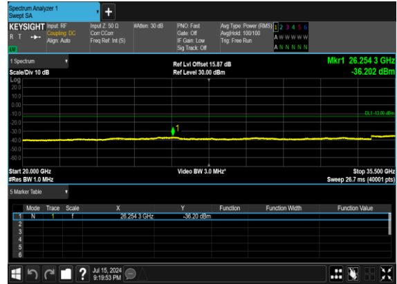
N77(100M)_DFT-s- OFDM_BPSK_Edge_1RB_Left_Mid_CH
