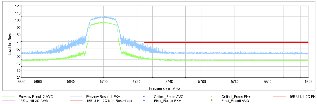
Fig.37 Band Edges (802.11a Ch140, 5700MHz)
