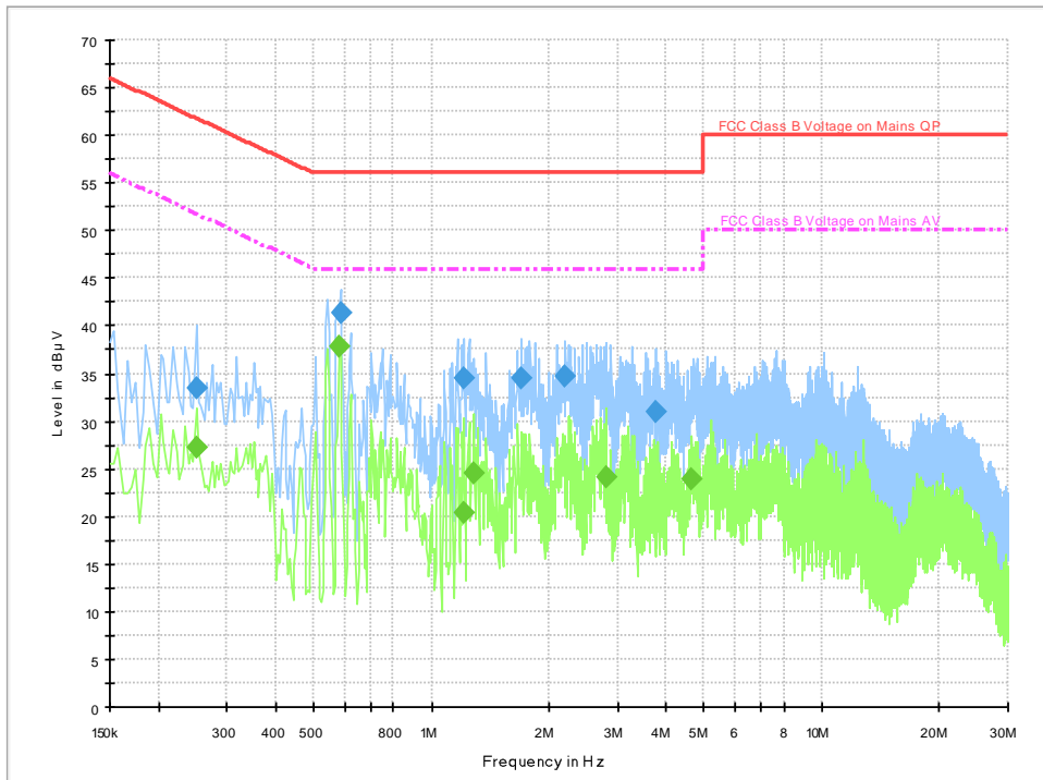
Fig.B.9.1 AC Powerline Conducted Emission- bluetooth
