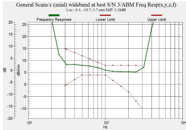
Figure C.1 Frequency Response of WCDMA 850
