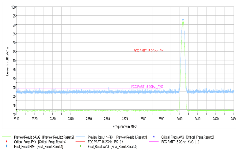
Fig.3. Frequency Band Edges: GFSK, 2402 MHz, Hopping Off, 2.31 GHz – 2.43GHz
