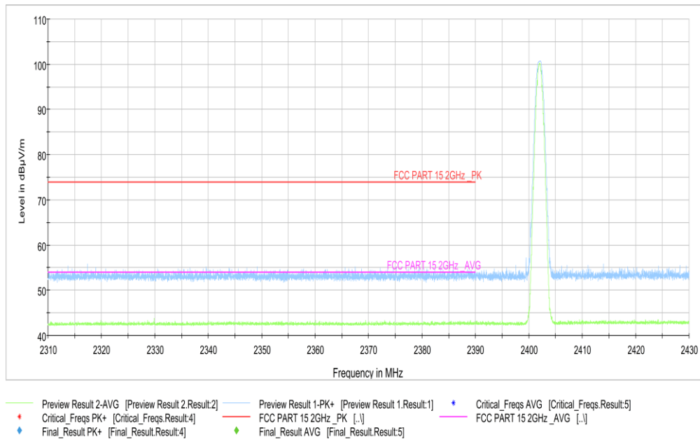
Fig.13. Frequency Band Edges: GFSK, Channel 0, Hopping Off, 2.31 GHz – 2.43GHz
