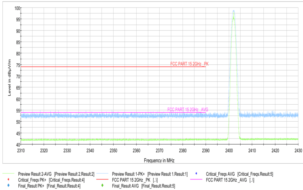
Fig.17. Frequency Band Edges: 8DPSK, Channel 0, 2.31 GHz - 2.43GHz
