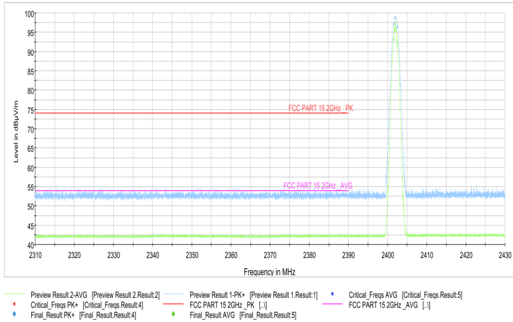
Fig.15. Frequency Band Edges: \pi/4 DQPSK, Channel 0, Hopping Off, 2.31 GHz - 2.43GHz
