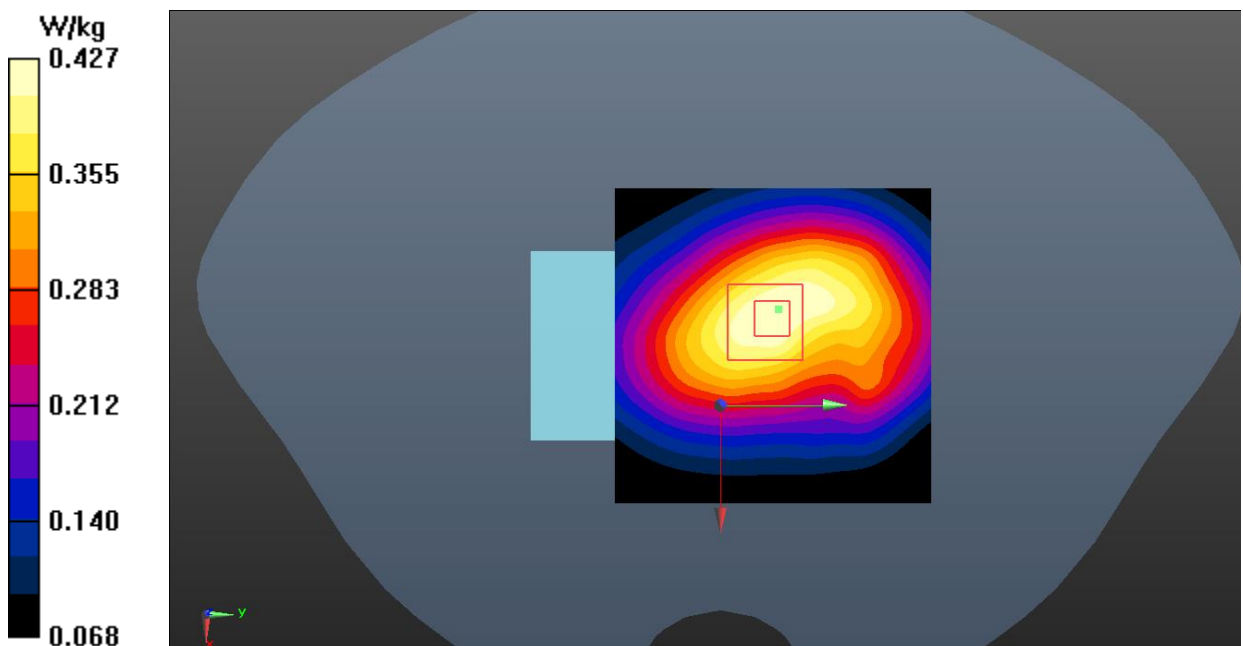
Fig.29 LTE Band 71 Hotspot
