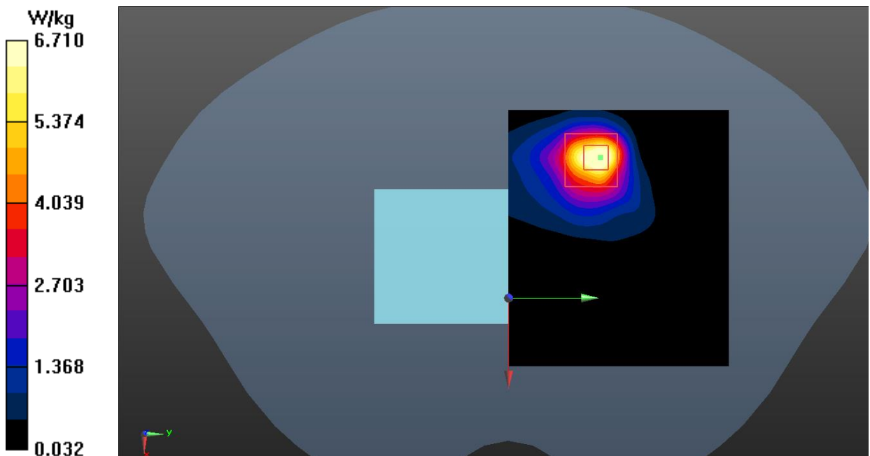
Fig.38 WCDMA Band 4 Body
