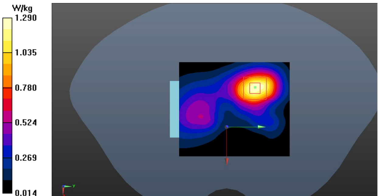
Fig.17 LTE Band 7 Hotspot
