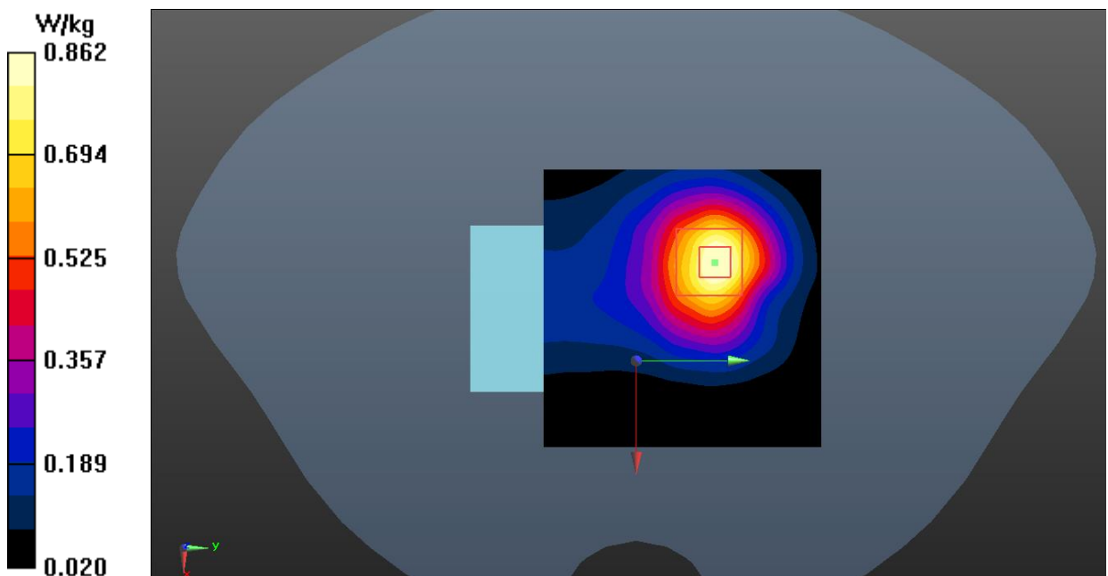
Fig.27 LTE Band 66 Body-Worn
