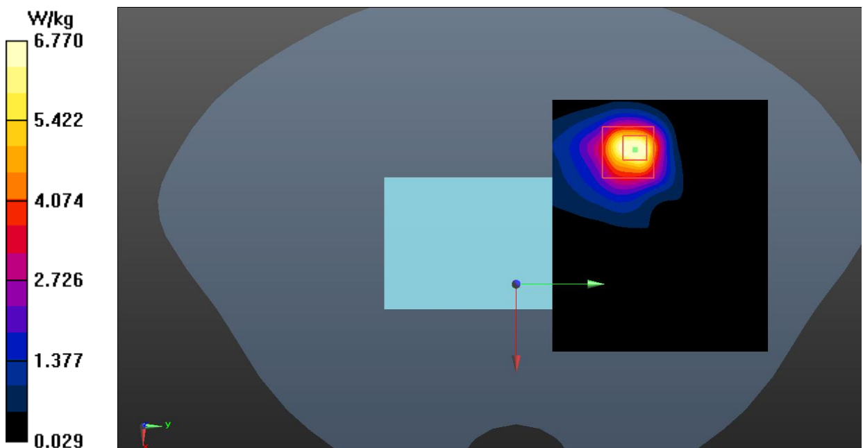
Fig.41 LTE Band 66 Body
