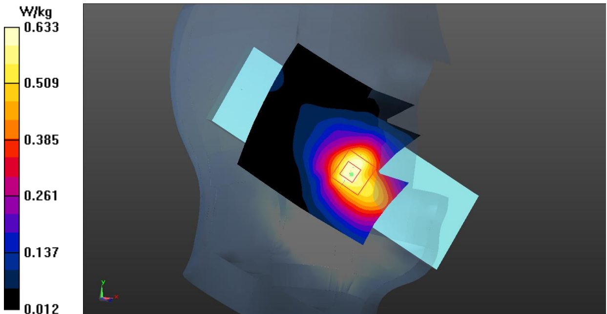
Fig.16 LTE Band 7 Head
