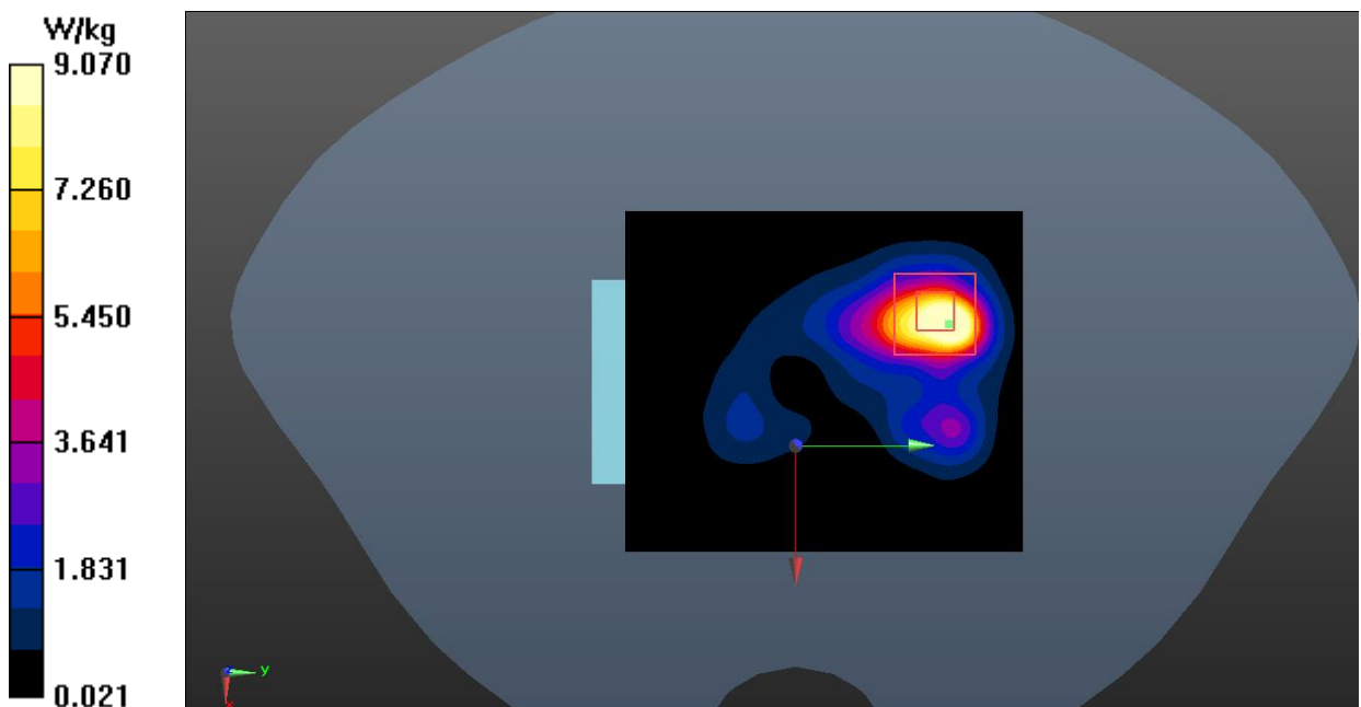
Fig.40 LTE Band 7 Body
