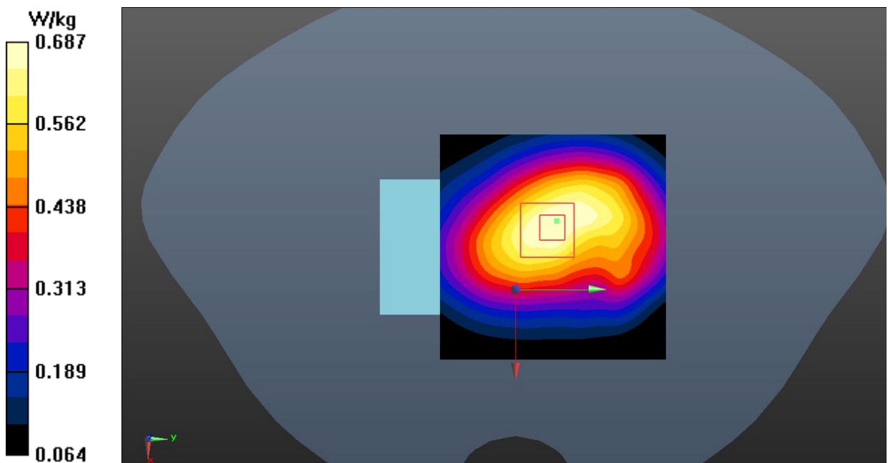
Fig.21 LTE Band 12 Body-Worn
