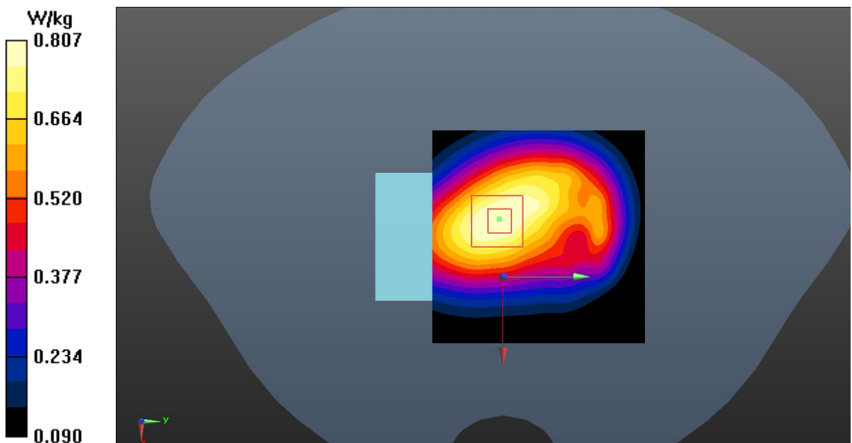
Fig.14 LTE Band 5 Hotspot
