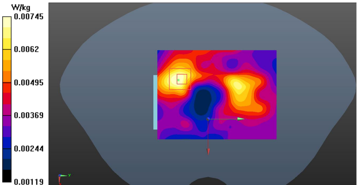
Fig.33 Bluetooth Body-Worn
