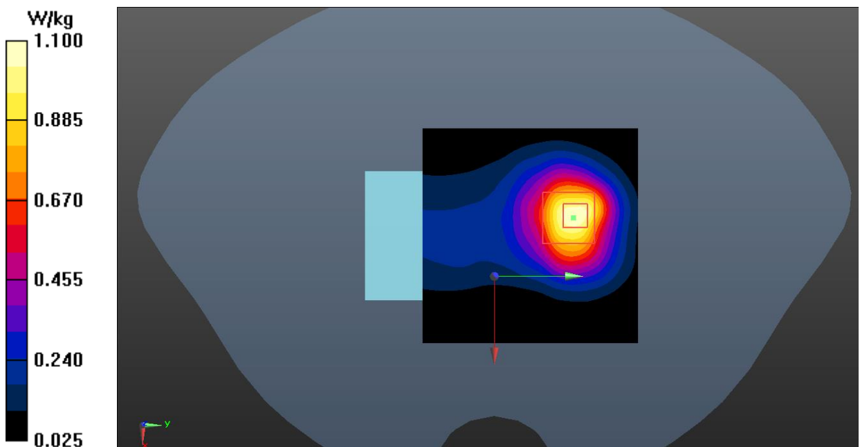
Fig.26 LTE Band 66 Hotspot
