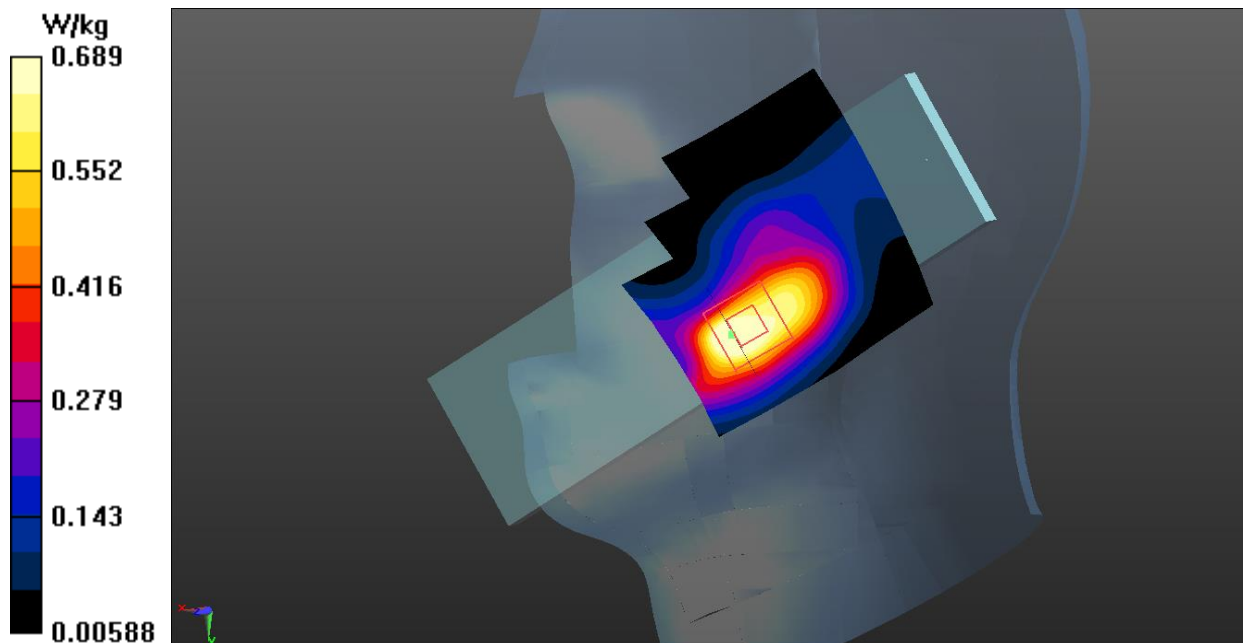
Fig.34 WLAN 2.4G Head
