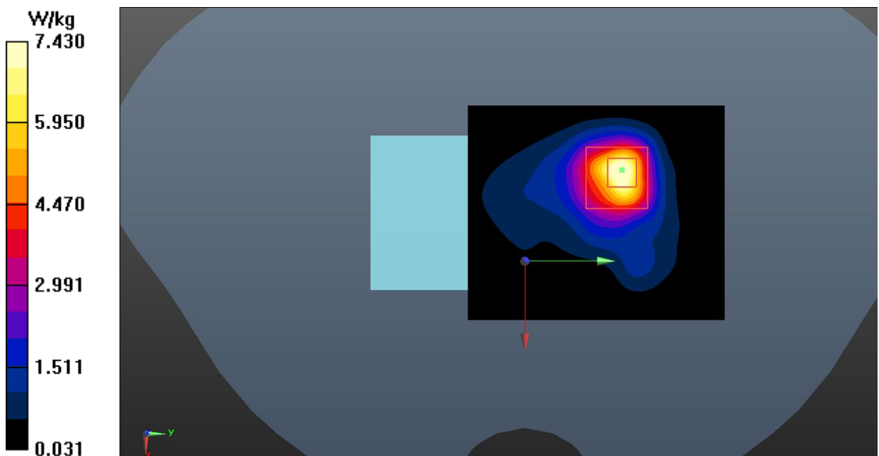
Fig.39 LTE Band 2 Body
