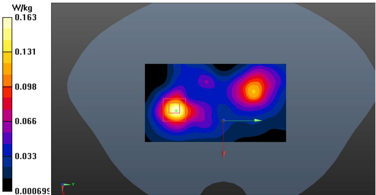
Fig.35 WLAN 2.4G Hotspot
