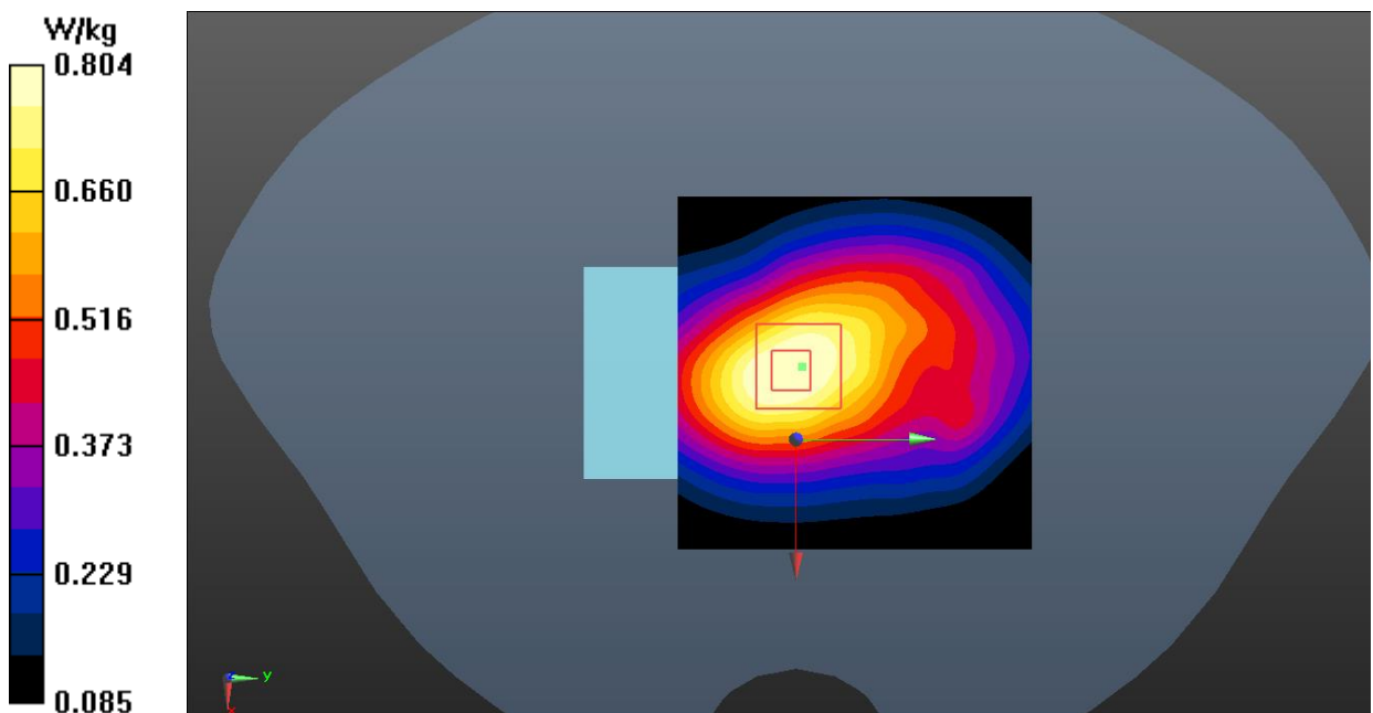
Fig.23 LTE Band 13 Hotspot
