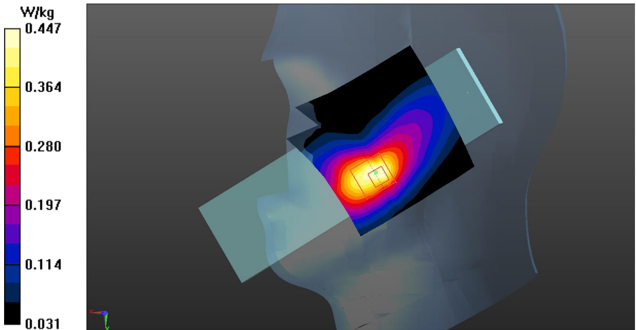
Fig.28 LTE Band 71 Head
