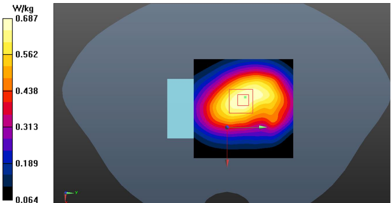
Fig.20 LTE Band 12 Hotspot
