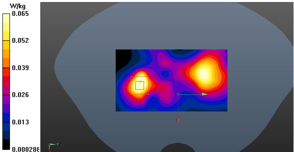
Fig.36 WLAN 2.4G Body-Worn
