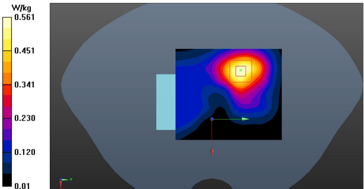
Fig.18 LTE Band 7 Body-Worn
