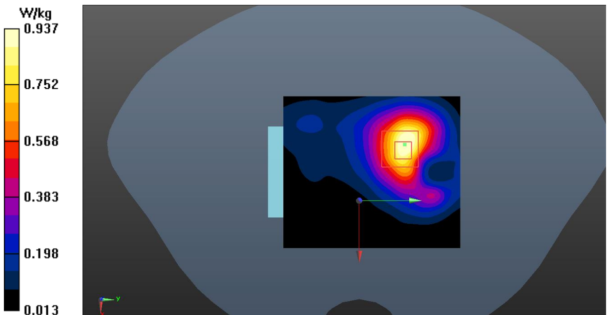
Fig.11 LTE Band 2 Hotspot
