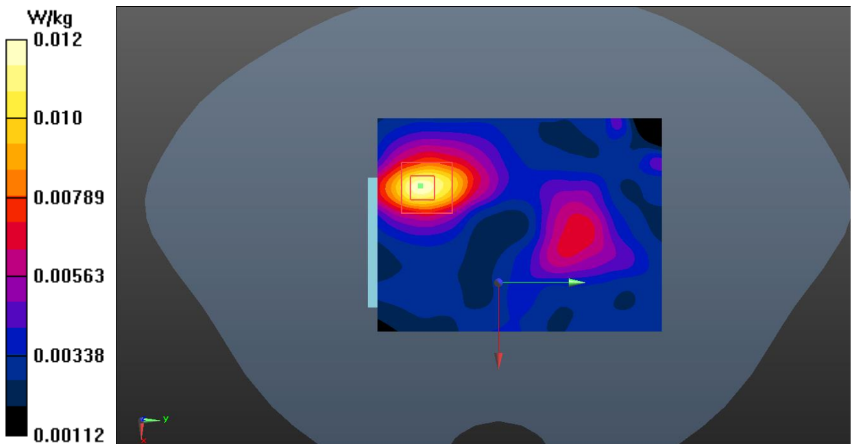
Fig.32 Bluetooth Hotspot
