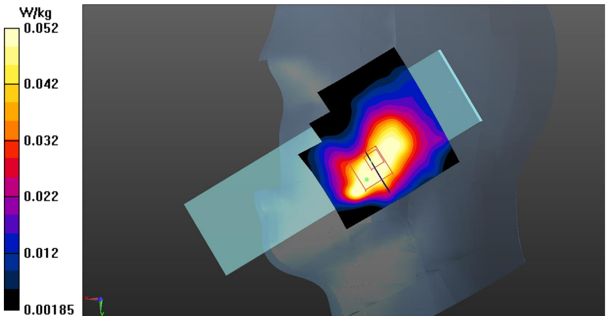
Fig.31 Bluetooth Head
