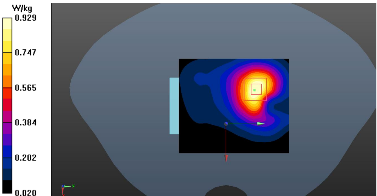
Fig.12 LTE Band 2 Body-Worn
