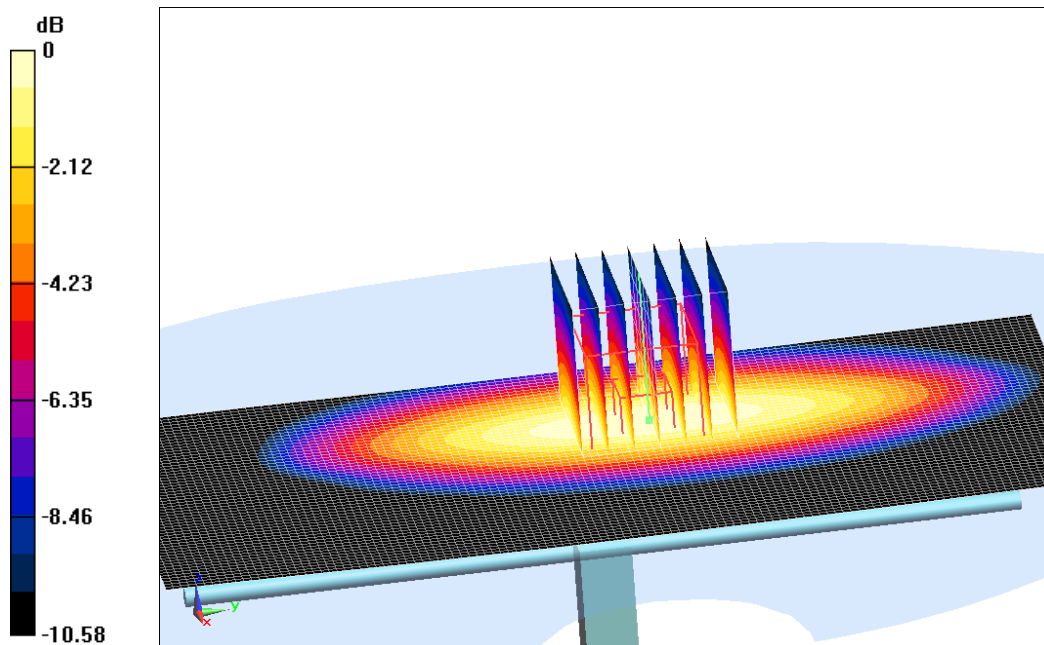
Fig.I.5-1 validation 835 MHz 250mW
