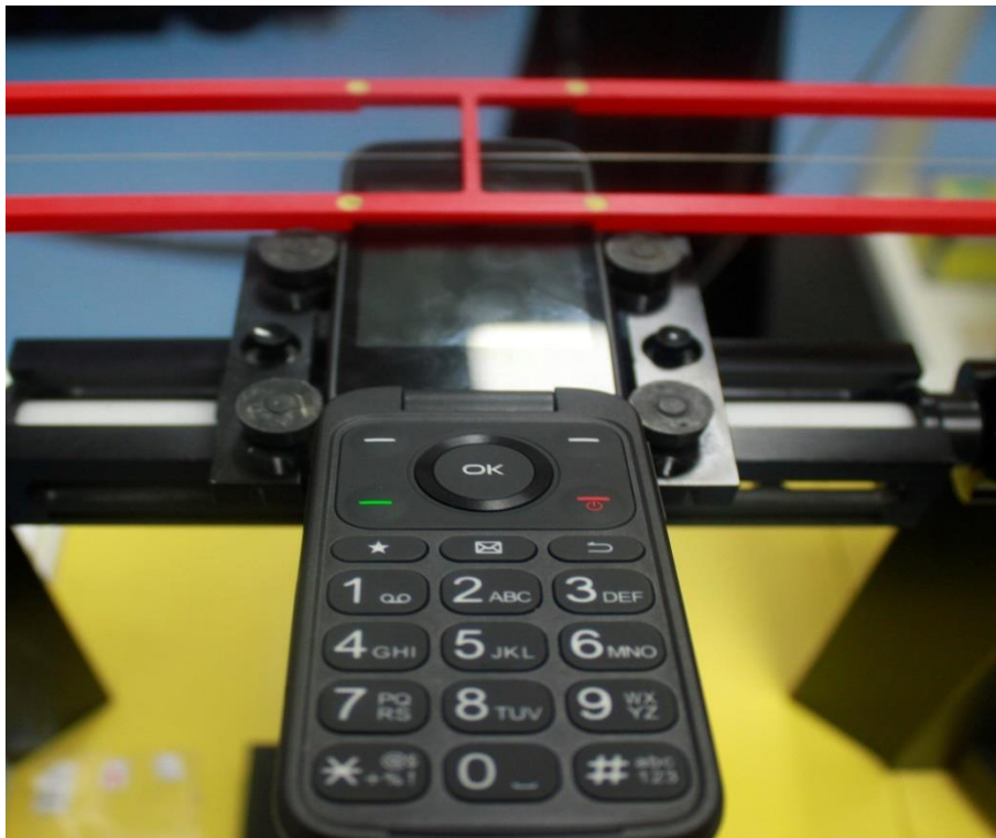
Picture 2: EUT Positioning for RF/T-coil
