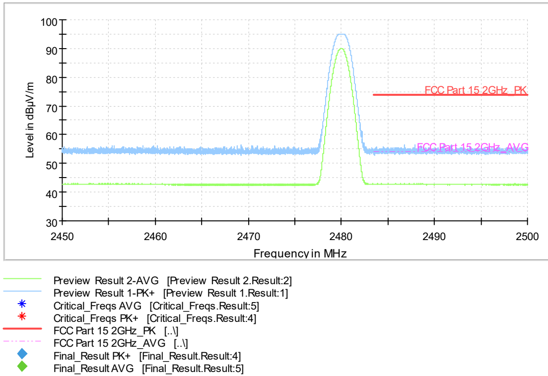
Fig.4. Frequency Band Edges: BLE GFSK, 2480 MHz, Hopping Off , 2.45 GHz - 2.50GHz
