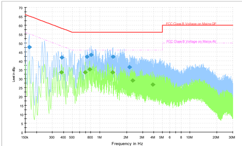
Fig.B.9.1 AC Powerline Conducted Emission- Bluetooth BLE
