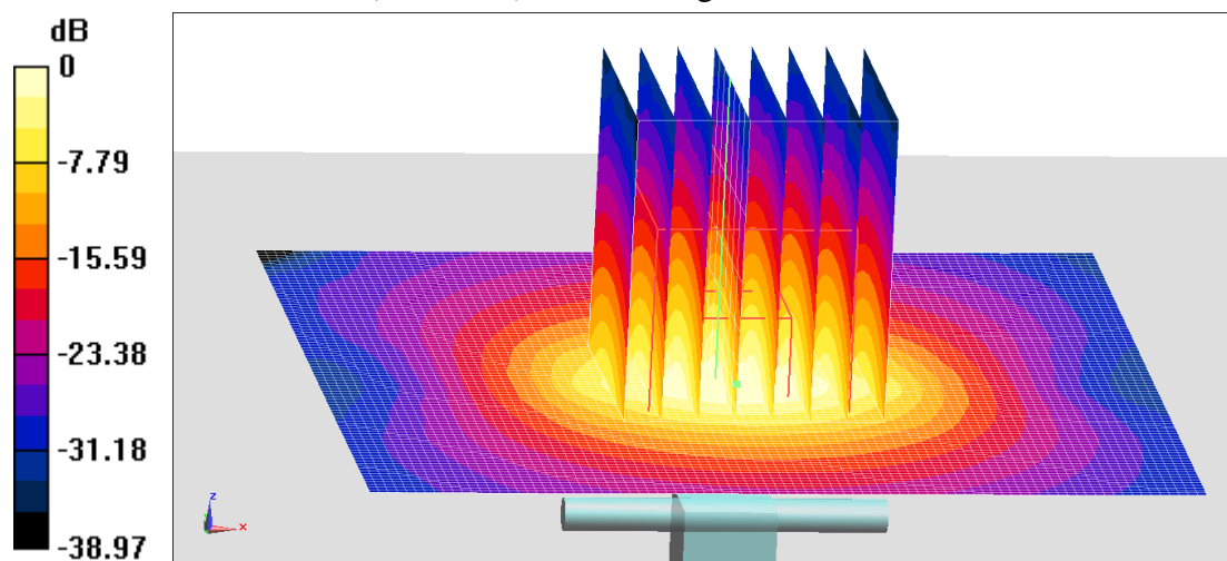
Fig.B.13 validation 3800 MHz 100mW
