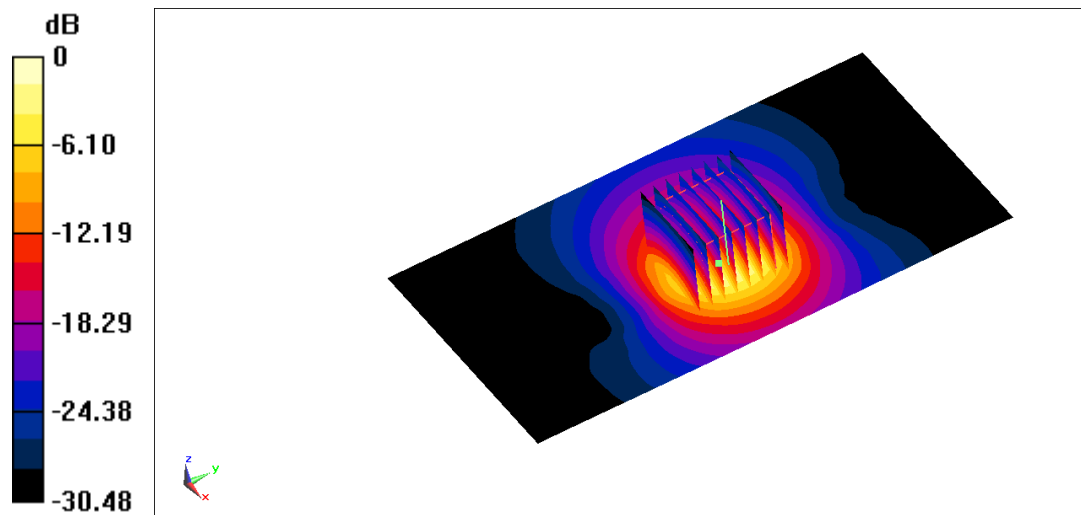
Fig.B.12 validation 3500 MHz 100mW
